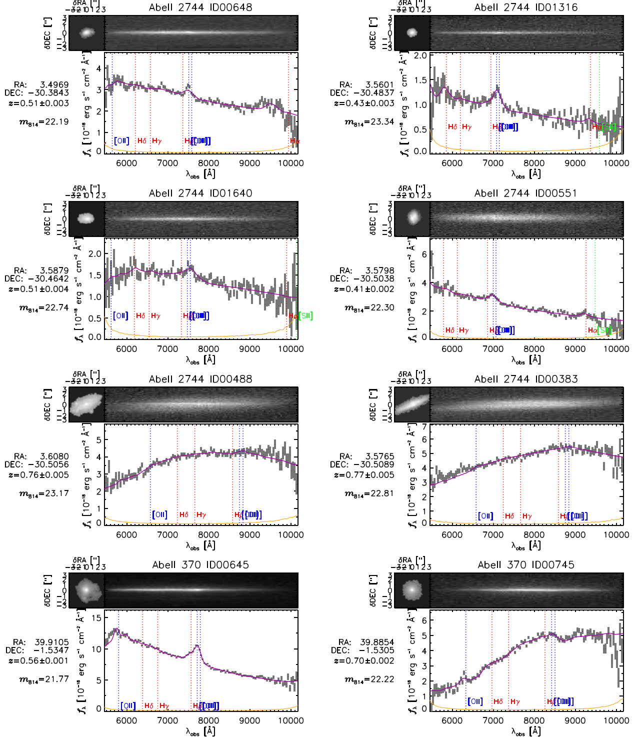
Figure D1. Examples of the \sim 300 bright, S/N \geq 5 [\text{O III}] emitters in the glass data base.
