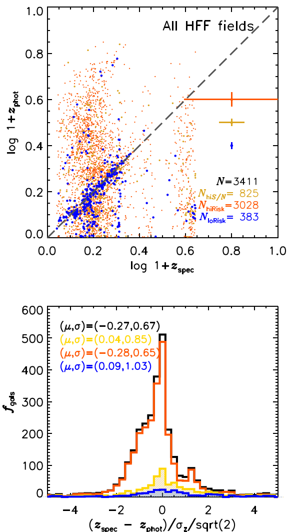
Figure C1. Similar to Fig. 4 but plotting HFF photometric redshifts from Shipley et al. (2018) ( z_{\text{phot}} ) against GLASS G800L redshifts ( z_{\text{spec}} ). Distributions are much wider, but agreement is still fair, with low risk sources having photo- z errors consistent with Gaussian noise. All samples show slight biases, but those for high- S/N + lines and low-risk sources are small in the mean.
