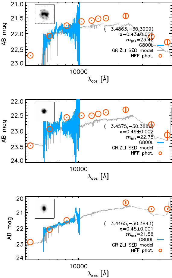
Figure 12. Examples of GLASS G800L spectra (blue) and GRIZLI inferred continuum SEDs (grey) shown with matched source photometry from the HFF campaign (Shipley et al. 2018, orange circles). Some inferences agree remarkably well with photometry lying well outside the grism bandpass despite its limited coverage; others are less consistent. Such offsets – typically at the \sim 0.25 mag level (Section 4.2) – will affect stellar mass and SFR estimates. However, the consistent location of observed and inferred features (e.g. the 1.6\ \mu\text{m} bump) support the accuracy of these sources’ grism-determined redshifts (see also Fig. C1). These data are available to anyone wishing to perform joint spectrophotometric SED fitting on the 13 fields where HST photometry exist (Table 1). More examples of low risk objects in the HFF footprints are shown in Appendix D.
