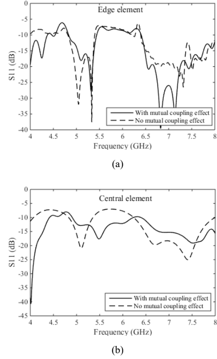
Fig. 5. Comparison of S_{11} with and without coupling effect (a) edge element, (b) central element.
