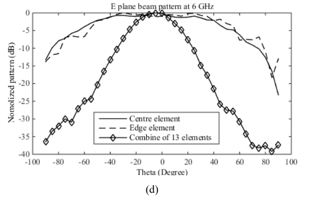
Fig. 7. Effect of Plexiglas dome applied on farfield pattern for one beam shown with 45 degree phi plane cut at (a) 4 GHz, (b) 6 GHz, and (c) 8 GHz (d) comparison of measured beam pattern by centre element, edge element and one combined beam.
