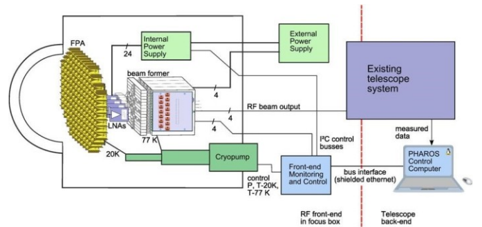
Fig. 3. Schematic of PHAROS.
