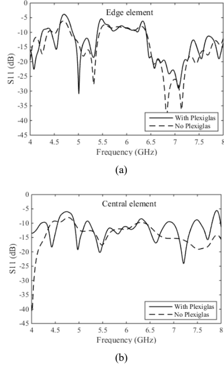
Fig. 6. Comparison of S_{11} with and without Plexiglas effect (a) edge element, (b) central element.
