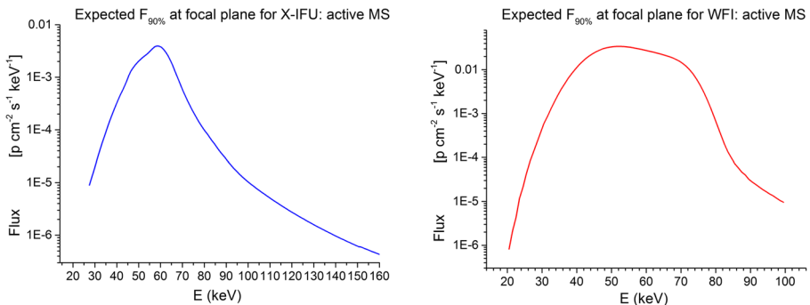
Fig. 10 Spectra of initial energies of the protons that reach the focal plane with 2 < E_{FPA} < 10 keV for the worst case of active magnetosheath (90% of time) for X-IFU (left) and WFI (right)
