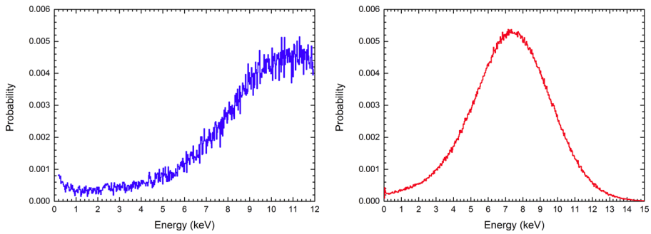
Fig. 6 Row of the redistribution matrix relative to the input proton energy of 60 keV for the X-IFU (left, blue) and the WFI (right, red)
