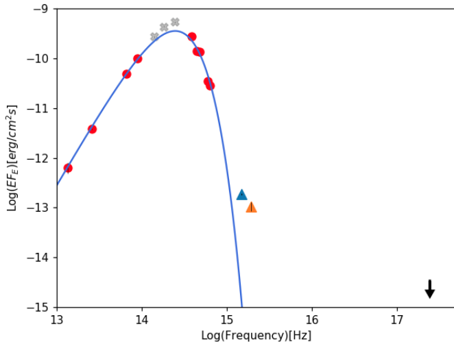
Fig. 4. LHS 1140 E_F SED, calculated with data from the CDS. The points are listed in Table 2. Red points mark the black-body temperature estimation. Gray symbols are 2MASS data. UVOT UVW2 NUV flux is represented by the blue triangle. F_{UVG} flux estimated with F_{UVG} - NUV_G correlation is represented by the orange triangle. The black arrow shows the 3\sigma upper limit to the X-ray flux of LHS 1140 at 1 keV. The blue line is the black body model with a temperature of 3015 K.
