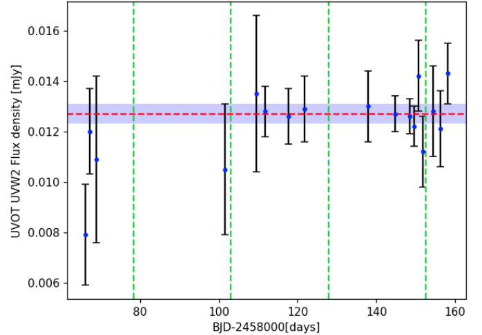
Fig. 2. LHS 1140 UVOT-UVW2 flux-density light curve. Error bars represent the 1\sigma uncertainty. The vertical green dashed lines are the epochs of transit of LHS 1140b. The horizontal dashed red line is the average flux density ( 12.7 \mu\text{Jy} ) as obtained from the analysis of the stacked UV image (Fig. 1) with its 1\sigma uncertainty ( 0.4 \mu\text{Jy} , shaded region).
