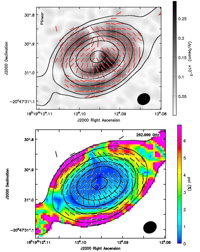
Figure 3. Top panel: composite of the 1.14 mm continuum ALMA Stokes I (contours), polarized intensity (grayscale), and polarization position angle segments (red bars) in the GGD27 MM1 disk. Bottom panel: similar as before, but the color image showing the polarization fraction (here, the polarization position angle segments appear as black bars). In both panels, the contour levels are 3, 10, 50, 120, 200, and 400 K. The wedge shows the scale of the polarized intensity and polarization fraction. The synthesized beam is shown in the bottom-right corner of the panels. Note that the 120 K contour appears at the transition radius, with an almost null polarization ring, between two distinctive polarization patterns.
