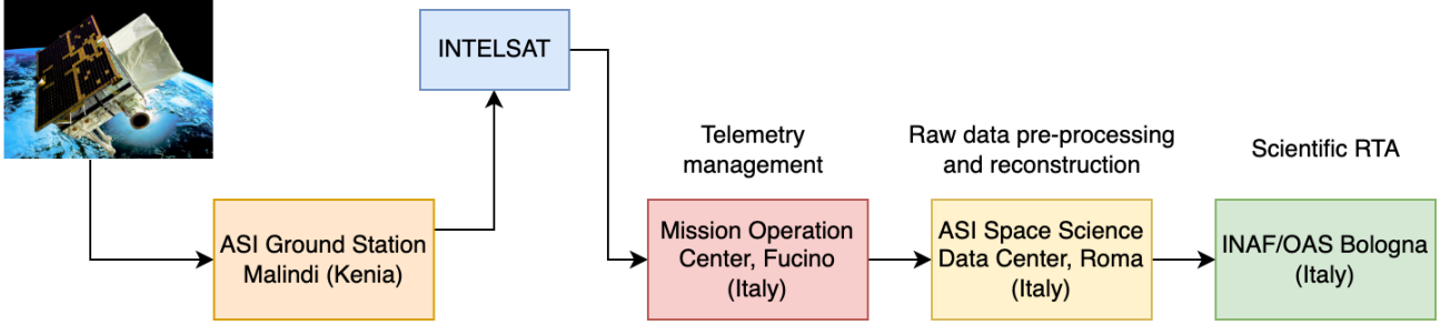
Figure 1: Schema of the AGILE data flow, from the satellite to the scientific pipelines.
