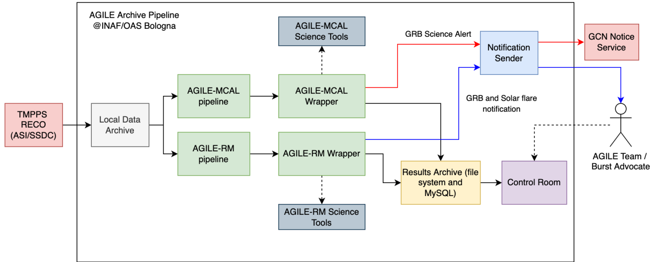
Figure 10: High-level schema of the AP. These pipelines are triggered by the arrival of new data from the ASI/SSDC Science Operation Center (Roma). The pipelines execute analysis to detect transient events (GRBs, TGFs, and solar flares) using the AGILE-MCAL and RM data. When a transient event is detected, the pipelines send an email to the AGILE Team. If the AGILE-MCAL pipeline detects a GRB, it automatically sends a notice to the GCN. The results are stored in the file system and in a MySQL database. The AGILE Team can visualize the results using the Control Room.
