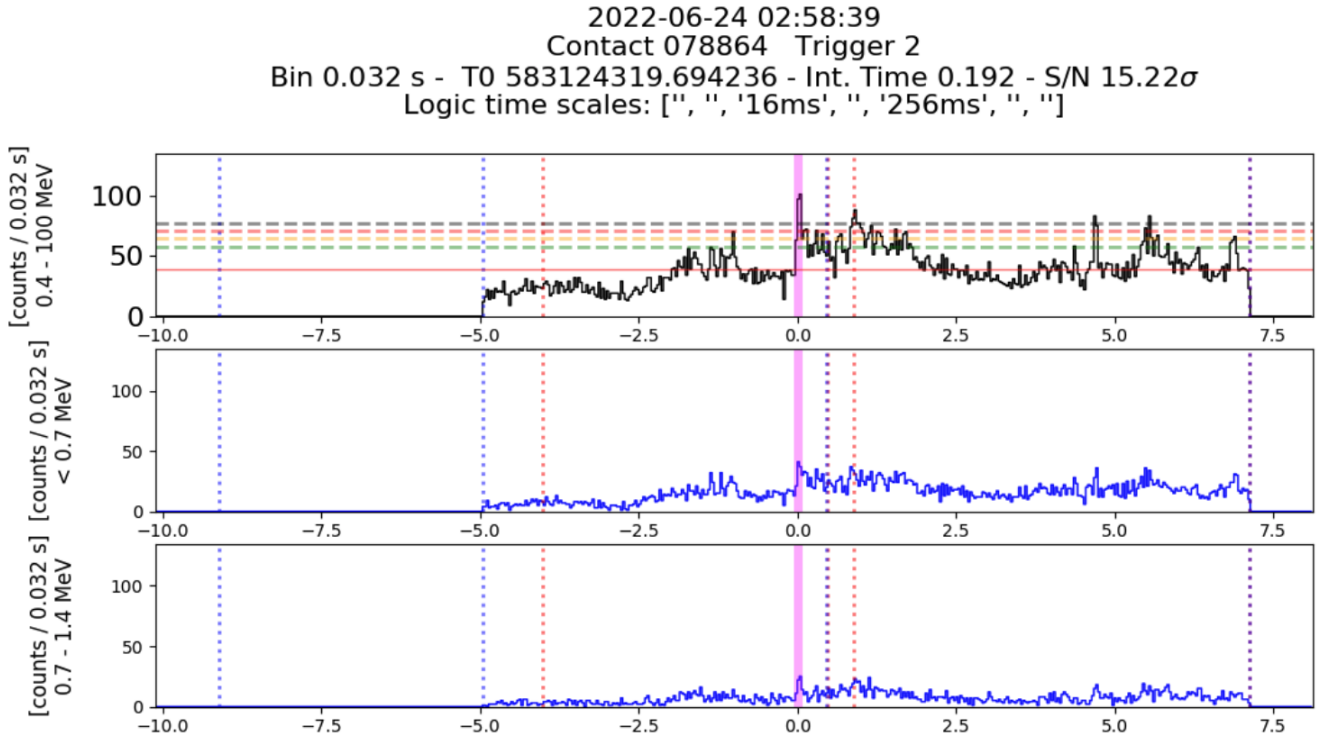
Figure 11: AGILE-MCAL light curve of the GRB220624A at different energy ranges (only the first three bands for space reasons). The dashed horizontal lines represent the different significance levels of the signal. The vertical purple line indicates the peak of the GRB. The vertical dotted lines indicate the on-board trigger logic with the time start and time end of data acquired around the trigger time and the pre/post burst time windows.
