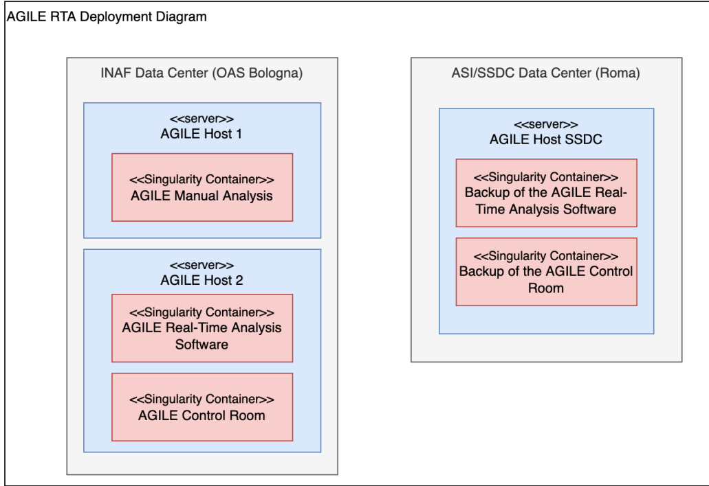
Figure 17: Deployment schema of the AGILE real-time analysis system. The system is deployed in two data centers geographically separated (one in Roma, the other in Bologna) to improve availability in case of failures.
