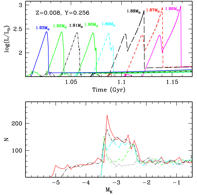
Fig. 3. Top panel: as top panel of fig. 2 but for the chemical composition Z = 0.008 , Y = 0.256 . Bottom panel: LF (0.1 mag bin size) of the upper RGB of \sim 10^6 M_{\odot} clusters for the same chemical composition, and ages t = 1.14 (solid line), 1.12 (dotted), 1.10 (short dashed), 1.08 (long dashed), 1.06 (dot-dashed) Gyr, respectively.
