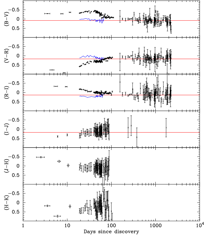
Figure 3. The optical/NIR broadband color evolution of Nova LMC 2009a from day 1 to 2247 post-discovery. The red lines indicate the mean color from day 400 onwards (where data exist). The blue lines show the continuum color corrected for the line emission, as described in the text. The B - V color is bluest near day 40, after which it reddens. The V - R color monotonically becomes bluer, while R - I becomes redder. This reflects the decline in the emission line flux.
