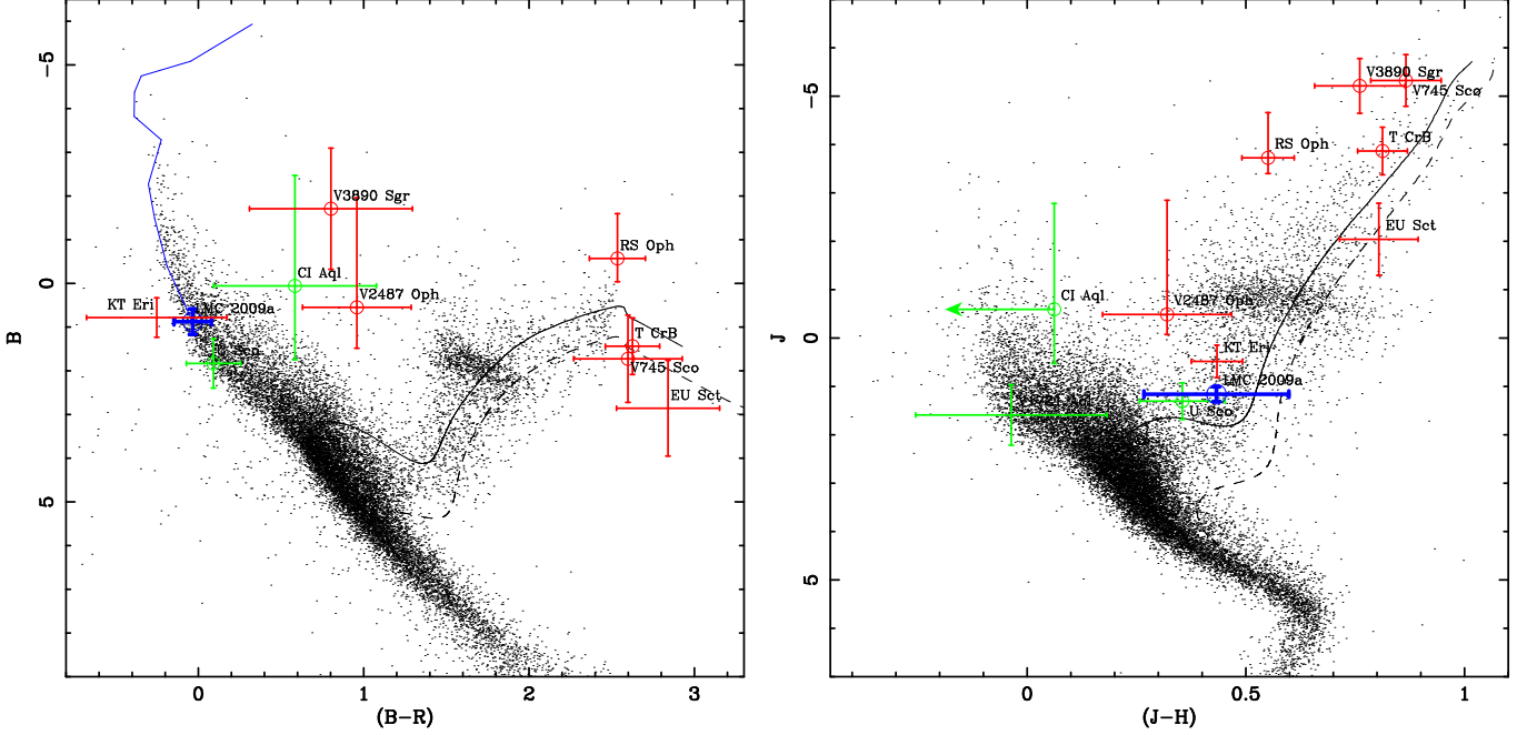
Figure 20. Color-magnitude diagrams showing stars from the Hipparcos data set (black points; Perryman et al. 1997) with parallax errors < 10 percent. These stars have been transformed to the distance and extinction of the LMC as given in the text. B photometry is taken directly from the Hipparcos catalogue, R photometry is taken from the NOMAD1 data set (Zacharias et al. 2005; via the VizieR database, Ochsenbein, Bauer, & Marcout 2000), and NIR photometry from the 2MASS catalogue. The dark blue data point shows the location of the nova LMC 2009a quiescent system, considering the uncertainty in the photometry and extinction. The dark blue line indicates the track of the nova from day 10 post-eruption back to quiescence. The hashed-black and solid-black lines are evolutionary tracks of 1M_{\odot} and 1.4M_{\odot} stars, respectively (Pietrinferni et al. 2004). The red points represent Galactic RG-novae and the green points Galactic SG-novae (see Schaefer 2010; Darnley et al. 2012, and references therein). The known recurrent novae in this sample have been identified by an additional circle. The B vs. (B - R) color-magnitude diagram is very sensitive to the accretion disk in the system, hence the position of LMC 2009a (similar to a massive main sequence star) implies the presence of a luminous and hot disk. The J vs. (J - H) diagram is much less sensitive (in general) to the disk, and more so to the secondary; here the position of LMC 2009a lies around the sub-giant branch or the base of the red giant branch.
