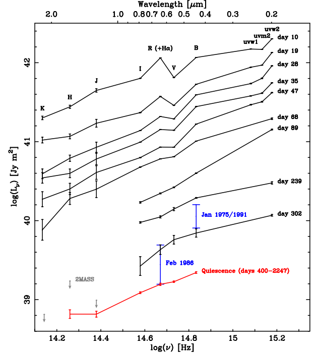
Figure 4. Distance and extinction corrected SED showing the evolution of Nova LMC 2009a from day 10 post-discovery through to quiescence (red data points). The blue data points indicate two independent inter-eruption detections (see Section 3.5). The gray points indicate three inter-eruption upper limits obtained from re-analysis of the 2MASS data. Here only the photometric uncertainties are shown (the magnitude of systematic uncertainties from distance and extinction are shown in the similar Fig. 19). The central wavelength locations of the optical/NIR BVR IJHK filters and the NUV Swift /UVOT uvw1 , uvm2 , and uvw2 filters are shown to assist the reader.
