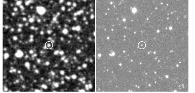
Figure 18. The progenitor of nova LMC 2009a found on an SERC_JDSS1 image taken on 1975 January 10 UT (left) compared with a SMARTS V -band image taken on 2009 December 28 UT (day 326 after discovery; right).
