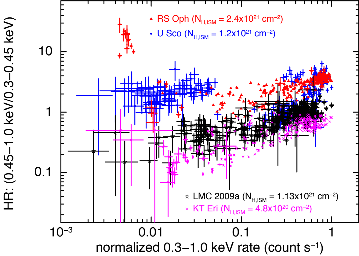
Figure 21. Evolution of the X-ray hardness ratios vs XRT counts for 4 well-observed novae through the SSS phase. Note that in each case the count rate has been normalised to observed peak counts.
