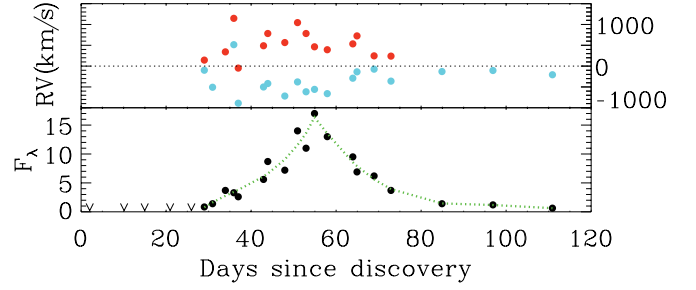
Figure 8. The evolution of the velocities of the components (top panel) and the flux (in units of 10^{-14} erg cm^{-2} s^{-1} ; bottom) in the He II \lambda 4686 line as a function of days since discovery. The radial velocities are of the two components to the line, fit as Gaussians, relative to the rest wavelength of the LMC (dotted line). The lines appear to separate until about day 50, after which they start to converge again. Only a single component is visible after day 80. Absolute fluxes are determined as stated in the text and RMS errors on the measured velocities are estimated as typically around 45 km s^{-1} . No line is visible before day 29 and the flux peaks near day 55. The dotted green line is a third order polynomial independently fit to the rising and falling legs. We attribute no physical significance to the functional form.
