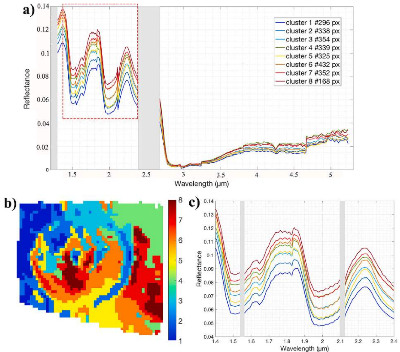
Fig. 12. a) Average spectra (with associated number of pixels) coming from the application of the spectral clustering technique on the 1.5 μm band. This panel shows the eight classes describing variations in grain size, composition, and temperature across the Melkart crater surface. The grey rectangles show the NIMS bad bands that are not considered in this work. b) Spatial distribution of the 8 clusters identified in the NIMS dataset. c) Close up view of panel A, in the 1.4–2.4 μm wavelength range. For A and C panels the colors of the spectra refer to the same colors used for panel B.
