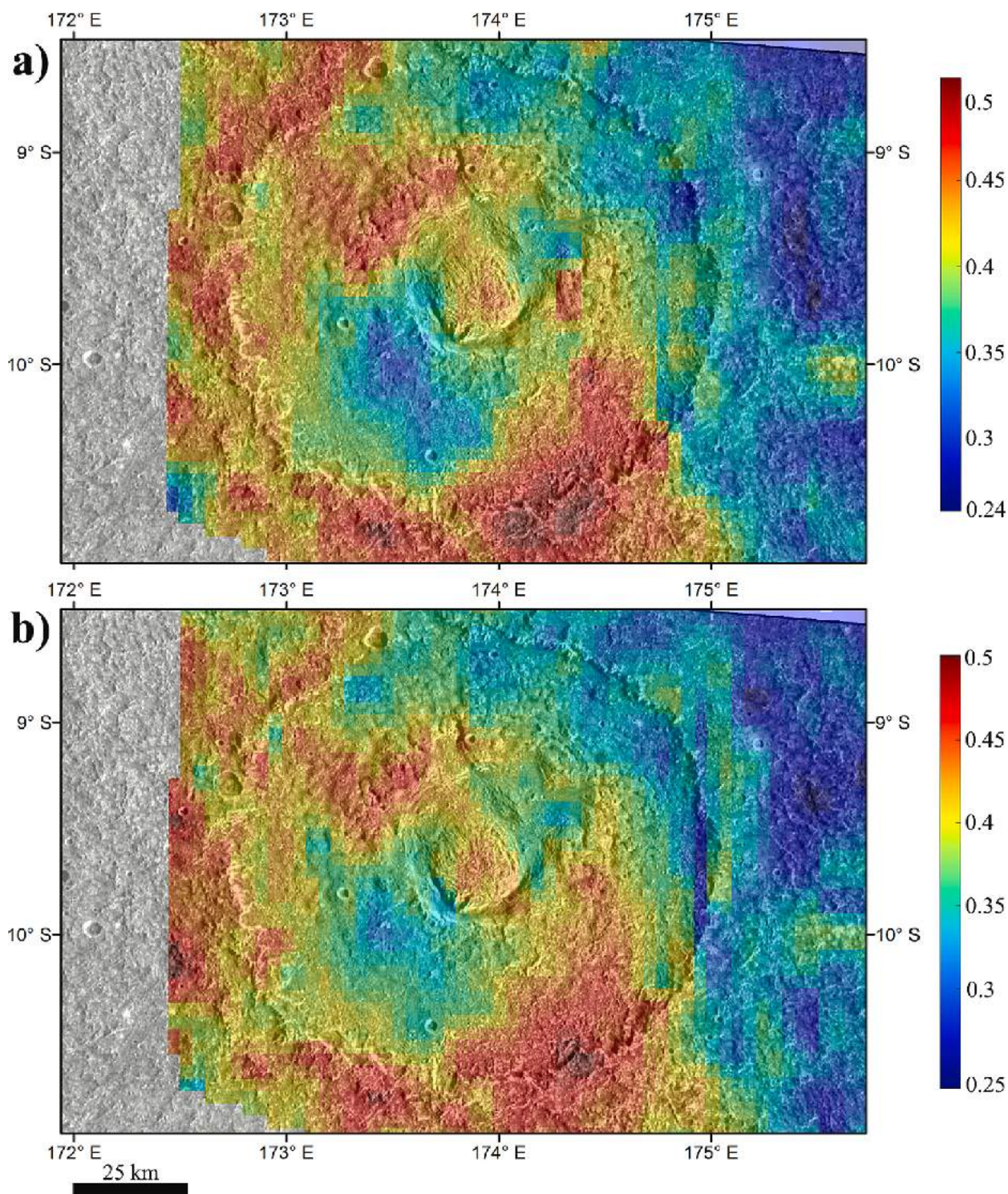
Fig. 11. Colour coded band depth maps of Ganymede's Melkart crater of the H 2 O-ice absorption at (a) 1.5 μm (BD(1.5)) and (b) 2 μm (BD(2)). The BD maps are projected onto the SSI mosaic in order to correlate the spectral behavior with the geological terrains characterizing the area. The BD range values are 0.24–0.52 and 0.25–0.5, for BD(1.5) and BD(2), respectively.
