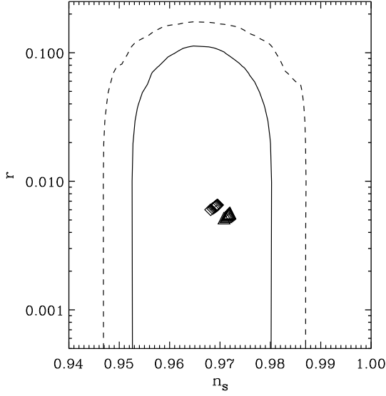
Fig. 2. We compare the theoretical predictions in the r - n_s plane for different values of \alpha for the Planck Collaboration 2015 data release for the TT correlation assuming \Lambda CDM + r [60]. Triangles are for N = 55 and squares for N = 60 e-folds. Solid and dashed lines are the 1\sigma and 2\sigma confidence levels, respectively.
