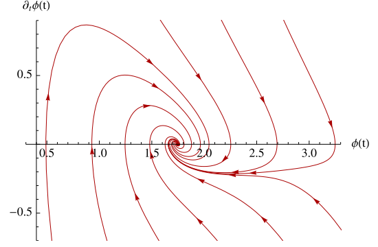
Fig. 4. Phase space evolution in the \phi - \dot{\phi} space for \alpha = 1.5 and \Lambda = 10 . This case arises when V_+(\phi_{\min}) > 0 .
