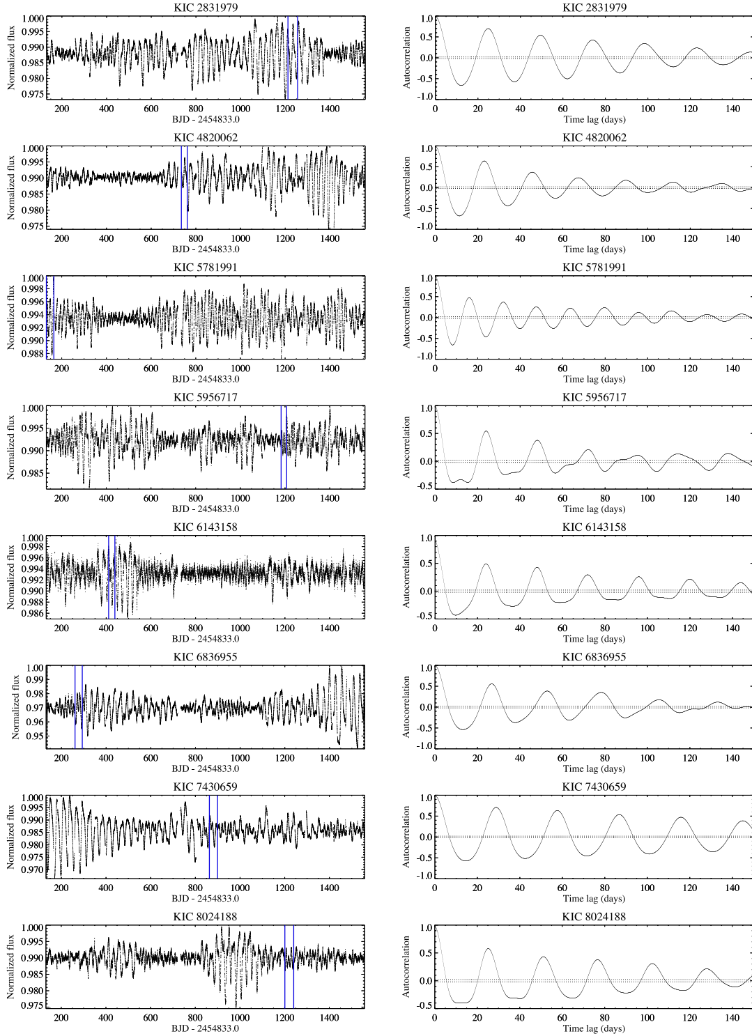
Figure A1. Left: photometric time series of Kepler stars (from top to bottom) KIC 2831979, KIC 4820062, KIC 5781991, KIC 5956717, KIC 6143158, KIC 6836955, KIC 7430659, KIC 8024188, KIC 8037792, KIC 8495770, KIC 9996105, KIC 10079452, KIC 10279927, KIC 10460082, KIC 10514649, KIC 11199277 and KIC 12520213. The flux has been normalized to the maximum value observed along each time series. The vertical solid lines (in blue) display the initial and final times of the intervals considered for MCMC analysis (see Table 1). Right: autocorrelation functions of the LCs of the stars in our sample. The dotted lines indicate the interval corresponding to \pm\sigma , where \sigma is one standard deviation of the autocorrelation as expected for a pure random noise with some degree of autocorrelation according to the large-lag approximation.
