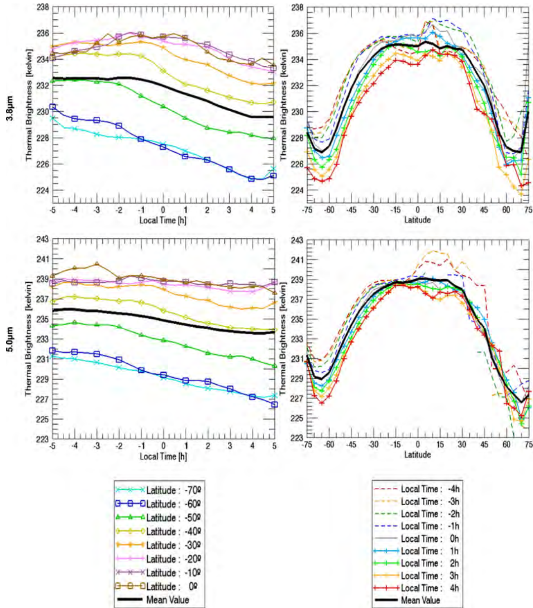
Fig. 16. Profiles of Thermal Brightness at 3.8 \mu\text{m} (top), 5.0 \mu\text{m} (bottom) plotted with respect to local time (left) and latitude (right). The regions close to the terminator and the polar caps are omitted since they are affected by scattered radiation.
