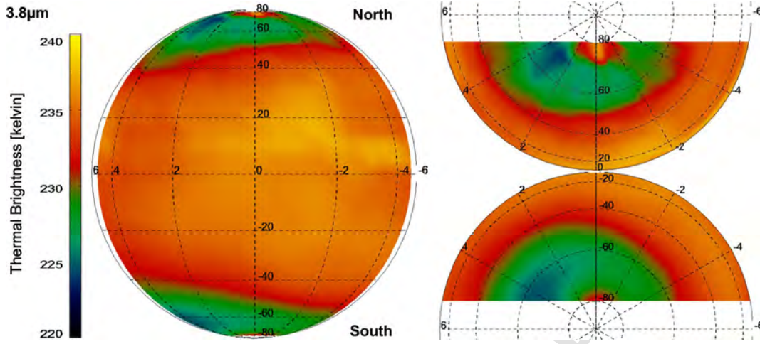
Fig. 14. Thermal Brightness mean map of Venus at 3.8\mu\text{m} , shown in Orthographic projection, distributed along Latitude (north up, south down) and Local Time. The left projection is centred at the anti-solar point (Midnight, Local Time = 00h). The right projections are centred at the poles.
