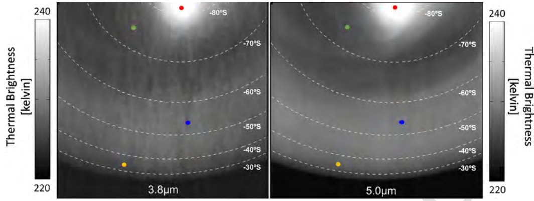
Fig. 6. Comparison of the thermal brightness observed in the two wavelength bands in the same observation (VI0025.07, taken 15 May 2006 at 14:36 UTC) of the southern hemisphere of Venus. The coloured dots mark four representative latitude regions (Red = polar vortex; Green = cold collar, Blue = mid-latitude, Orange = low-latitude). (For interpretation of the references to colour in this figure legend, the reader is referred to the web version of this article.)
