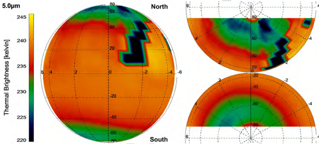
Fig. 15. Thermal Brightness mean map of Venus at 5.0\mu\text{m} , shown in Orthographic projection, distributed along Latitude (north up, south down) and Local Time. The left projection is centred at the anti-solar point (Midnight, Local Time = 00h). The right projections are centred at the poles.
