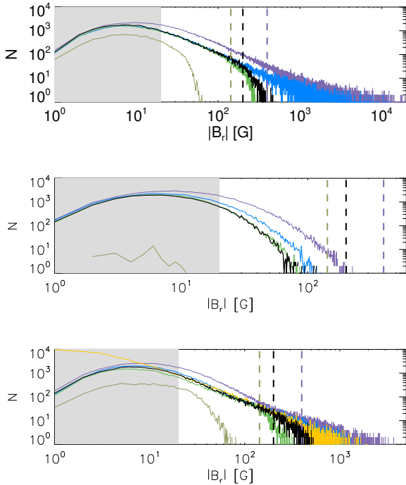
Fig. 1. Histograms of the unsigned radial magnetic flux density |B_r| in magnetograms reconstructed from Ca II K observations taken on 11 August 2001 ( top ), 16 July 2009 ( middle ), and 10 May 2012 ( bottom ). The observations used are from RP (black), MD1 (blue/purple for reconstructions with/without the normalisation of the contrast values to RP, see Sect. 3), SF (dark/light green for reconstructions with/without the normalisation), and SDO/HMI (orange, shown only in the bottom panel as these data are not available prior to 2010) archives. The histograms are produced for bins of 1 G. The vertical dashed lines mark the adopted B_{\text{sat}} value for each archive when using PMOD TSI as the reference, while the grey shaded surface denotes the 3\text{-}\sigma noise level ( \sim 20 G) of the SDO/HMI magnetograms.
