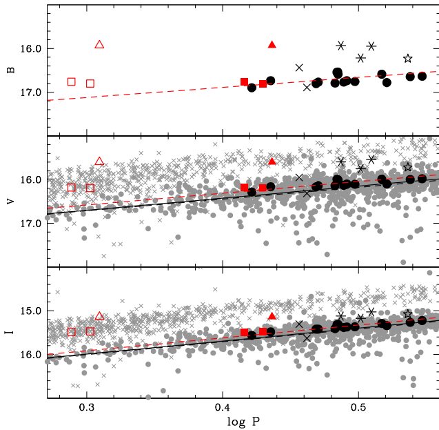
Figure 4. PL relation for NGC 1866 Cepheids in the B , V and I bands. In the V and I bands, our sample is compared with the OGLE one. See the text for symbols.
