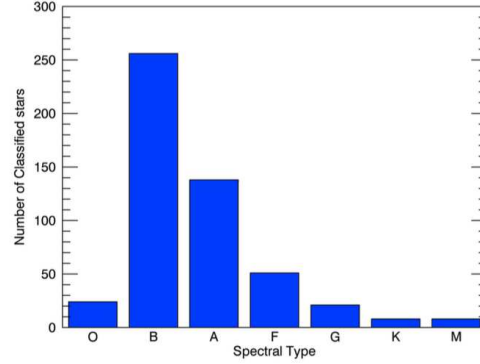
Figure 2. Distribution of the subsample with Spectral Classification as reported in Simbad as function of spectral types. The larger number of B-type stars is a consequence of the presence of a part of the ScoOB1 association and of its nuclear cluster NGC 6231 in the field.
