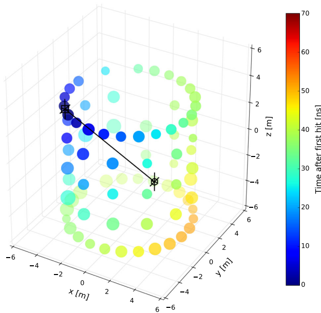
Fig. 15 The arrival time information of light in the PMTs of the muon veto detector (color coded points) allows the approximate reconstruction of the muon track (black line) though the water shield. This example shows an event where the muon traversed the shield close but next to the TPC
