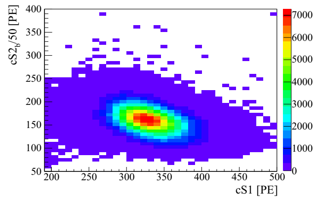
Fig. 24 The position-corrected S1 and bottom S2 signals of the ^{83m}\text{Kr} isomer decay allows for the determination of the light and charge yields at 41.5 keV. The ^{83m}\text{Kr} decay produces two consecutive conversion electrons which are combined for this analysis
