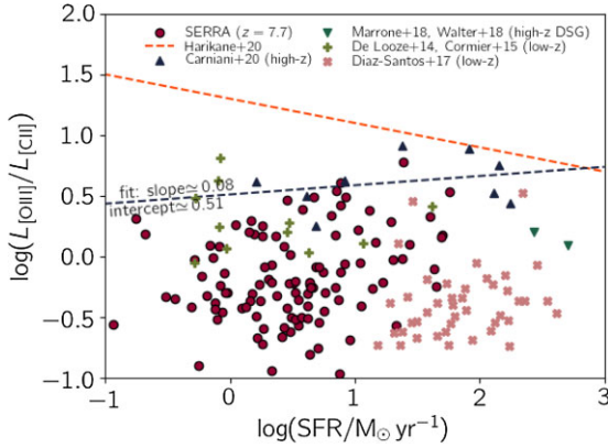
Figure 13. [O III]-to-[C II] ratio as a function of SFR. We plot the collection of observations obtained for normal high- z galaxies ( \text{SFR} < 100 \text{ M}_\odot \text{ yr}^{-1} ; Carniani et al. 2020) and dusty star-forming galaxies ( \text{SFR} > 100 \text{ M}_\odot \text{ yr}^{-1} ; Marrone et al. 2018; Walter et al. 2018), along with data for local normal (Díaz-Santos et al. 2017) and dwarf (De Looze et al. 2014; Cormier et al. 2015) galaxies. We also plot the fits from Harikane et al. (2020) and Carniani et al. (2020, computed in the present, best-fitting parameters indicated in the figure).
