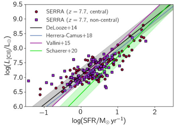
Figure 12. The integrated [C II]–SFR relation found in SERRA. Along with SERRA data at z = 7.7 divided into the central and non-central sample, we show the results obtained from local observations (De Looze et al. 2014; Herrera-Camus et al. 2018), the relation found at z = 4\text{--}6 by ALPINE ( \text{SFR} \gtrsim 10 M_\odot \text{ yr}^{-1} ; Schaerer et al. 2020), and the results from physical motivated models (Vallini et al. 2015, Z = 0.5 Z_\odot ).
