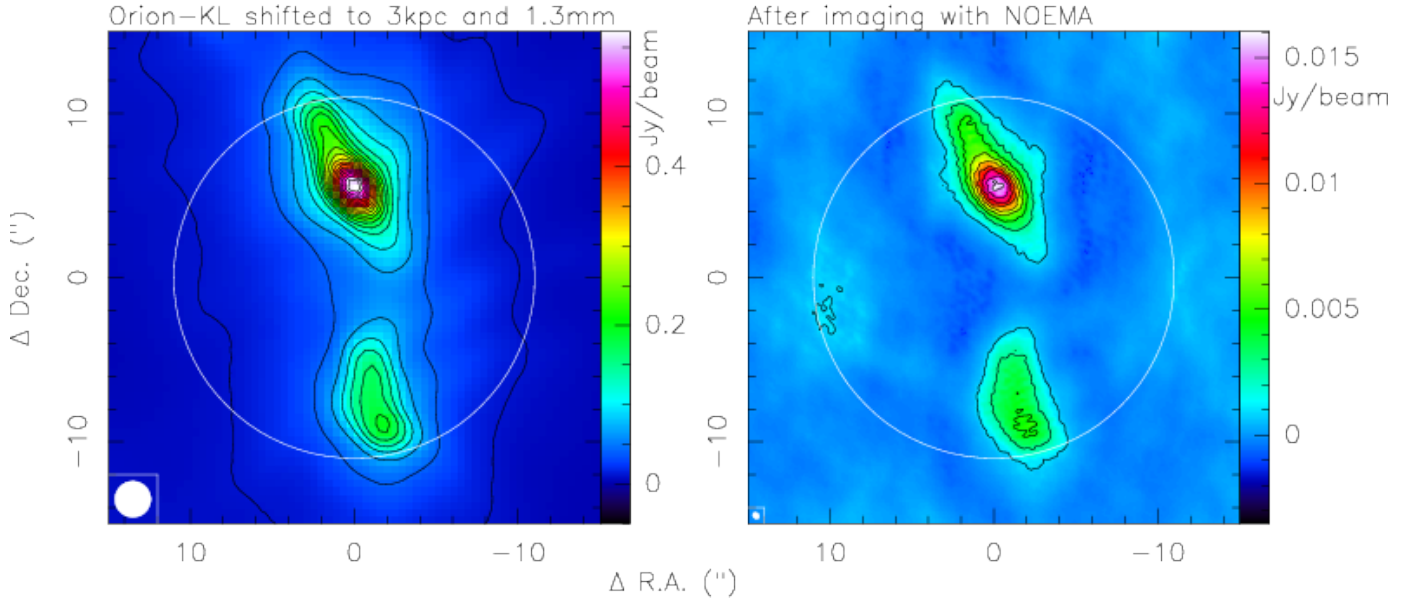
Fig. A.1. Simulated CORE observations at 1.3 mm wavelength using original data obtained for Orion-KL by Lane et al. (2016). For details of the simulations see appendix A. The beam for the left panel (Orion shifted to 3 kpc) is 2.19'' , whereas the synthesized beam of the simulated image in the right panel is 0.44'' \times 0.34'' (P.A. 44 deg). The contours in the left panel start at 10 \text{ mJy beam}^{-1} and continue in 30 \text{ mJy beam}^{-1} steps. The contours in the right image start at 3\sigma and continue in 6\sigma steps ( 1\sigma \sim 0.3 \text{ mJy beam}^{-1} ). The large circles are of 22'' diameter marking the FWHM of the primary beam.
