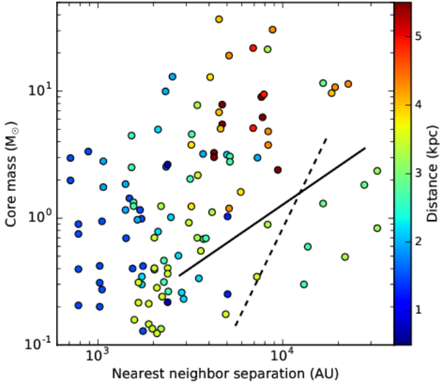
Fig. 13. Fragment masses against nearest neighbor separation from the minimum spanning tree analysis. The full line corresponds to the Jeans lengths and Jeans masses calculated at 50 K for a density grid between 10^5 and 10^7 \text{cm}^{-3} . For comparison, the dashed line corresponds to the Jeans lengths and Jeans masses calculated at a fixed density of 5 \times 10^5 \text{cm}^{-3} (Beuther et al., 2002) with temperatures between 10 and 100 K. The color-coding shows the distances of the sources.
