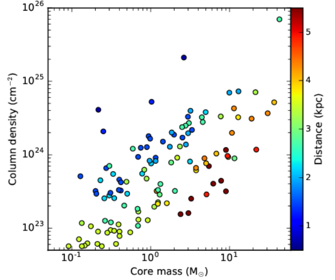
Fig. 9. Gas column densities versus masses for all detected cores. The color-coding shows the distances of the sources.
