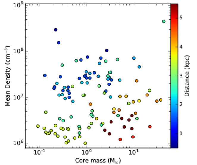
Fig. 10. Mean core densities versus masses for all detected cores. The color-coding shows the distances of the sources.
