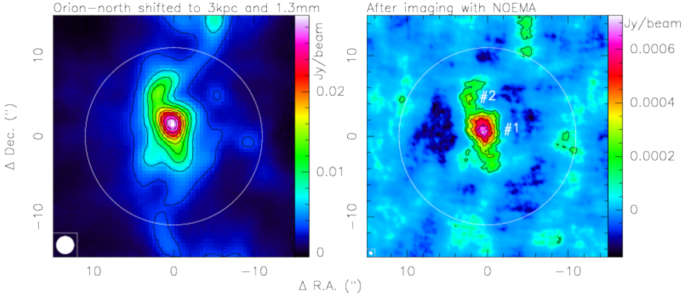
Fig. A.2. Simulated CORE observations at 1.3 mm wavelength using original data obtained for a field in the northern filament of Orion A by Lane et al. (2016). For details of the simulations see appendix A. The beam for the left panel (Orion shifted to 3 kpc) is 2.19'' , whereas the synthesized beam of the simulated image in the right panel is 0.44'' \times 0.34'' (P.A. 44 deg). The contours in the left panel are in 3 \text{ mJy beam}^{-1} steps. The contours in the right image start are in 3\sigma steps ( 1\sigma \sim 0.04 \text{ mJy beam}^{-1} ). The large circles are of 22'' diameter marking the FWHM of the primary beam.
