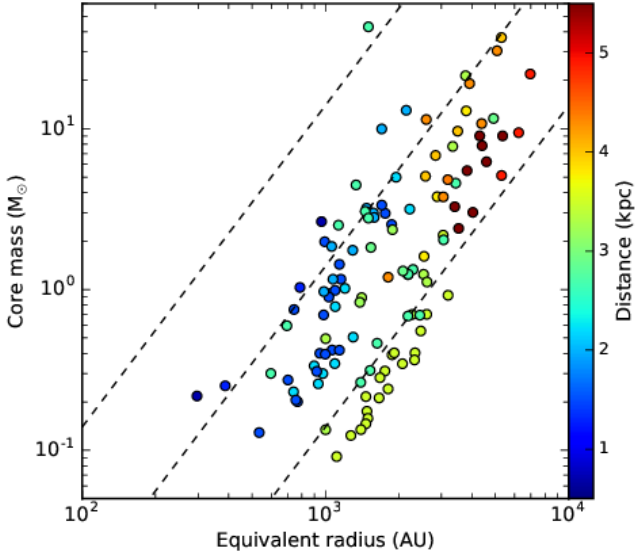
Fig. 11. Core masses versus equivalent radii for all detected cores. The color-coding shows the distances of the sources. The dashed lines show constant column density with levels of 10^{23} , 10^{24} and 10^{25} \text{cm}^{-2} from right to left.
