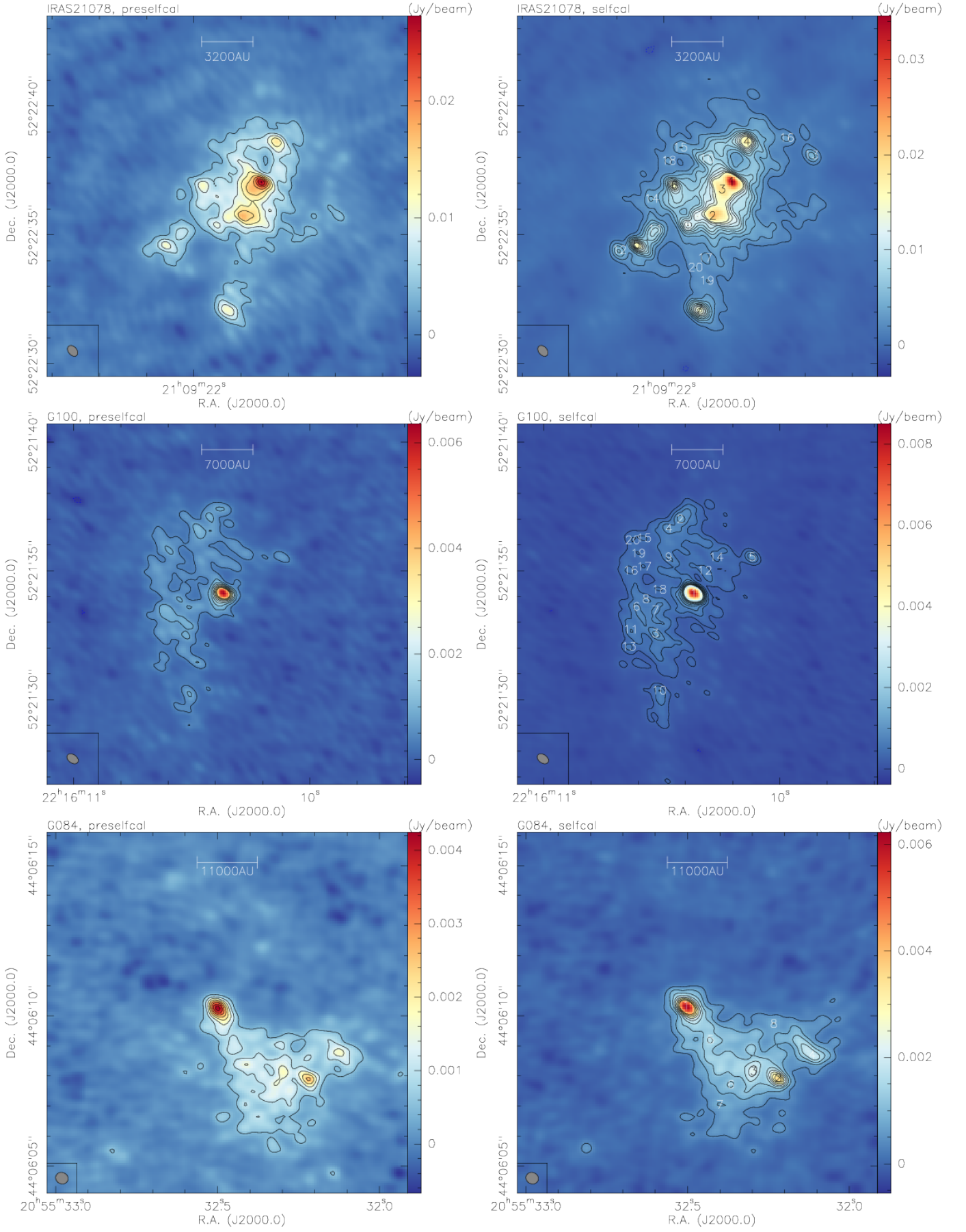
Fig. B.3. 1.37 mm continuum data for CORE sources. The left panels always show the data without applying self-calibration, and the right panels show them after applying self-calibration. The contours are always in 5\sigma steps (see table 3). The right panels mark the cores identified with clumpfind.
