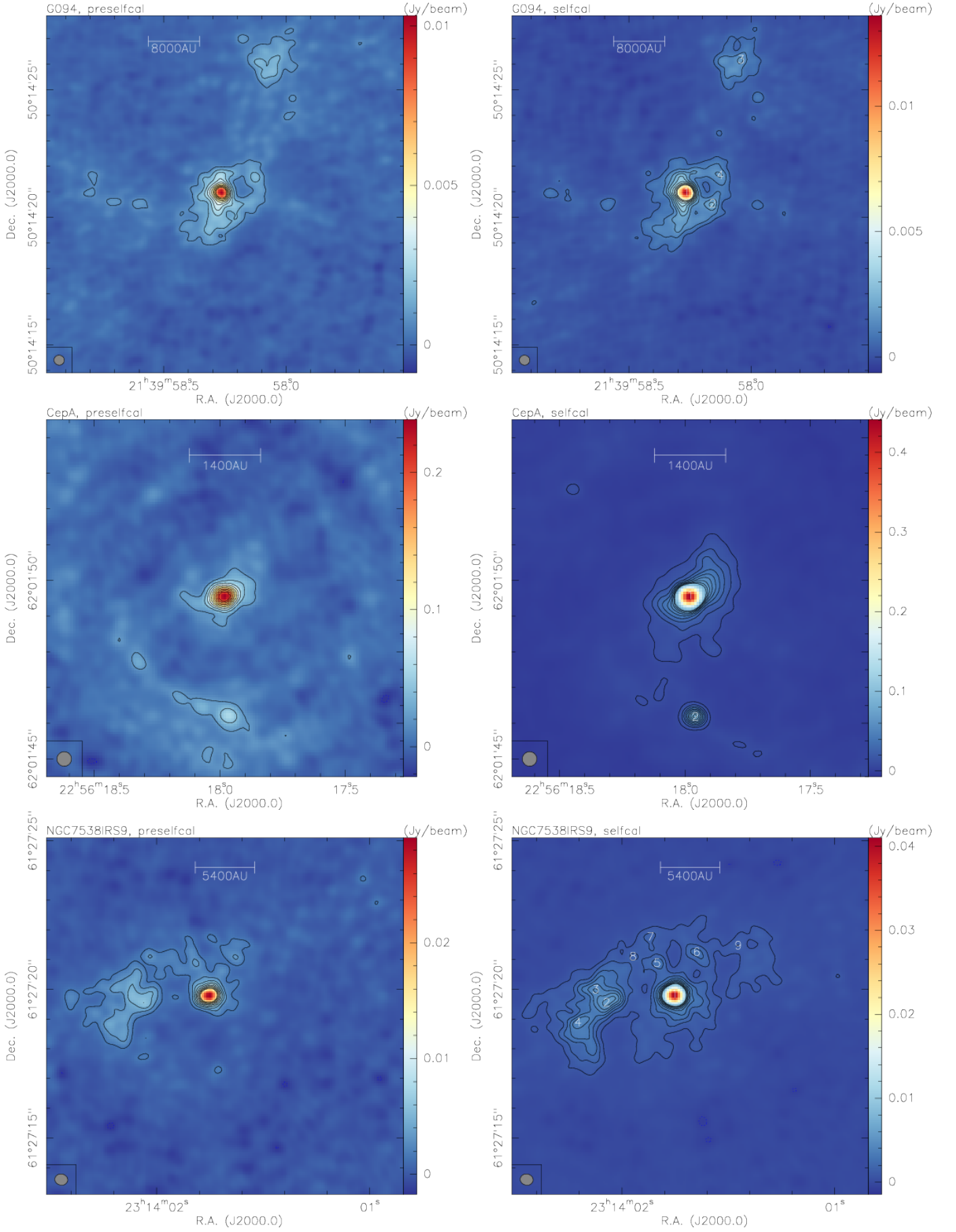
Fig. B.4. 1.37 mm continuum data for CORE sources. The left panels always show the data without applying self-calibration, and the right panels show them after applying self-calibration. The contours are always in 5\sigma steps (see table 3). The right panels mark the cores identified with clumpfind.
