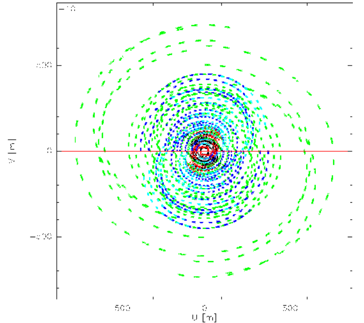
Fig. 4. Example uv-coverage for CepA. The different colors correspond to different observed (half-)tracks. Red and black correspond to D-array observations, blue and cyan to B-array, and green to A-array data.
