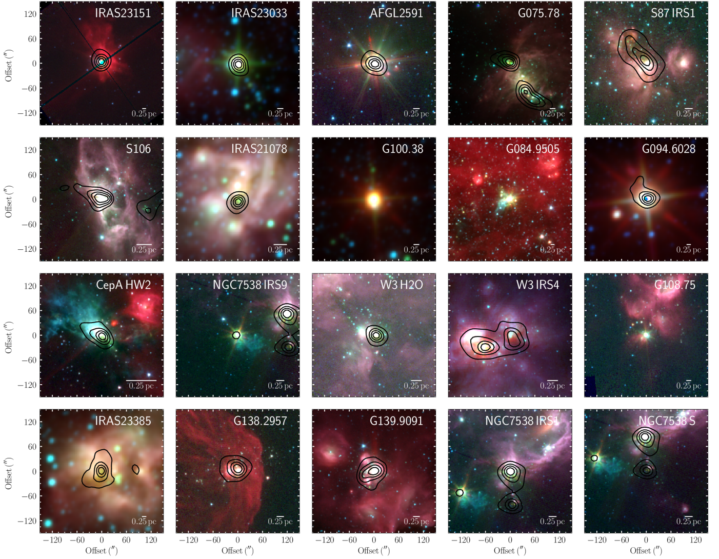
Fig. 2. Large-scale overview images for the whole CORE sample. The color-scale show 3-color images with blue, green and red from Spitzer 3.6, 4.5 and 8.0\,\mu\text{m} for all sources except IRAS 23033, IRAS21078, G100, G094 and IRAS 23385 for which WISE 3.4, 4.6 and 12\,\mu\text{m} data are presented. Furthermore, W3IRS4 uses Spitzer 3.6, 4.5\,\mu\text{m} and MSX 8\,\mu\text{m} . The contours show SCUBA 850\,\mu\text{m} continuum data (di Francesco et al. 2007; contour levels 20, 40, 60, 80% of the peak emission) for all sources except G100, G084 and G108 where these data do not exist.
