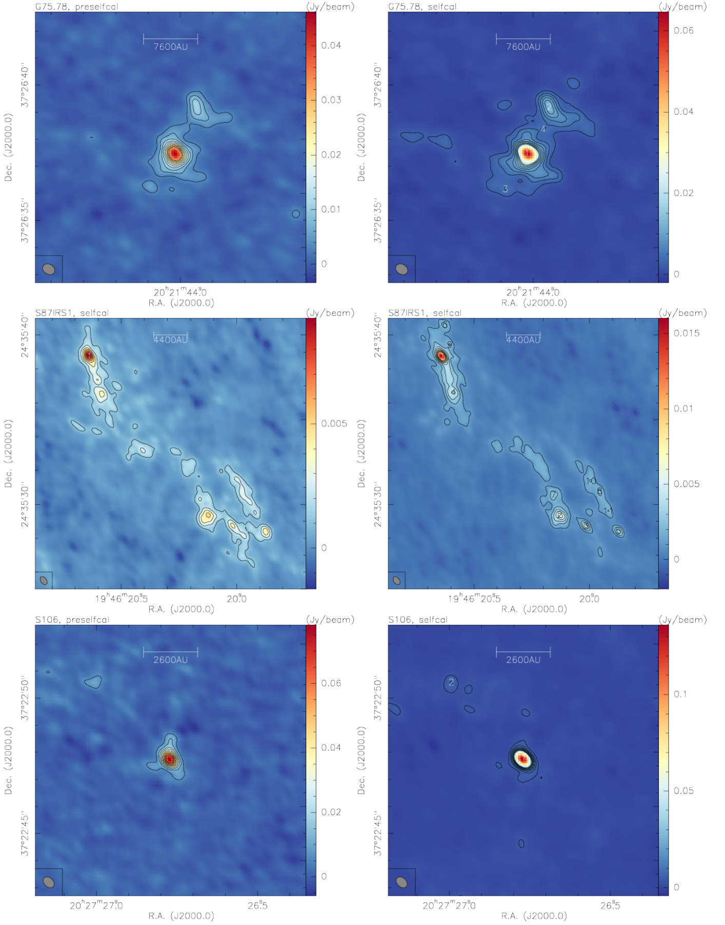
Fig. B.2. 1.37 mm continuum data for CORE sources. The left panels always show the data without applying self-calibration, and the right panels show them after applying self-calibration. The contours are always in 5\sigma steps (see table 3). The right panels mark the cores identified with clumpfind.
