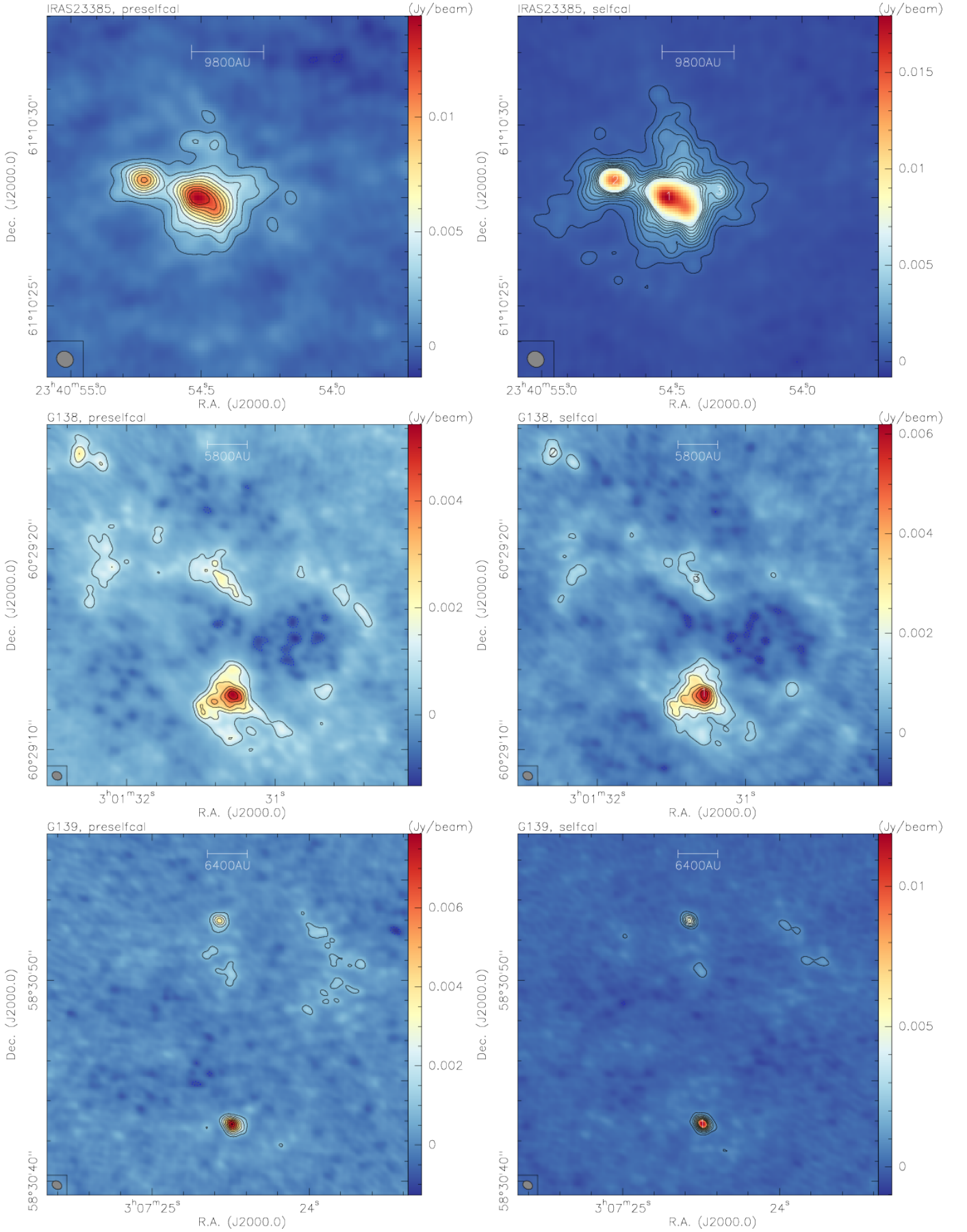
Fig. B.6. 1.37 mm continuum data for CORE sources. The left panels always show the data without applying self-calibration, and the right panels show them after applying self-calibration. The contours are always in 5\sigma steps (see table 3). The right panels mark the cores identified with clumpfind.
