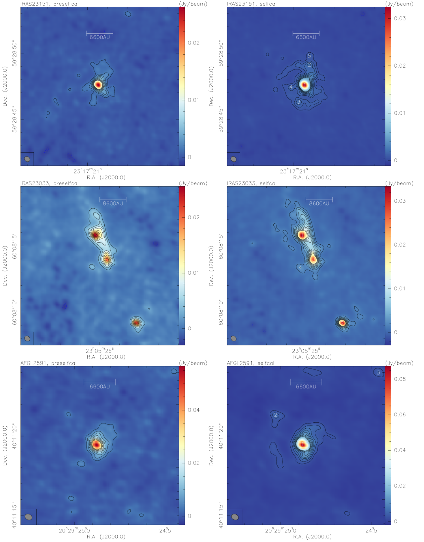
Fig. B.1. 1.37 mm continuum data for CORE sources. The left panels always show the data without applying self-calibration, and the right panels show them after applying self-calibration. The contours are always in 5\sigma steps (see table 3). The right panels mark the cores identified with clumpfind.
