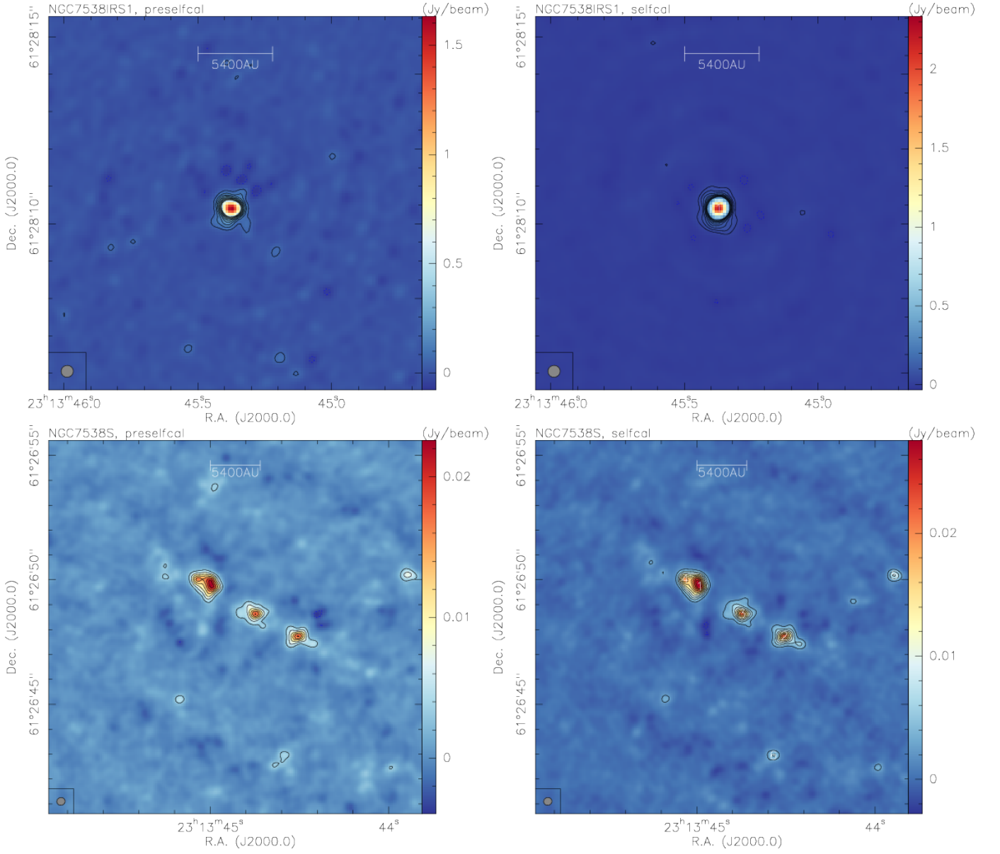
Fig. B.7. 1.37 mm continuum data for two CORE pilot sources. The left panels always show the data without applying self-calibration, and the right panels show them after applying self-calibration. The contours are always in 5\sigma steps (see table 3). The right panels mark the cores identified with clumpfind.
