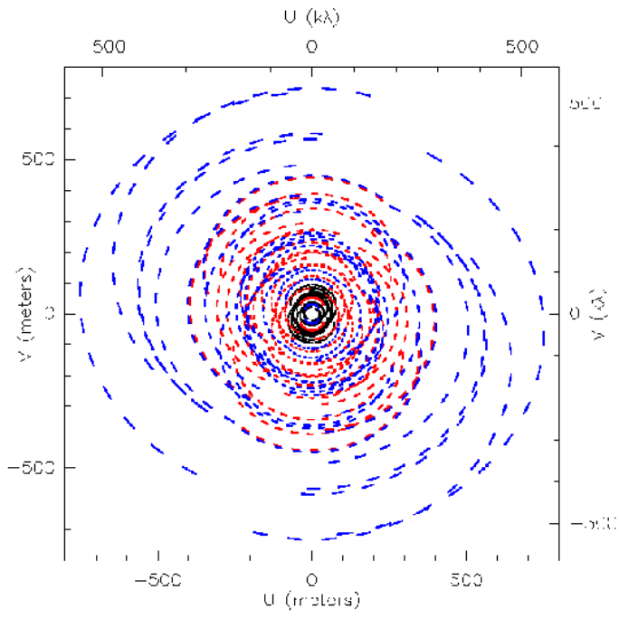
Fig. A.3. Simulated uv-coverage.
