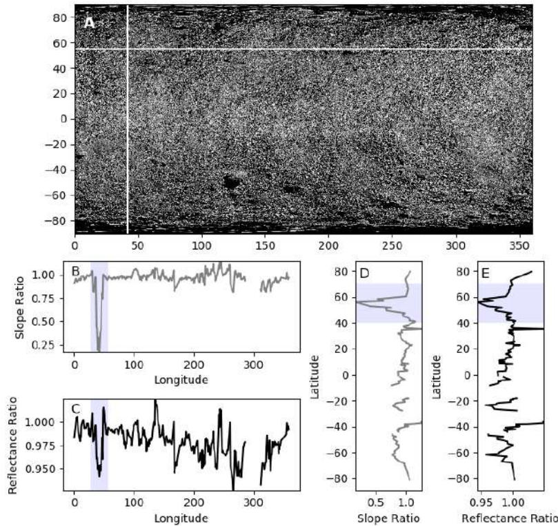
Figure S31. Latitude and longitude transects of spectral slope ratio (BFF/EQ3 spectral slopes from 0.5 – 1.0 \mu\text{m} ) and reflectance ratio (BFF/EQ3 reflectance at 0.55 \mu\text{m} ). (A) Transects were chosen to cover the Nightingale site at \sim 42\text{E} , 55\text{N} . (B, D) The slope ratio is significantly lower at Nightingale (blue box; >5 standard deviations) due to the reddening of BFF slope, which approaches zero in the BFF observations of Nightingale. (C, E) The reflectance ratio at Nightingale is \sim 3 standard deviations lower than other points on the latitude transect (E), however, the longitudinal reflectance ratio transect shows the effect of an increase in detector temperature with time, as the spacecraft scans moved from west to east; even with this effect, Nightingale still has a lower reflectance ratio due to darkening in BFF observations than surrounding longitudes (C).
