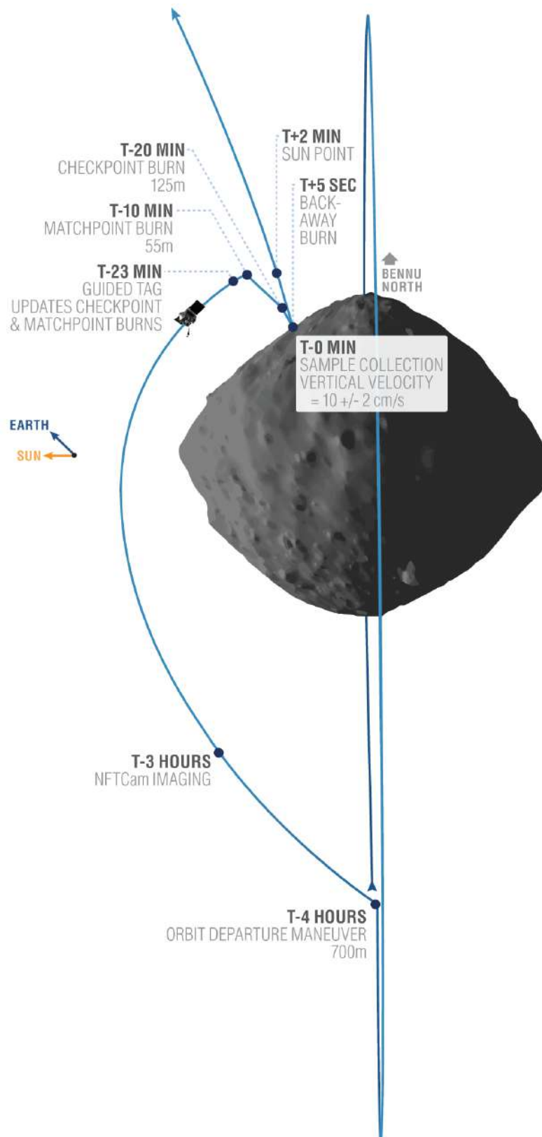
Figure S2. Diagram of the spacecraft trajectory and key events during sampling [1]. Credit: Lauretta et al. 2021.
