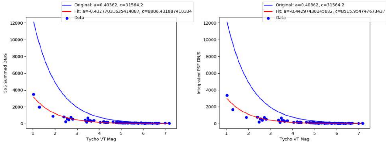
Figure S16. Comparison of conversion from visual magnitude to image intensity before (blue) and after (red) sampling using Tycho VT star magnitudes and a 5x5 summed grid of pixels (left) and the integrated volume of the fit to the point spread function of observed stars (right).
