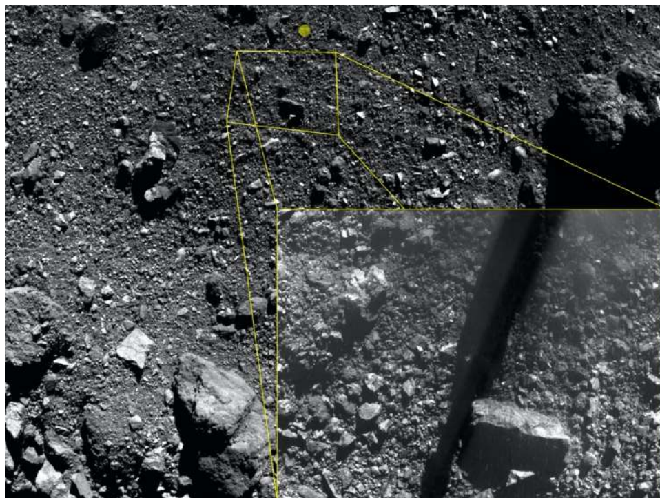
Figure S9. Last pre-contact NavCam 2 image with the contact location in the field of view acquired at 21:46:41.117 UTC. The yellow circle shows the contact location based on correlation with the SamCam image acquired at the time of contact. The inset image (lower right) is the NavCam 2 image acquired at 21:49:50.689 UTC during the initiation of surface contact. In the upper right of the pre-contact image is a boulder which was left undisturbed by the sampling event, indicating material outside of an area \sim 7 m in radius or more from the sample site was unchanged in the immediate aftermath.
