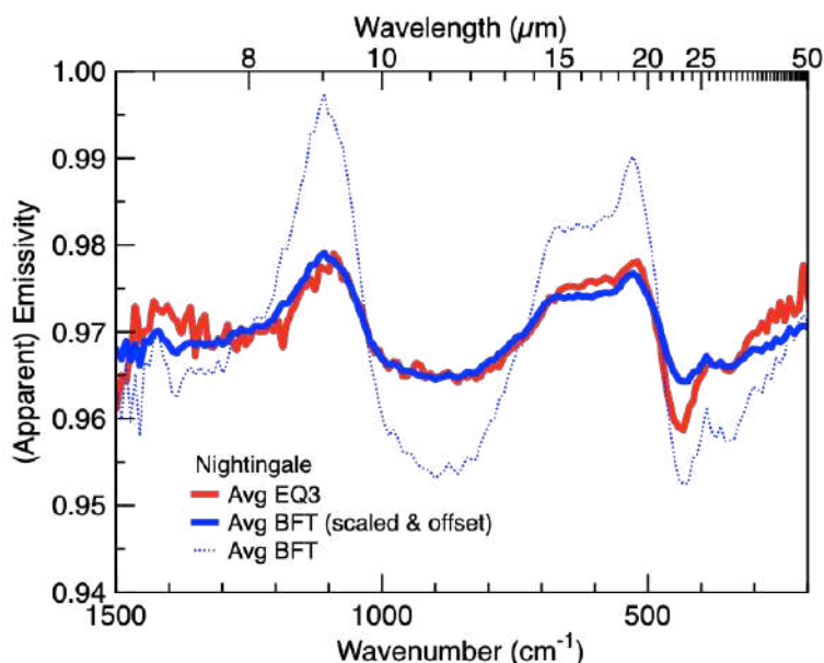
Figure S19. Scaling the final flyby spectrum to a comparable pre-sampling spectrum
