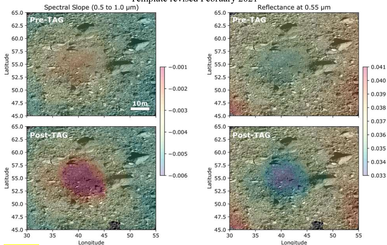
Figure 6. OVIRS spectra show the changes in spectral slope and reflectance resulting from sampling. (A) OVIRS spectral slope before sampling. (B) OVIRS reflectance at 0.55 \mu\text{m} before sampling. (C and D) Same as (A) and (B), but after sampling.
