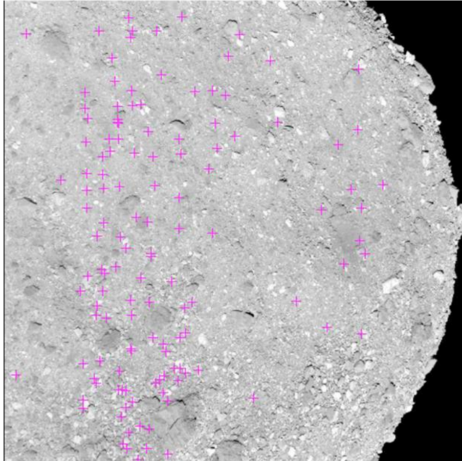
Figure S29. The pre-sampling MapCam image with an overlay of control point locations measured with the overlapping post-sampling MapCam images. The latitude, longitude and radius values of these points were established with the pre-sampling image and held as ground truth in the bundle adjustment.
