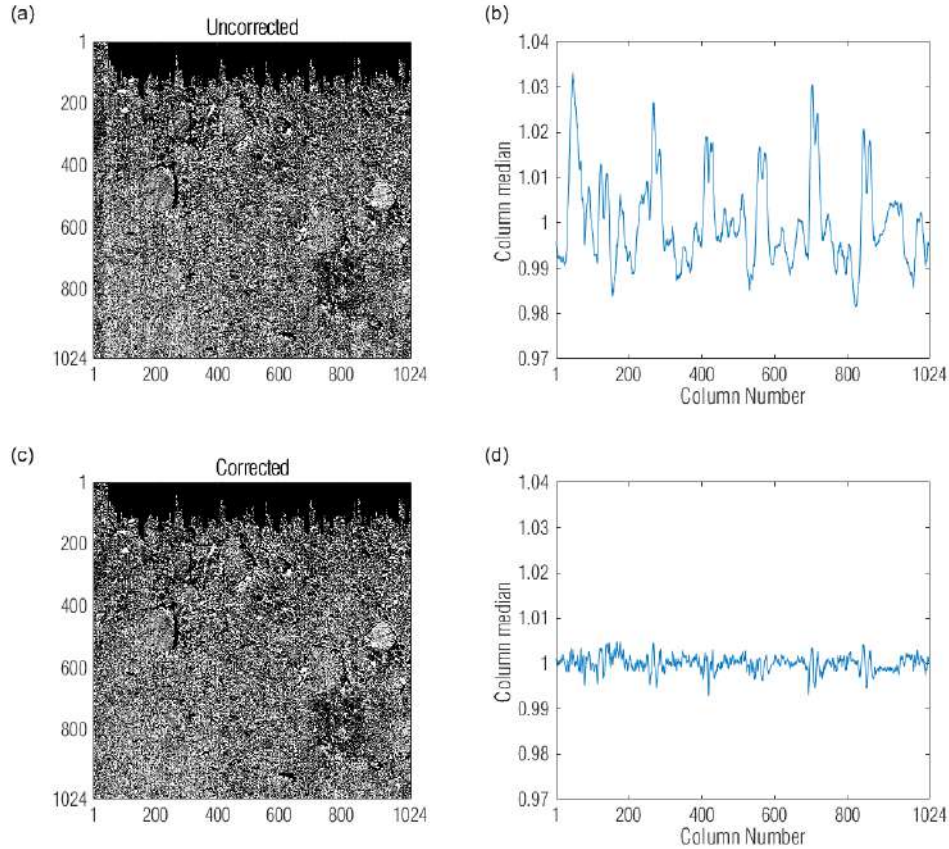
Figure S14. Uncorrected charge smear in FB1 images (a) have a columnar structure (b). Using post-sampling imaging as a reference, we can remove the majority of the artifacts (c and d).
