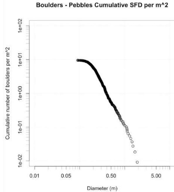
Figure S25. Cumulative number of particles per square meter identified on the Nightingale post-sampling surface.
