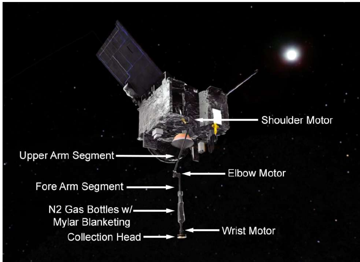
Figure S1. Illustration highlighting the major components of TAGSAM. TAGSAM acquired the bulk sample by releasing a jet of high-purity nitrogen gas that excites and “fluidizes” at least 60 g of regolith into the collection chamber. During the collection time, gas is injected into the surface and subsurface, mobilizing particles into the collection volume. The baseplate of TAGSAM contains 24 contact-pad samplers made of stainless-steel Velcro. These pads collect small particles up to 1 mm in diameter upon contact with the asteroid surface. Image Credit: NASA/Goddard/SVS/CI Lab.
