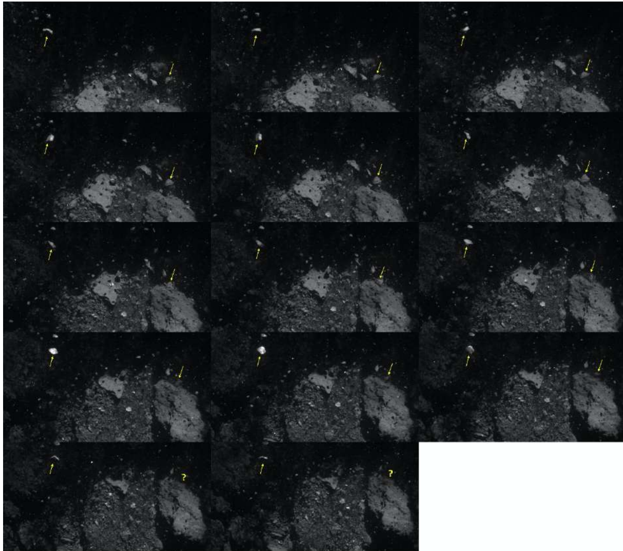
Figure S12. NavCam 2 post-contact image sequence showing two lofted bodies, one second separates each frame. The lofted object on the left is the Tumbling Rock from fig. S10 . The lofted object on the right is the Impactor from fig. S10 . To view the images in a time sequence, see Movie S4 .
