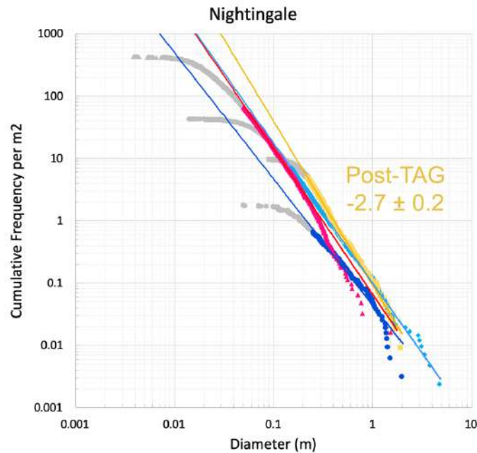
Figure S27. The Nightingale post-sampling SFD compared to the pre-sampling results of Burke et al. (2021).
