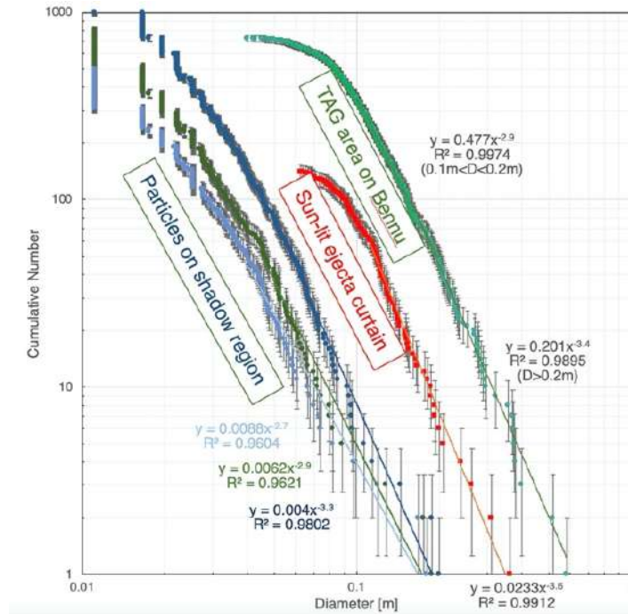
Figure S39. Particles in ejecta curtain generated by the sampling disturbance. (A) A NavCam 2 image of the TAGSAM ejecta curtain (20201020T215045S680_nft_L2). Particles moving in the sunlit side of the curtain are marked with light green. The motion was confirmed by comparing adjacent images. The shadowed region also contains moving ejecta particles. Because of the absence of a bright background curtain, smaller particles could be identified in the shadow region. (B) Comparison among the SFD of particles on Bennu surface near the sampling area, that in the sunlit side of the ejecta curtain, and that in the shadow region. We placed three different threshold brightness levels for finding small particles in the shadow region, but the obtained three SFDs agree with each other within the effort bars.
