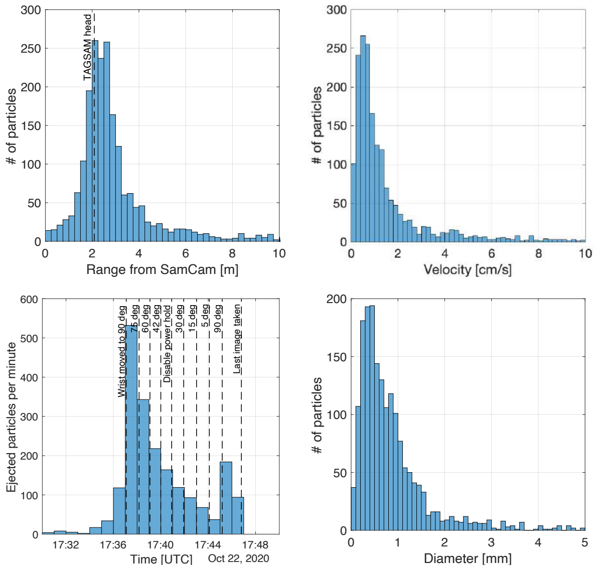
Figure S35. (a) Histogram of estimated range from the camera to each particle at the time of their first observation in 0.25 m bins. The vertical dashed line indicates the approximate range to
