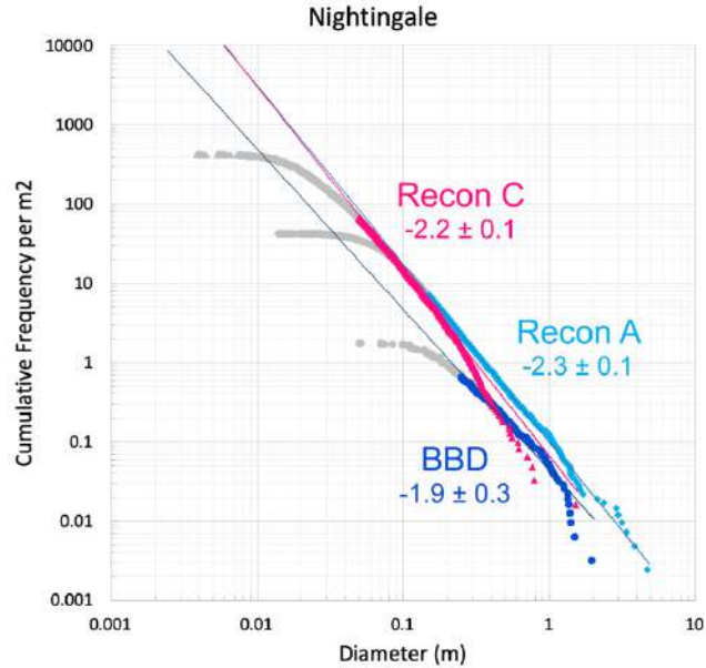
Figure S23. The Nightingale pre-sampling size frequency distributions obtained on the BBD, Recon A, and Recon C imagery datasets, with the corresponding power-law indices obtained above the completeness limits. Particles below the completeness limit are shown in grey. Data from [14].
