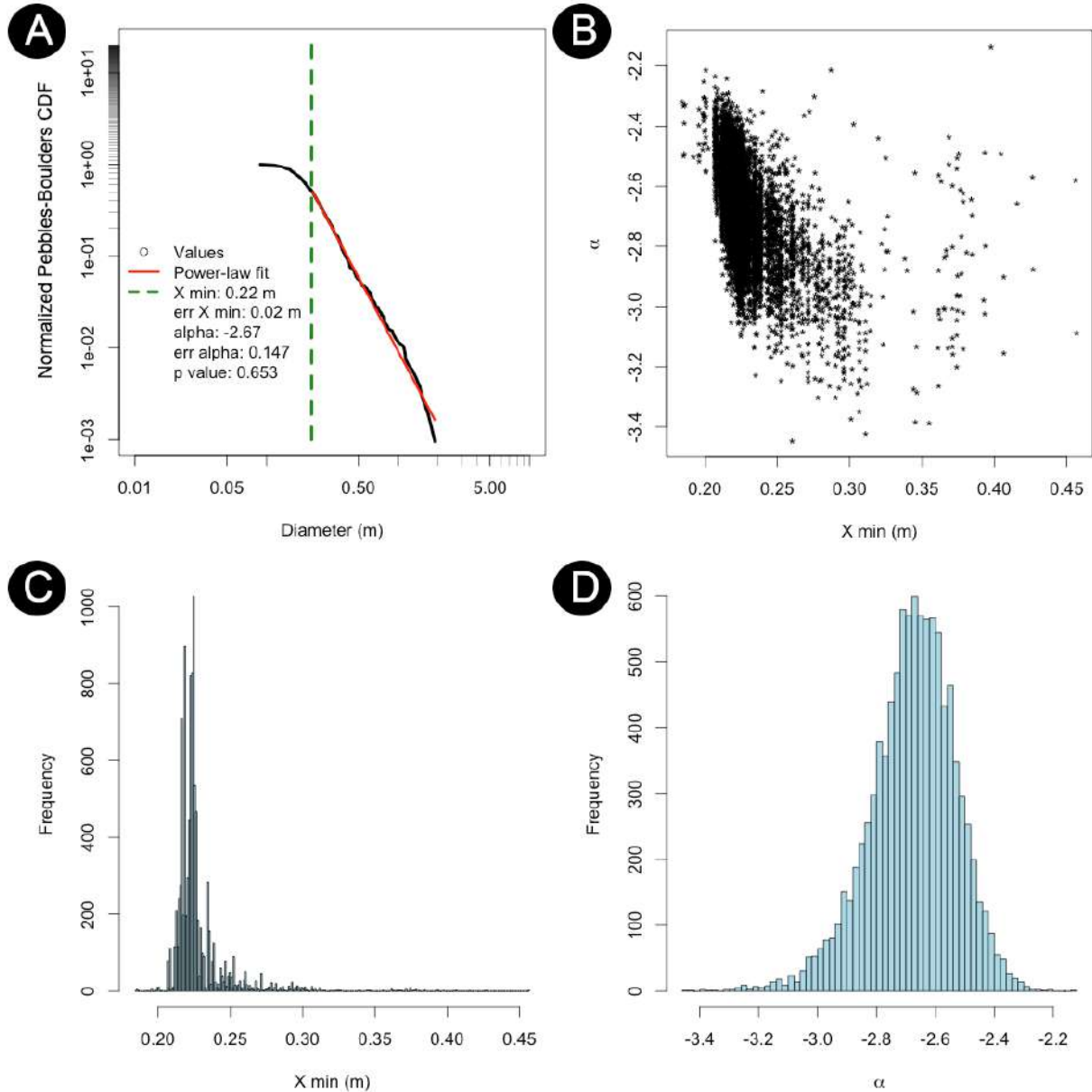
Figure S26. (A) Normalized cumulative distribution function showing the obtained sizes, the power-law fitting curve and the x_{\min} limit. The total number of particles larger than x_{\min} and used for the fit is 561. (B) Scatterplot of x_{\min} against \alpha resulting from 10000 synthetic datasets. (C) Frequency histogram of x_{\min} . (D) Frequency histogram of the power-law index \alpha .
