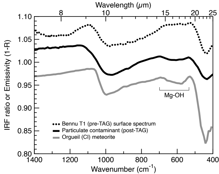
Figure 3. OTES spectra reveal the composition of the sub-mm dust from Bennu's subsurface. Plot showing an example Bennu surface type (T1) spectrum prior to TAG [17], particulate contaminant on instrument post-TAG (IRF ratio), and a representative carbonaceous meteorite, the Orgueil CI chondrite [17]. Spectra are offset vertically for clarity; the Bennu T1 spectrum is shown at 300% contrast to enable comparison of spectral features. The meteorite exhibits a small Mg-OH absorption from \sim 700\text{--}535\text{ cm}^{-1} ( \sim 14.3\text{--}18.7\text{ }\mu\text{m} ) that is common to aqueously altered, phyllosilicate-rich CI and CM chondrites but has been difficult to distinguish in Bennu surface spectra.
