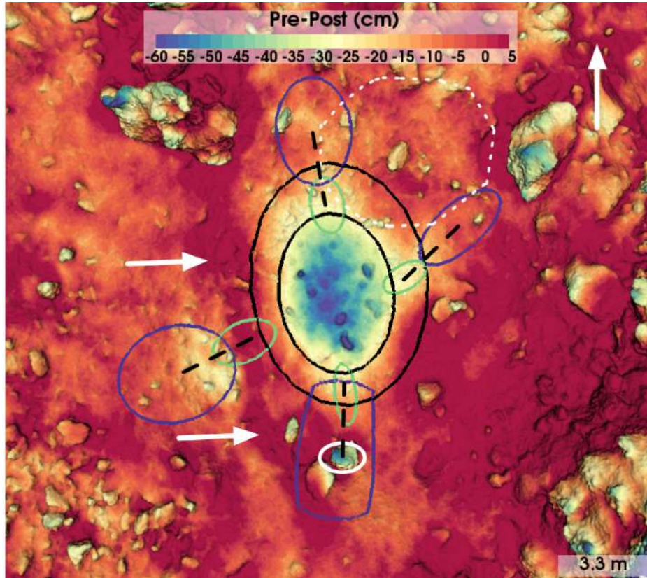
Figure S21. Same as Fig. 4D highlighting features of interest. These include areas influenced by the spacecraft thrusters (light green ellipse for start position and dark purple for final position); a boulder that appears in the scene after sampling (solid ellipse); white arrows indicate location where debris might have been deposited during surface relaxation ( ). Black ellipses show two bounding cases for the post-TAG crater used in this analysis: the smaller limit measures 6.0x4.3m or 5.1±1.2 (Total displaced volume=8.6±0.9 m -3 ) and is delineated by the inner edge of the estimated thruster plume locations, and thus results from TAGSAM gas release. The large crater is likely a combination of both TAGSAM and thruster firing during the backaway burn and measures 9.0x6.5m or 7.8±1.8m (Total displaced volume = 12.2±0.9 m -3 ). Black dotted lines approximately connect the maximum thruster pressures at the start and end of the departure maneuver [15]. Dotted region to the north and north-west of indicate regional readjustment.
