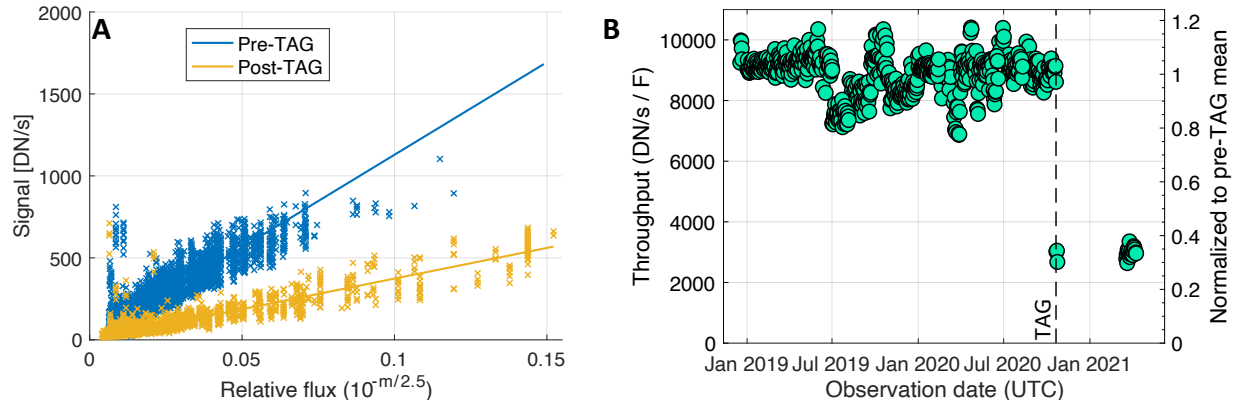
Figure S15. (A) Measured star signals for NavCam 1 as a function of expected relative flux according to the UCAC4 star catalog V-band magnitude. Pre-sampling (blue) is all stellar observations from 10 August to 20 October 2020 with their linear fit, the slope of which is the measured throughput. Post-sampling (yellow) is all stellar observations from 21 to 23 October 2020 and 19 March 19 to 9 April 2021 with their linear fit. (B) Measured NavCam 1 throughput over time for stellar observations binned by observation date. The vertical dashed line denotes when sampling occurred on 20 October 2020.
