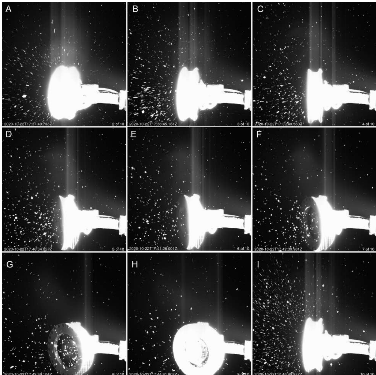
Figure S34. SamCam images acquired on October 22, 2020, during the TAGSAM post-sampling checkout. These long (1.5 s) exposure images highlight the escaping particles, which appear as radiating lines due to their relative motion during the image exposure period.
