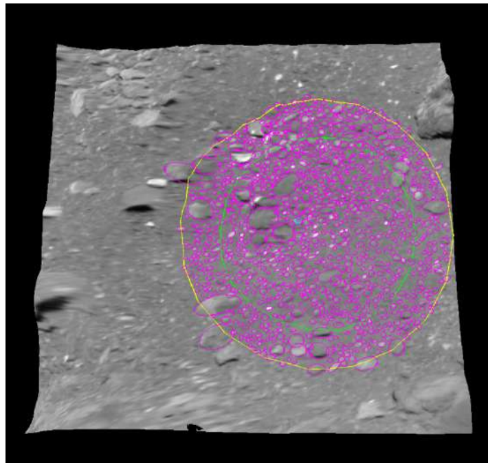
Figure S24. The 1048 particles identified inside the Nightingale site post-sampling. The light blue circle is the estimated contact spot (30 cm). The green circle is the 80 percent 2 sigma sampling site (8.6 m size). The yellow circle is the actual 11.8 m circle where we counted all particles. The image in background is ocams20210407t062114s948_pol_iofl2pan_536373.fits (pixel scale of 5 cm) overlaid on the post-sampling DTM.
