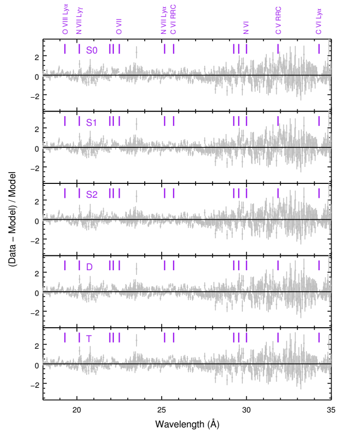
Fig. 3. As Figure 2 in the 18–35 Å band.
