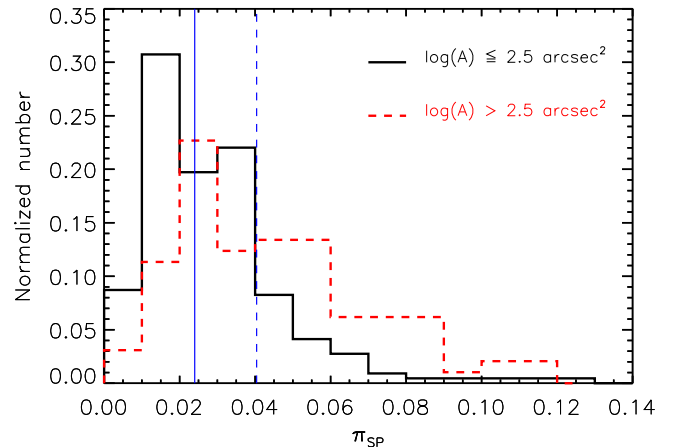
Figure 18. The \pi_{\text{SP}} distributions of the unresolved (black solid line) and extended (dashed red line) steep-spectrum objects in the NVSS survey. The deconvolved surface area thresholds \log(A) \leq 2.5 \text{ arcsec}^2 and \log(A) > 2.5 \text{ arcsec}^2 are used to separate unresolved and extended sources, and the two vertical blue solid and dashed lines represent the medians of \pi_{\text{SP}} for the two samples, respectively.
