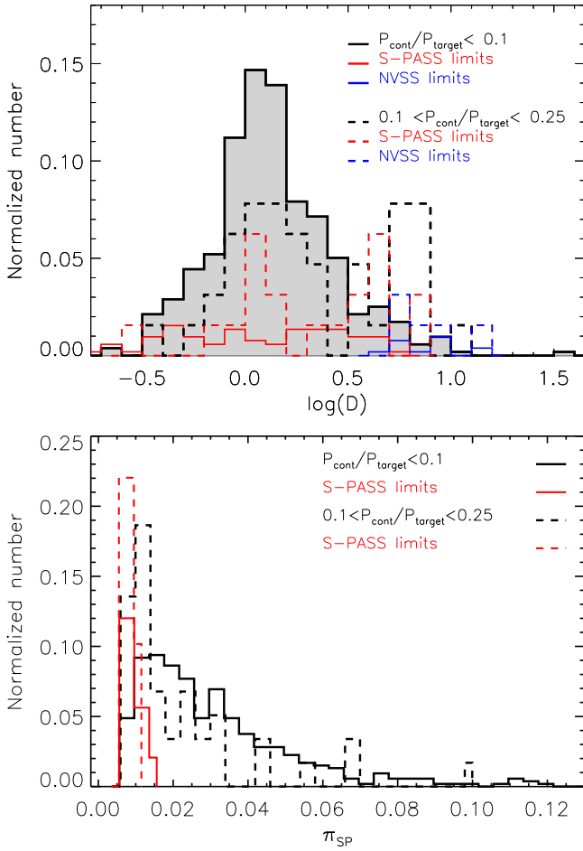
Figure 5. Distribution of \log(D) (top) and 2.3 GHz fractional polarization \pi_{\text{SP}} (bottom) of objects with \frac{P_{\text{cont}}}{P_{\text{target}}} < 0.1 and 0.1 < \frac{P_{\text{cont}}}{P_{\text{target}}} < 0.25 are shown with solid and dashed lines, respectively. Black, red, and blue represent objects with detection, upper limits in S-PASS, and upper limits in NVSS polarizations. The area under the \log(D) histogram of objects with \frac{P_{\text{cont}}}{P_{\text{target}}} < 0.1 and detected polarization flux densities is colored in gray for clarity.
