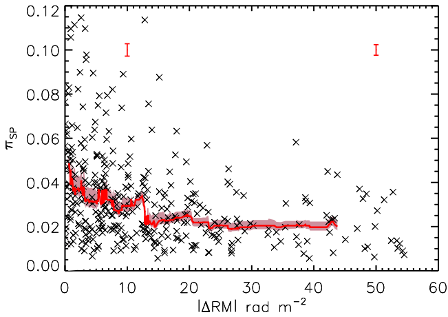
Figure 16. S-PASS fractional polarization vs. the |\Delta RM| , which is a representation of the Faraday structure.
