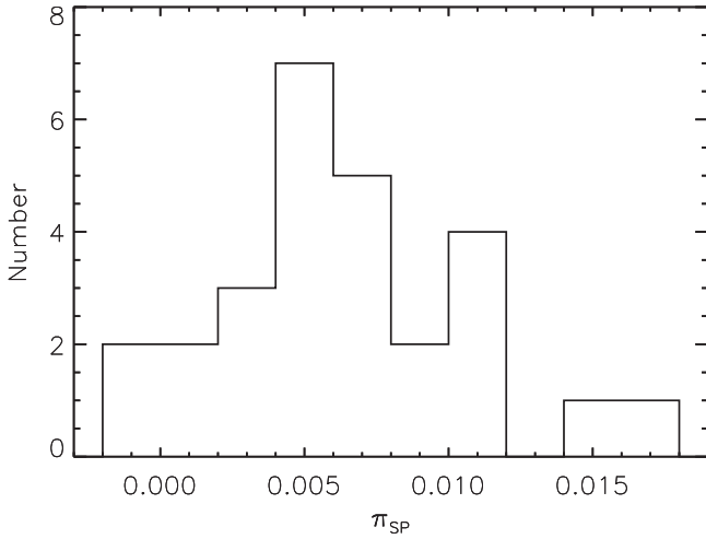
Figure 2. Distribution of S-PASS fractional polarization for 27 objects with \pi_{\text{NV}} < \epsilon_{\text{NV}} .
