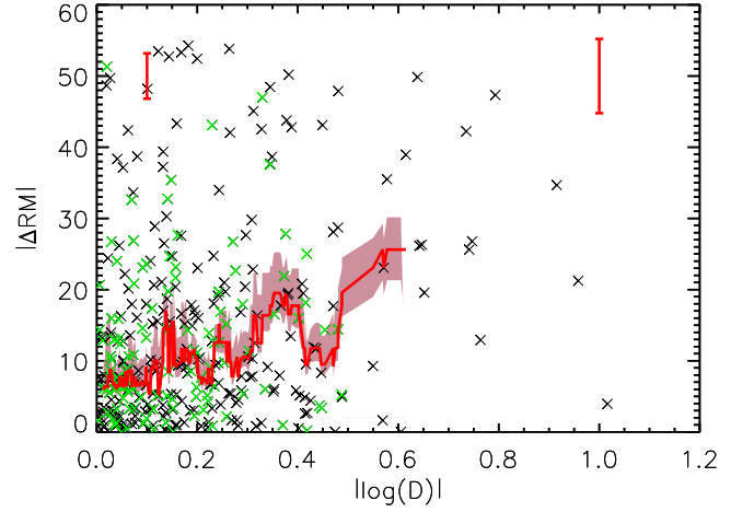
Figure 14. Absolute difference between rotation measures calculated in this work and in TSS09, |\Delta\text{RM}| vs. |\log(D)| . The black and green crosses represent depolarized and re-polarized objects, respectively. The solid red line is the running median of |\Delta\text{RM}| calculated for bins of 23 objects in |\log(D)| space which include both depolarized and re-polarized sources and the dark-pink shaded region is the estimated uncertainty on the running medians. The error bars on the left and right upper corners are the medians of intrinsic uncertainties in |\Delta\text{RM}| for the two halves of the data.
