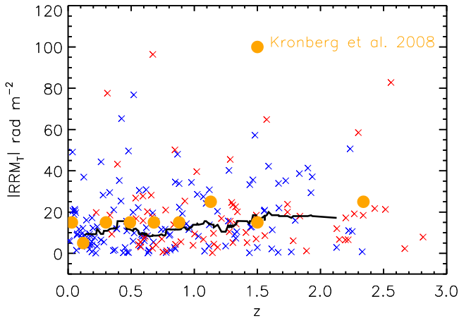
Figure 23. Distribution of the |\text{RRM}| for the 206 objects is plotted vs. redshift, z . The blue and red crosses represent objects with \alpha < -0.5 and \alpha \geq -0.5 . The solid black line shows the running medians of the |\text{RRM}| of all sources. The orange filled circles are the data points extracted from Figure 3 of Kronberg et al. (2008) as discussed in Section 5.5. Each circle represents the median value of their |\text{RRM}| for each redshift bin.
