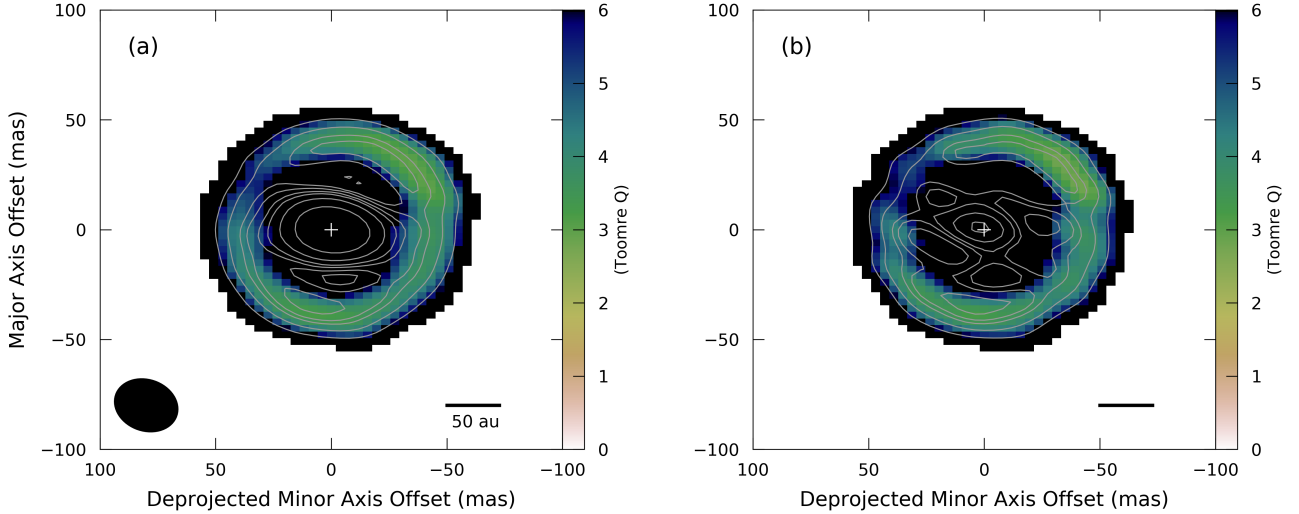
Fig. 3. Panel a: Toomre Q map of G17.64 using the dust emission with the minimum free-free fraction subtracted for the mass surface density. Panel b: same as (a), but the maximum free-free contamination was removed before the mass surface density was calculated. The synthesised beam is indicated at the bottom left of the left figure and a scale to the right, while the grey contours are those shown in Figs. 1a and b. Values below the 10\sigma dust continuum emission level are masked out. The maps are centred (0,0) on G17.64 but are rotated by the PA ( 25.9^\circ ), aligning the disc major axis in the north-south direction. The disc is deprojected along the minor axis using the inclination of 40^\circ in the image plane.
