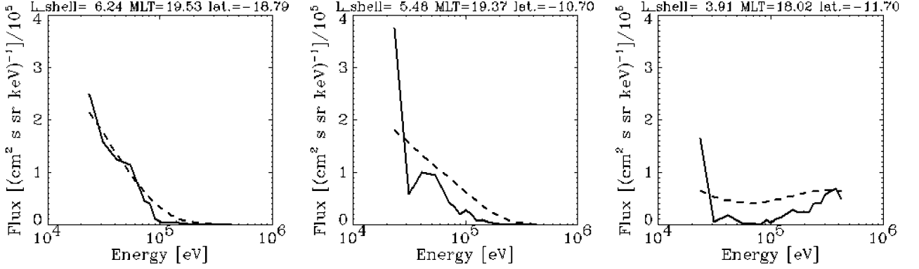
Figure 3. Comparison between modeled (dashed lines) and observed (solid lines) proton spectra at three different MLT and L_{\text{shell}} . The data were collected by the CRRES/MICS instrument in the energy range 20–300 keV, during a quiet time period (18 April 1991).
