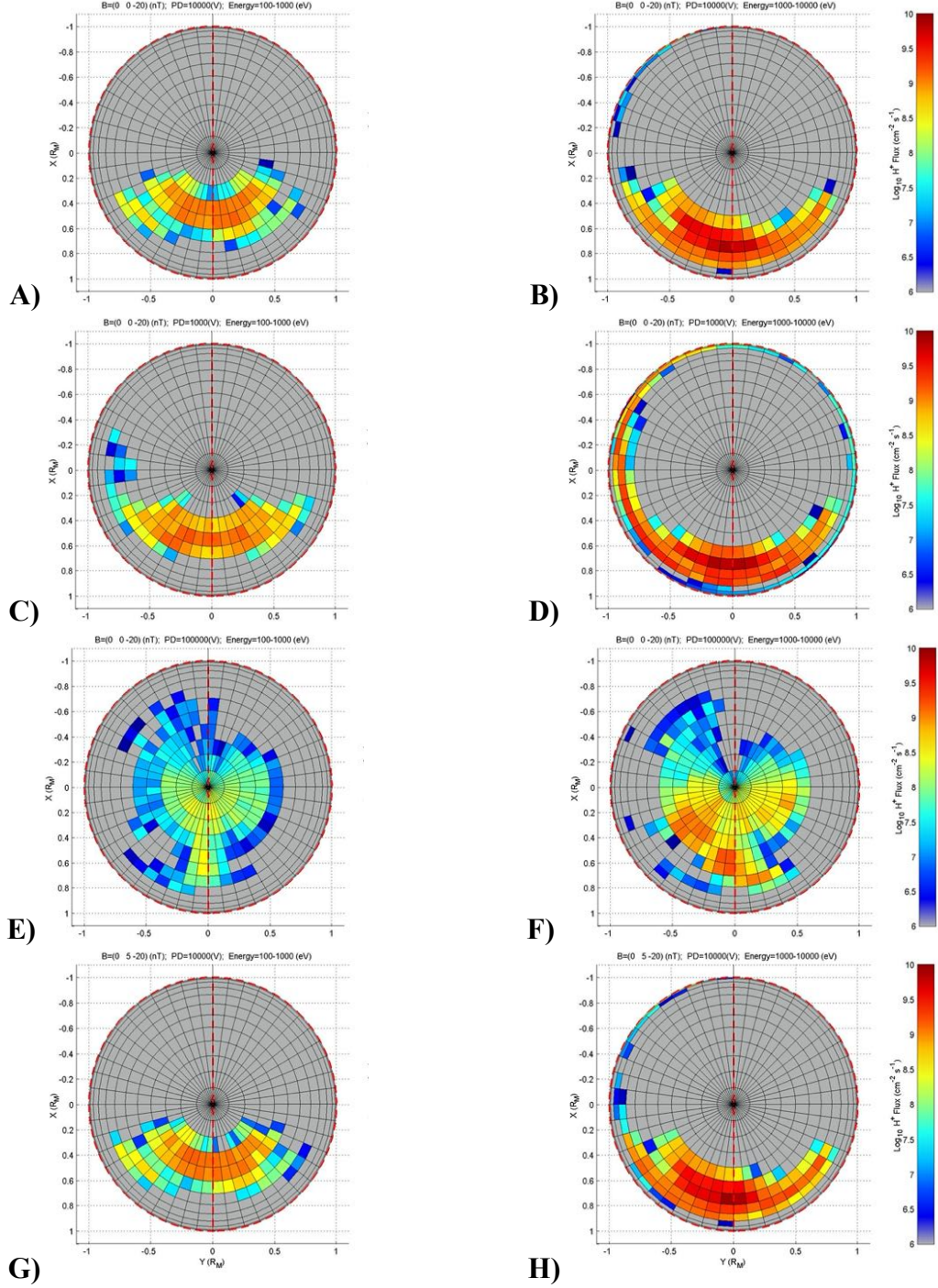
Figure 5.9 Colour-coded maps of H^+ flux over Mercury's surface. Panels A, C, E, G : low proton energy (100 eV – 1 keV); Panels B, D, F, H : high proton energy (1-10 keV). Panels A, B : reference condition. Panels C, D : same as A, B , but low potential drop ( PD=1 kV). Panels E, F : same as A, B , but high potential drop ( PD=100 kV). Panels G, H : same as A, B , but different IMF ( B_y = -5 nT).
