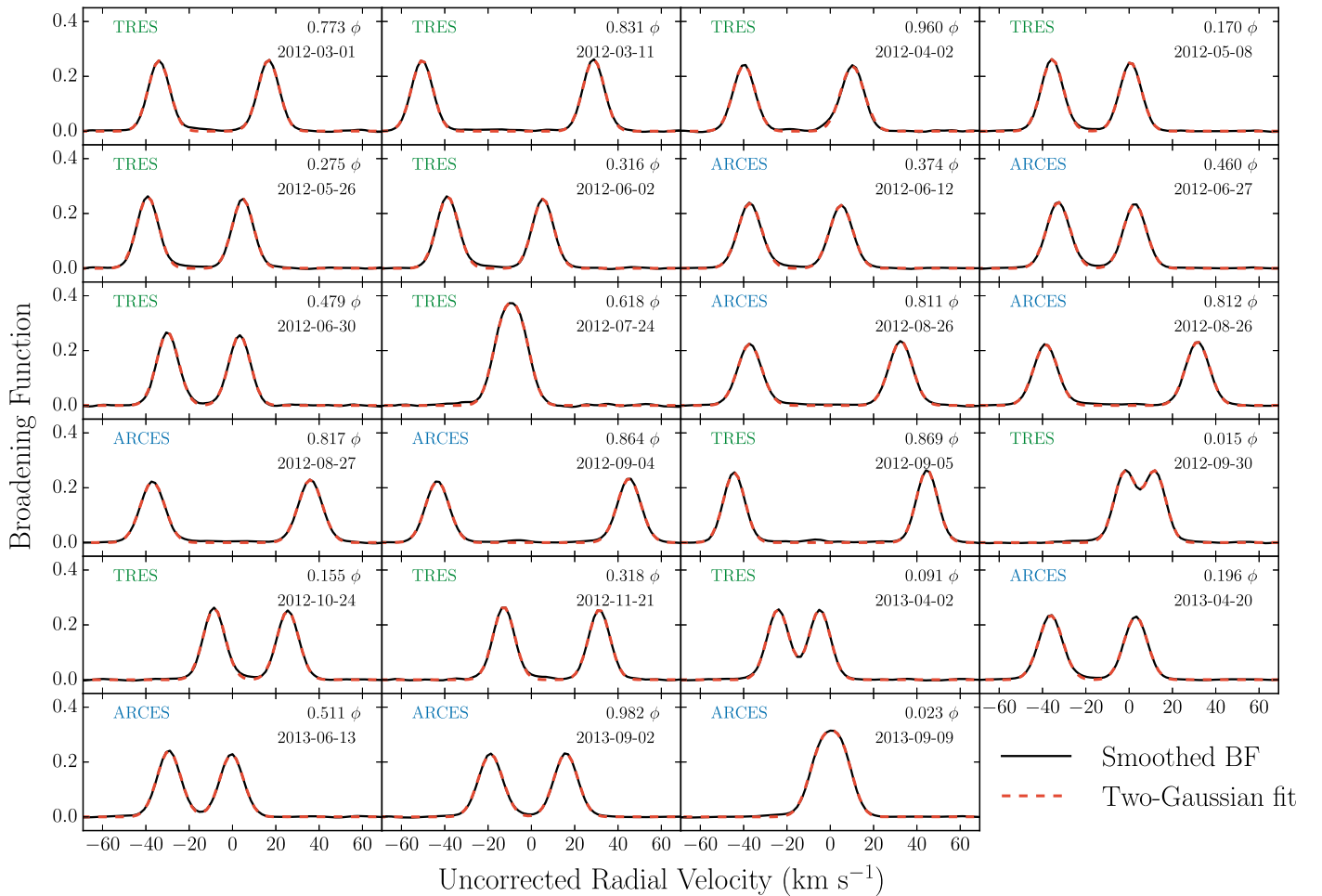
Figure 3. Radial velocities extracted for 23 ARCES and TRES observations of KIC 9246715 with the broadening function (BF) technique. Each panel represents one spectral observation, ordered chronologically, for which the BF convolution of the target star with a template PHOENIX model spectrum is shown in black. To identify the location of each BF in radial velocity space, we fit a pair of Gaussians, which are plotted in red. The date of observation, orbital phase, and instrument used are printed in the upper corners of each panel. Barycentric corrections have not yet been applied to these velocities.
