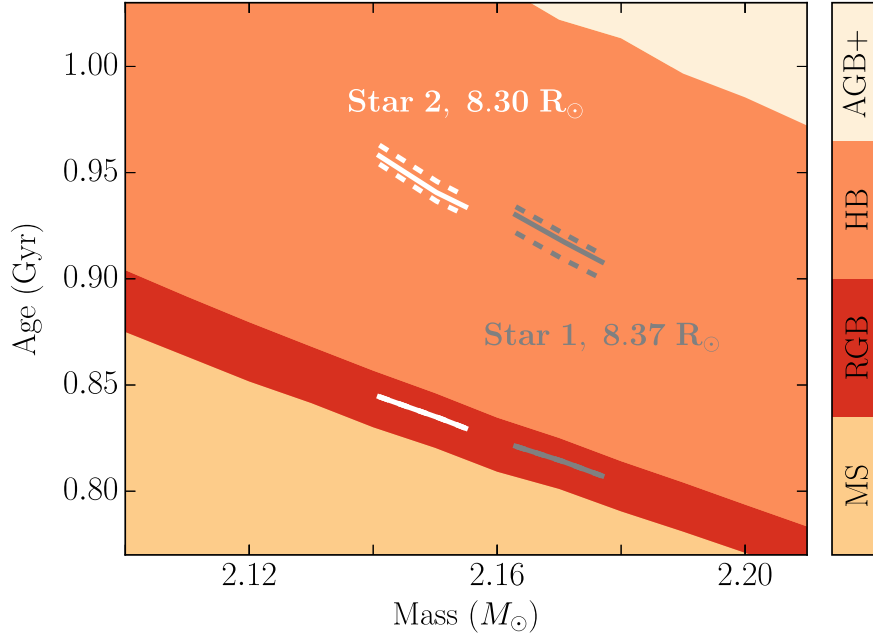
Figure 11. Ages for a suite of MESA stellar evolution models for stars of different masses. Color indicates the evolutionary state of a star as it moves from the Main Sequence (MS) → Red Giant Branch (RGB) → Secondary Red Clump/Horizontal Branch (HB) → Asymptotic Giant Branch and beyond (AGB+). Lines of constant radius equal to R_1 and R_2 that fall within the one-sigma errors in mass are shown (gray, R_1 \pm \sigma_{R_1} corresponding to M_1 \pm \sigma_{M_1} ; white, R_2 \pm \sigma_{R_2} corresponding to M_2 \pm \sigma_{M_2} ). All models assume a mixing-length parameter of \alpha = 2.5 . It is possible for both stars in KIC 9246715 to be the same age on the HB, but not on the RGB.
