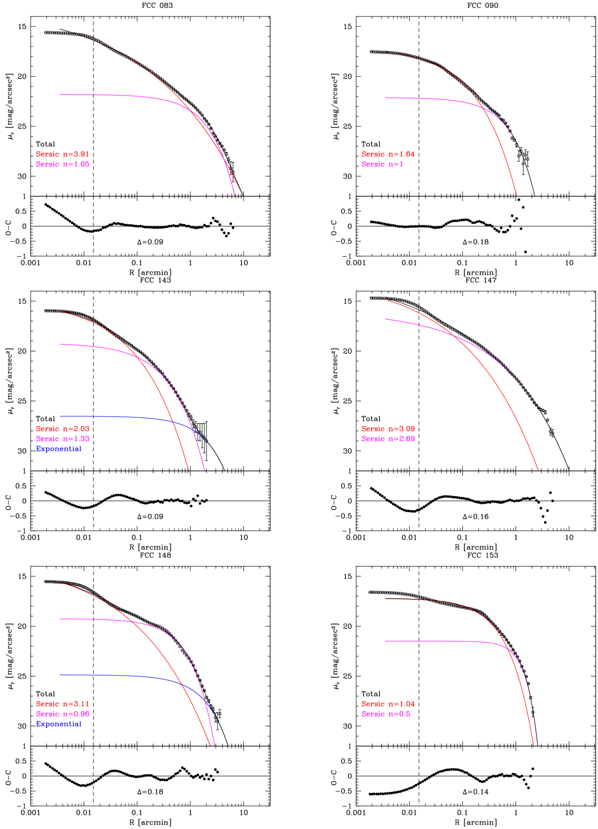
Fig. A.1. Top panels: deconvolved VST r-band profiles of ETGs in FDS plotted on a logarithmic scale. The blue line indicates a fit to the outer regions. The red and magenta lines indicate a fit to the inner and middle regions with a Sérsic profile, and the black line indicates the sum of the components from each fit. The dotted line indicates the core of the galaxy, which was excluded in the fit. Bottom panels: \Delta rms scatter (see text for details).
