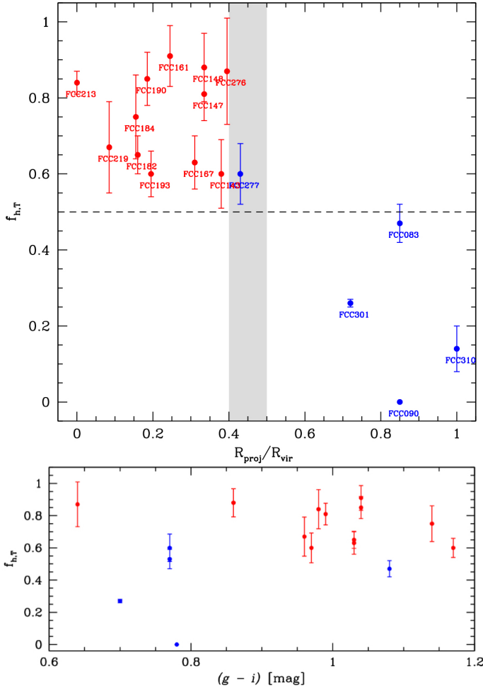
Fig. 5. Top panel: accreted mass fraction as a function of the projected distance from the cluster centre, normalised to the virial radius of the cluster ( R_{\text{vir}} = 0.7 Mpc, Drinkwater et al. 2001). Red dots indicate galaxies in the high-density region of the cluster, while blue dots indicate galaxies in the low-density region. The vertical grey region shows the range of cluster-centric distance where a clear separation occurs: galaxies located inside \sim 0.8 – 1 degree from the core of the cluster show a higher outer envelope mass fraction. Bottom panel: accreted mass fraction as a function of the (g-i) average colour for galaxies in the low- (blue dots) and high- (red dots) density regions of the cluster. On average, redder galaxies have higher accreted mass fractions. FCC 277 is in the transition region from high-to-low density; this region has a higher accreted mass fraction, but has colours comparable with galaxies in the low-density region.
