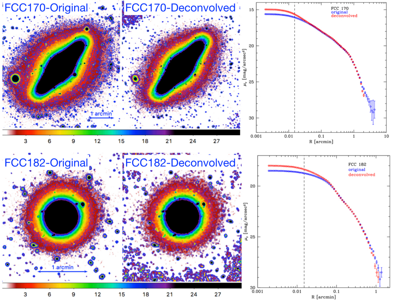
Fig. 2. Top panel: original (left) and deconvolved (middle) images of the flattest galaxy in our sample, FCC170. The original (blue) and deconvolved (red) surface brightness profiles of FCC170 are plotted in the right panel. Bottom panel: original (left) and deconvolved (middle) images of the smallest galaxy in our sample, FCC182. The original (blue) and deconvolved (red) surface brightness profiles of FCC182 are plotted in the right panel.
