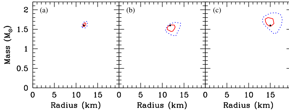
FIG. 5. Constraints on M and R obtained by fitting a waveform model to synthetic observed waveform data. Miller and Lamb, 2015 The black squares indicate the mass and radius used to construct the synthetic data, the solid red lines show the 1\sigma constraints, and the dashed blue lines show the 2\sigma constraints. Here the spin rate f_s = 600 Hz, hotspot inclination \alpha , and observer inclination i are 90^\circ , the fractional rms amplitude of the oscillations is 10.8%, and the total number of counts is 10^7 . M and R are tightly constrained: \Delta M/M = 2.8\% and \Delta R/R = 2.9\% . The parameter values used to generate the waveform data used in (b) are the same as in (a), except the rotation rate, which is much lower (300 Hz), causing the constraints on M and R to be weaker: \Delta M/M = 5.6\% and \Delta R/R = 7.6\% . (c) When the spot is at an intermediate colatitude (here 60^\circ ), the constraints on M and R are weaker ( \Delta M/M = 6.5\% and \Delta R/R = 6.7\% ), even if the star has a large radius (here 15 km) and is rapidly rotating (here at 600 Hz). From Miller and Lamb, 2015 .
