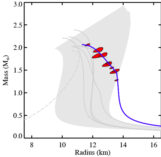
FIG. 6. 1\sigma confidence regions illustrating the constraints on the EOS that would be expected from a \sim 10\text{ m}^2 hard x-ray timing telescope. For illustration, the regions are assumed to trace the M - R curve of a proposed EOS that produces a neutron star with a strange matter core. The larger regions assume observing time has been dedicated to reach \mathcal{R} \approx 400 for the 50% of known burst oscillation systems (here 10) that have optimal spot and observer inclinations ( i = 60^\circ – 90^\circ ) if their orientations are randomly distributed. The size and shape of these regions are from the Bayesian analyses of waveform data by Lo et al. (2013) and Miller and Lamb (2015) that assume the hotspots and observers are in the equatorial plane and that there is no independent knowledge of any of the model waveform parameters. The smaller 1\sigma confidence regions show the constraints that could be achieved by a deep follow-up to halve the fractional uncertainties in M and R for the 3–4 stars that are most constraining, in terms of their locations in the M - R plane, the potential for reducing their uncertainties, and the availability of complementary constraints from other observations. Constraints like those shown will exclude many of the EOS models. In this illustration, the models shown as gray lines are excluded.
