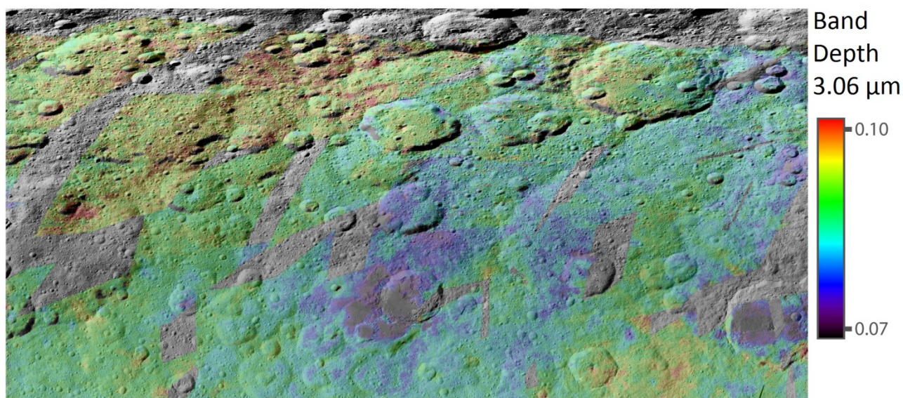
Figure 4. The band depth at 3.1 \mu\text{m} is indicative of the NH 4 -phyllosilicates abundance.
