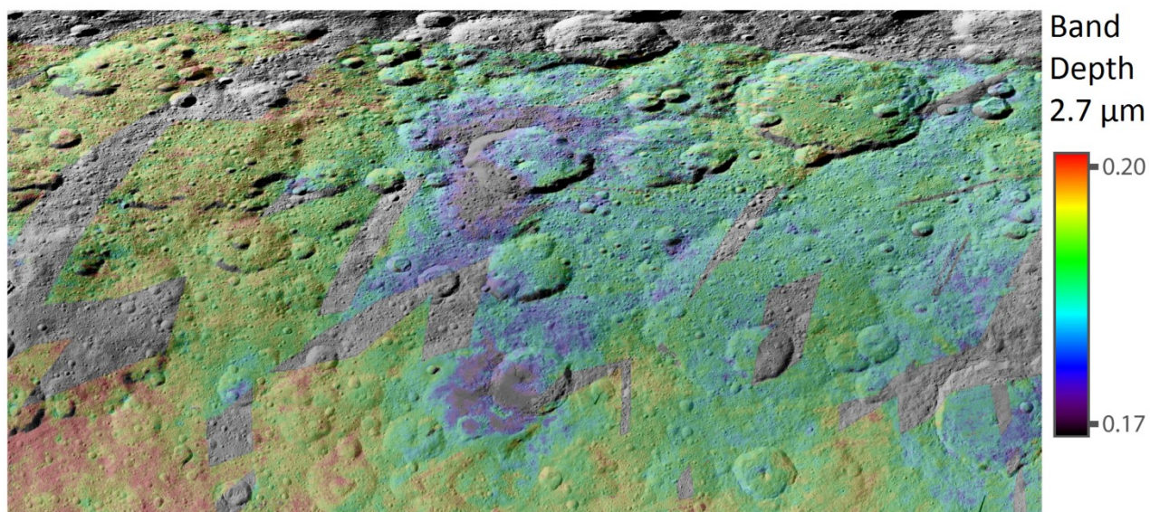
Figure 3. The band depth at 2.7 \mu\text{m} shows the abundance of Mg-phyllosilicates.
