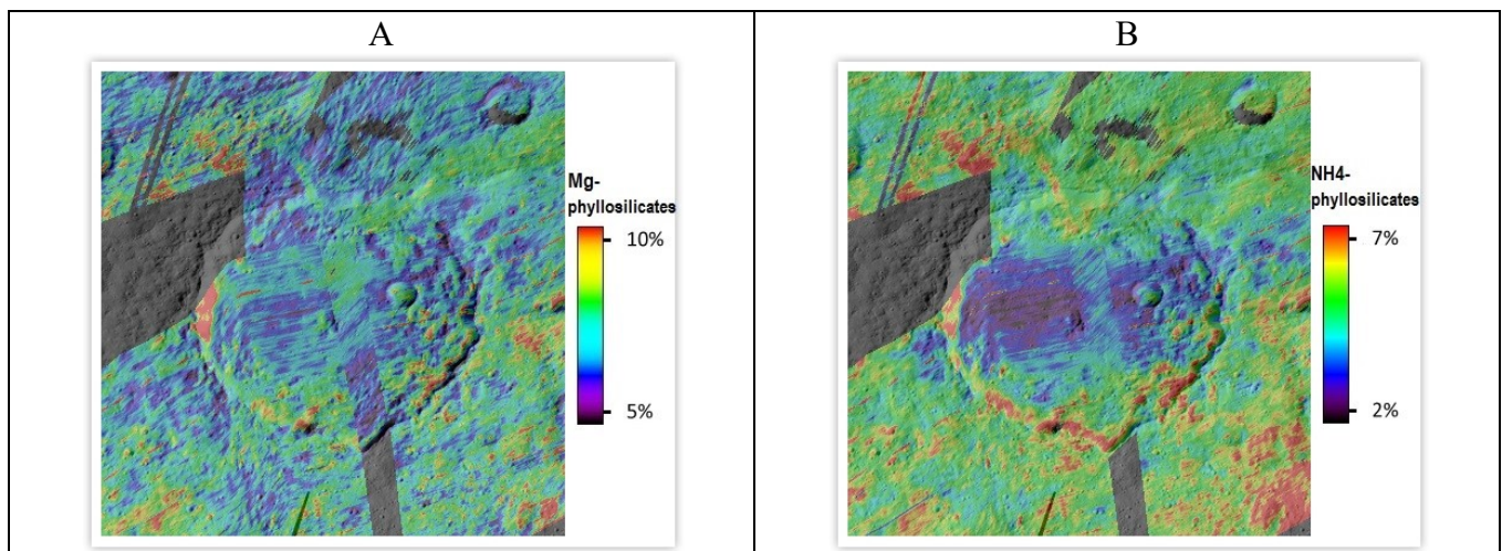
395 Figure 12. Gaue crater. Mg-phyllsilicates and NH 4 -phyllsilicate abundances. Other parameters are not shown 396 because they do not present significant differences with respect the average surface. 397 398
