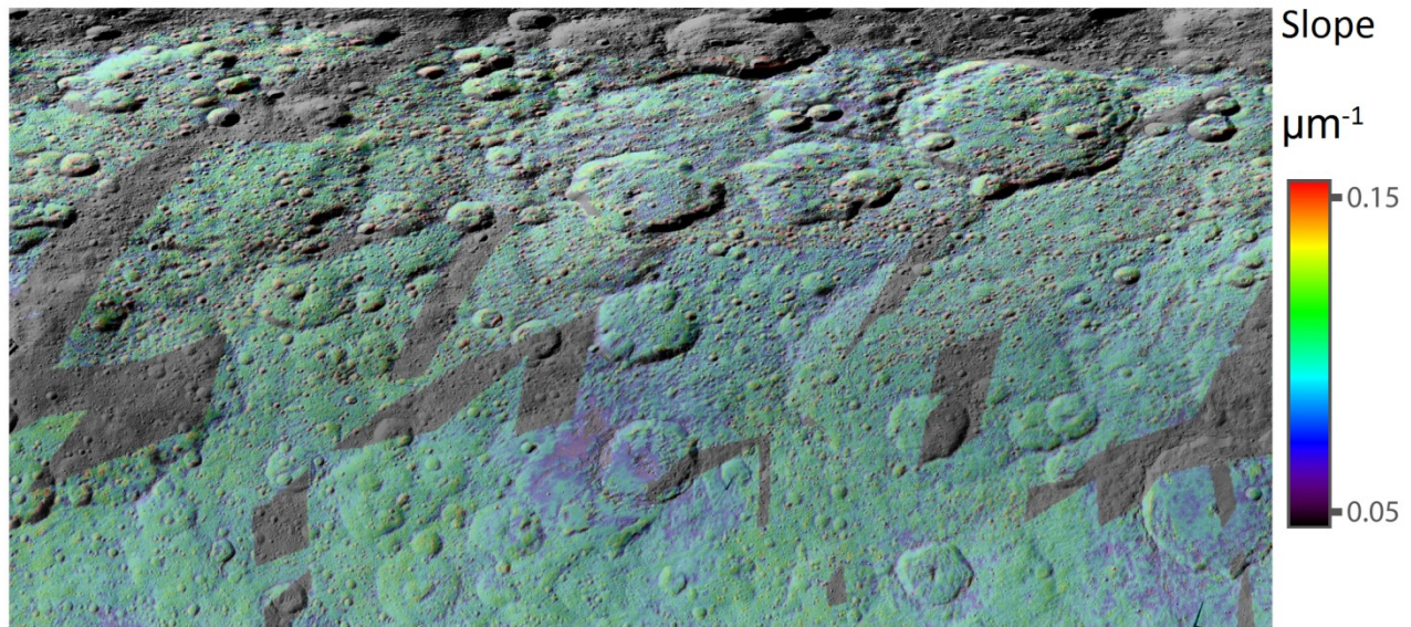
Figure 7. Coniraya 1.891-1.163 \mu\text{m} spectral slope map. To calculate the spectral slope, we use the definition used by Cuzzi et al. (2009), and Filacchione et al. (2012): \text{Slope} = (R_{\lambda_2} - R_{\lambda_1}) / (\lambda_2 - \lambda_1) / R_{\lambda_1} , where \lambda_1 = 1.163 \mu\text{m} , \lambda_2 = 1.891 \mu\text{m} , and R_{\lambda} is the reflectance at \lambda .
