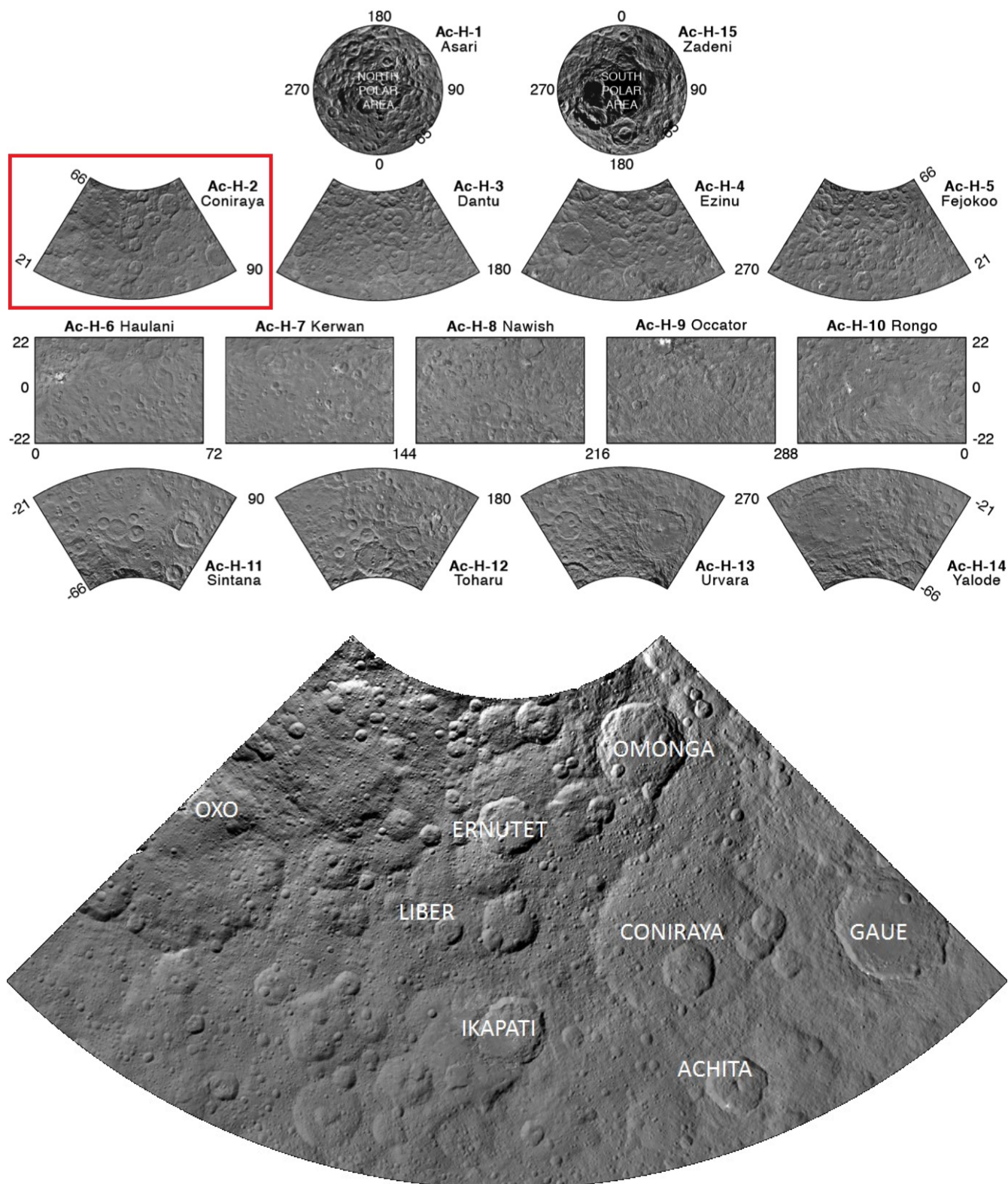
Figure 1. Upper panel: figure adapted from Roatsch et al. (2016), showing the 15-quadrangle scheme in which Ceres' surface has been divided. The Coniraya quadrangle, highlighted in red, is the main focus of this study and is located at 0° - 90°, 21° - 66° N. Bottom: Dawn Framing Camera clear filter LAMO base map mosaic in the Lambert Conical projection, with 35 m/pixel resolution. The names of the main craters are indicated.
