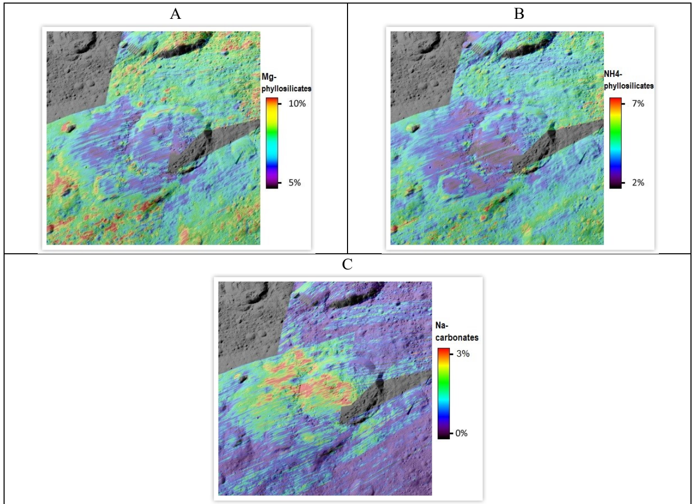
391 Figure 11. Distributions of the abundances of the modeled endmembers of the Ikapati crater. Panel A: Mg- 392 phyllsilicates, panel B: NH 4 -phyllsilicate, panel C: Na-carbonates. Other end-members abundances are not 393 shown because they do not present significant differences with respect the average surface. 394
