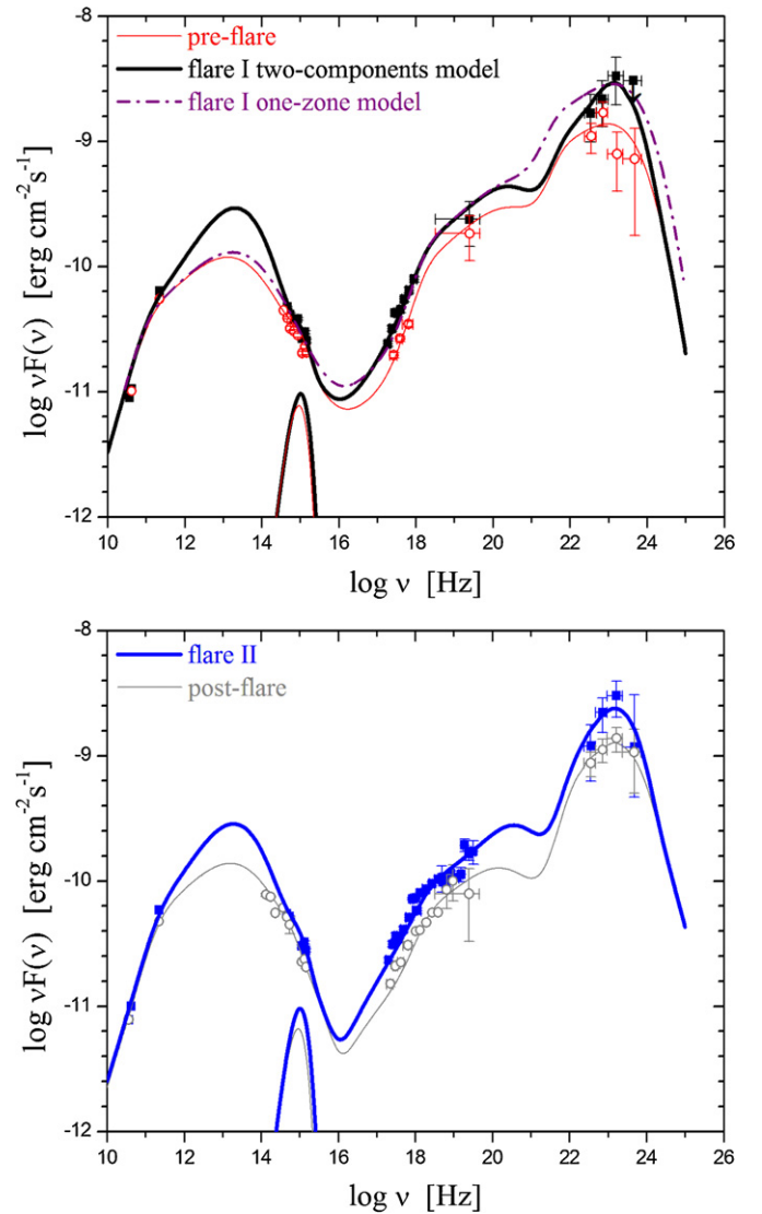
Figure 2. Multifrequency simultaneous spectra of 3C 454.3 at four different epochs superimposed with spectral modeling. Top panel: pre-flare (red open circles) and super-flare (black filled squares). Bottom panel: secondary flare (blue filled squares) and post-flare spectra (gray open circles). Models are detailed in the text.
