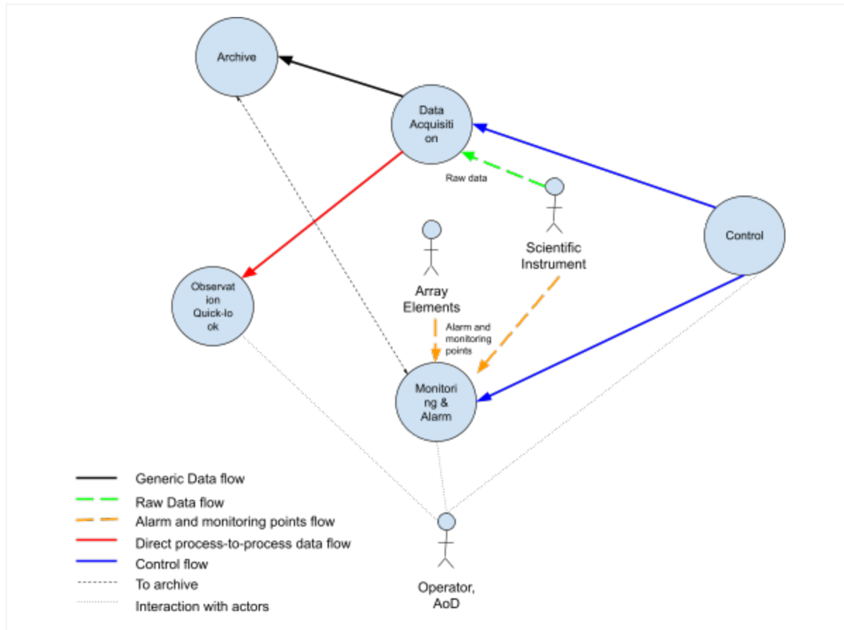
Figure 24: MA Software System data and information flow (schematic) for the Observation Execution phase . Details on the array control and data acquisition flow. The black dashed lines directed to/from the Archive indicate that a) all data is saved and can be retrieved from the Archive, and b) that the physical data flow may be handled by the Archive.
