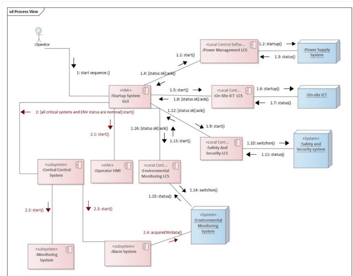
Figure 28: The Startup System sequence of operations. In the figure is shown also the subsystem started by the Central Control System.
