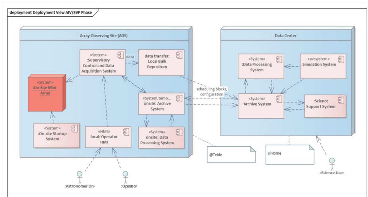
Figure 54: Deployment View in AIV/SVP phase.
