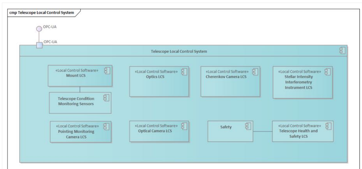
Figure 14: Telescope Local Control System's main Local Control Software.
