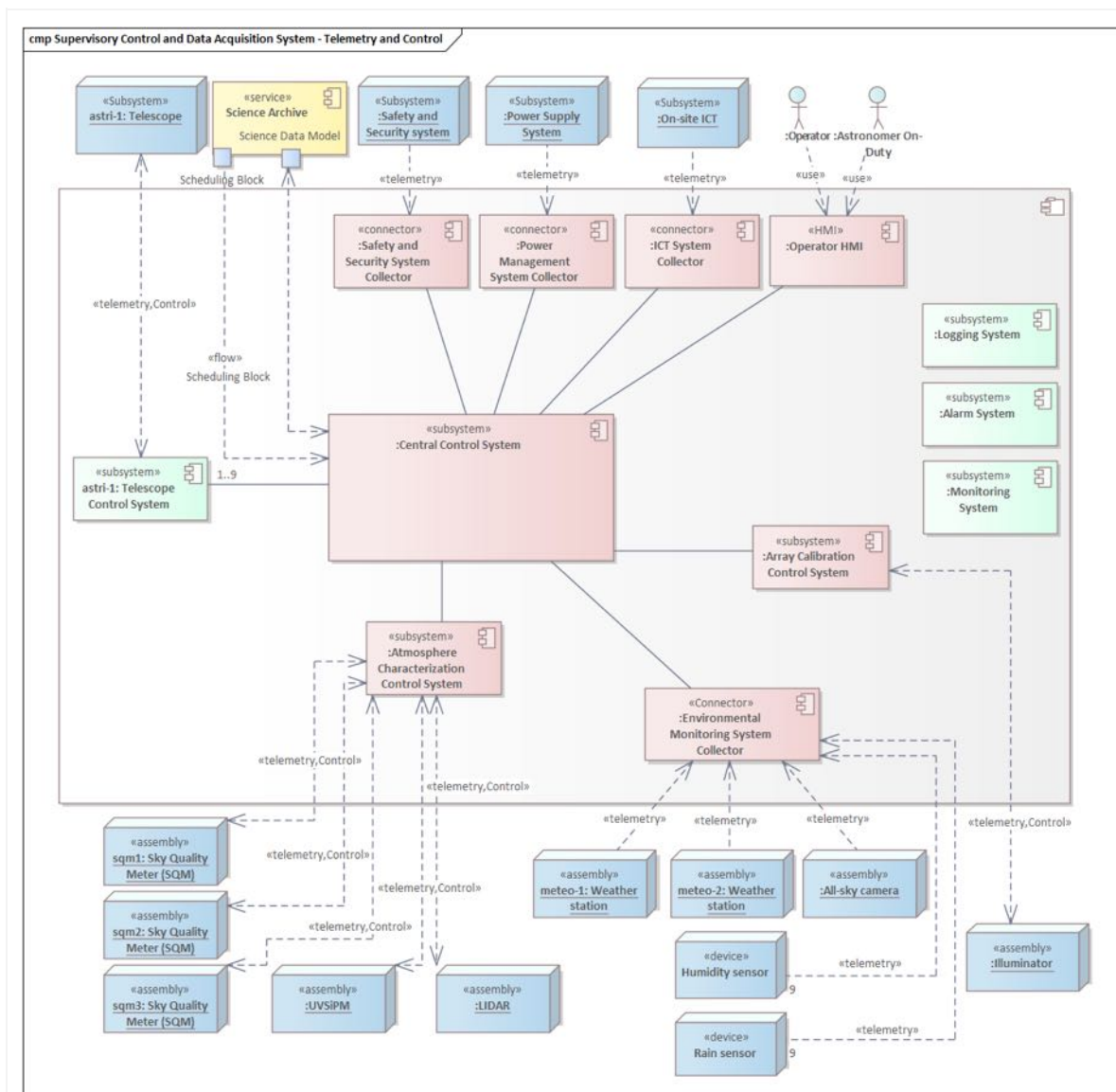
Figure 35: Telemetry and control flow. Logging system acquires logs from all events. Monitoring system acquires monitoring points from all assemblies. Alarm system receives alarms from assemblies. Only one telescope (and related subsystems) is shown. Not all connections are shown, in particular the interconnections between Control Software/Collectors and Central Control System are not shown. The SCDB is not shown.
