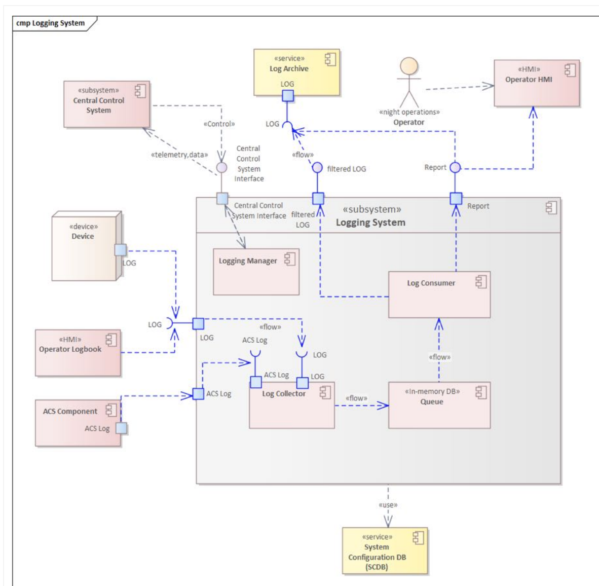
Figure 41: The Logging System. The Logging Manager coordinates the workflow.
