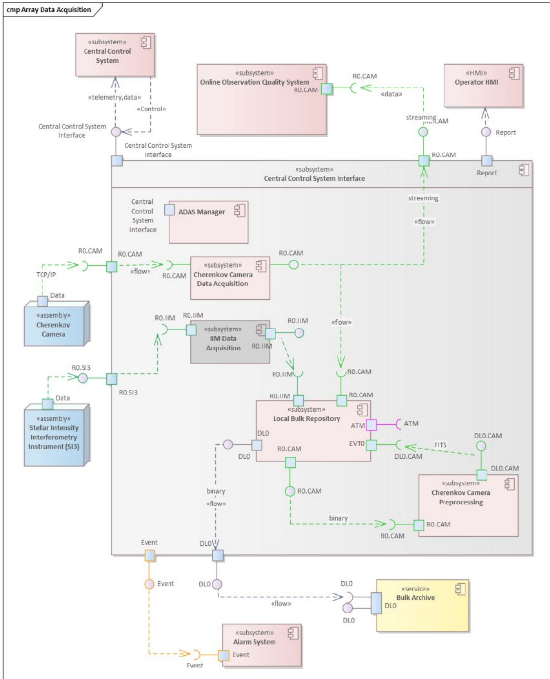
Figure 39: Array Data Acquisition system. Reports about the status of the acquisition are sent to the Operator HMI at the end of a Run. Each component can generate an event to the Alarm System and for this reason these connections are not shown.
