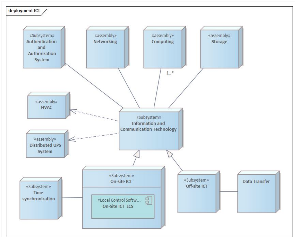
Figure 20: ICT System
