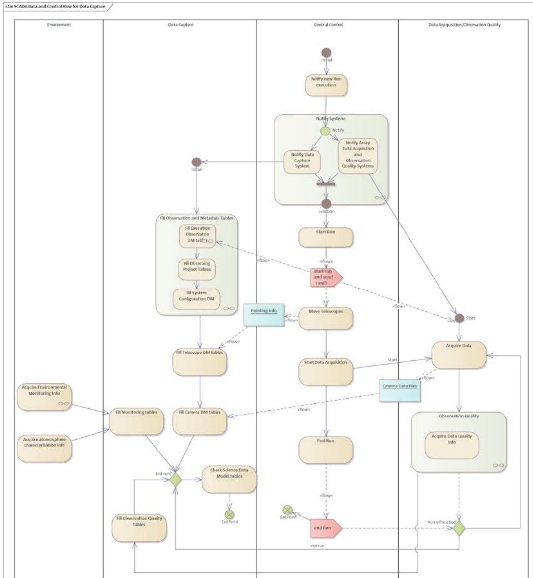
Figure 38: SCADA data flow and control flow for Data Capture, for the definition of the Science Data Model.
