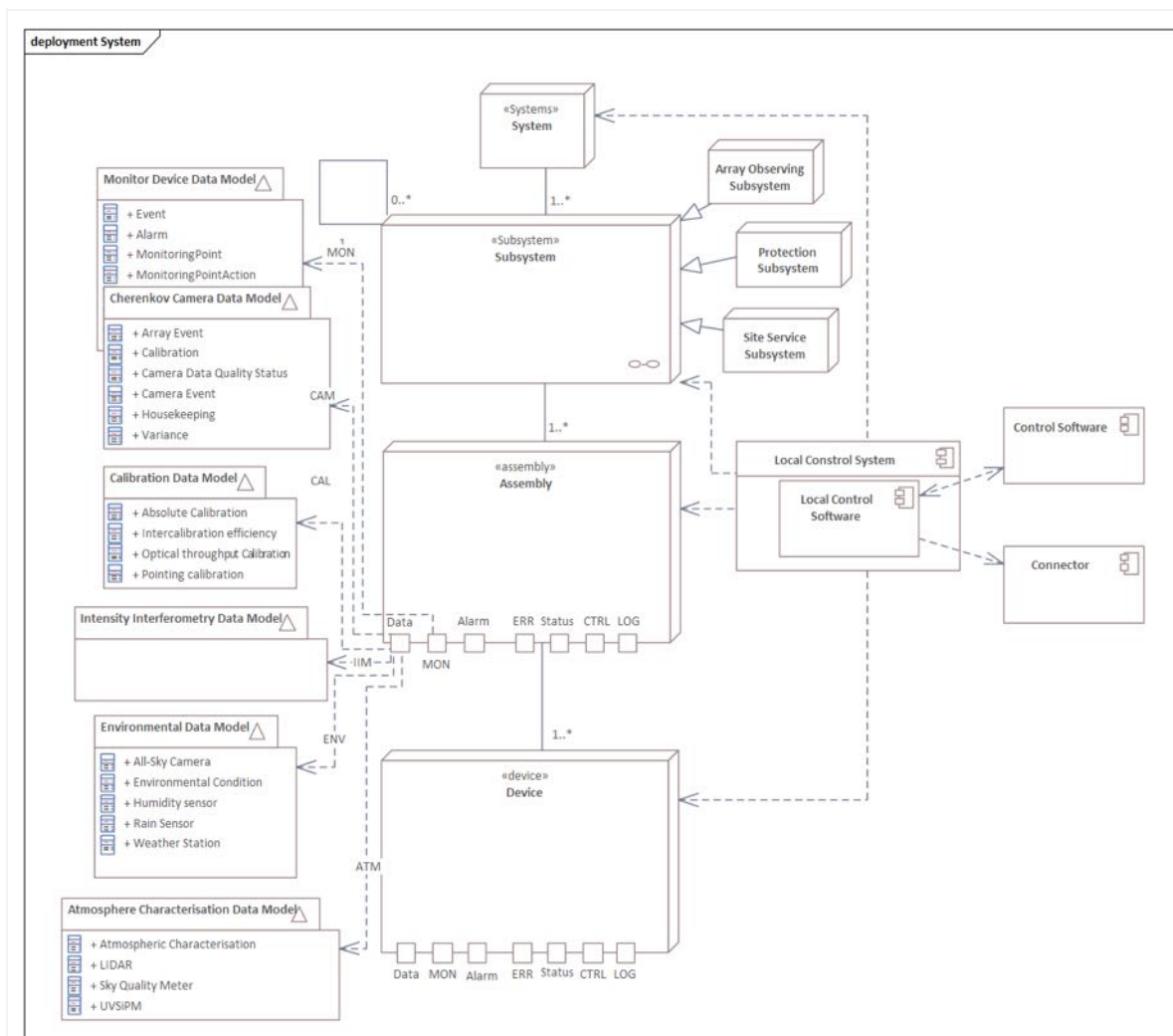
Figure 5: Systems, subsystems, assemblies, devices nodes, with Local Control Systems and Local Control Software and their relationships with some data models (see [AD2]) with their abbreviation used in the diagrams of this document. A Local Control Software has an server-side OPC-UA interface and is outside the SCADA system (see Sect. 5.2.).
