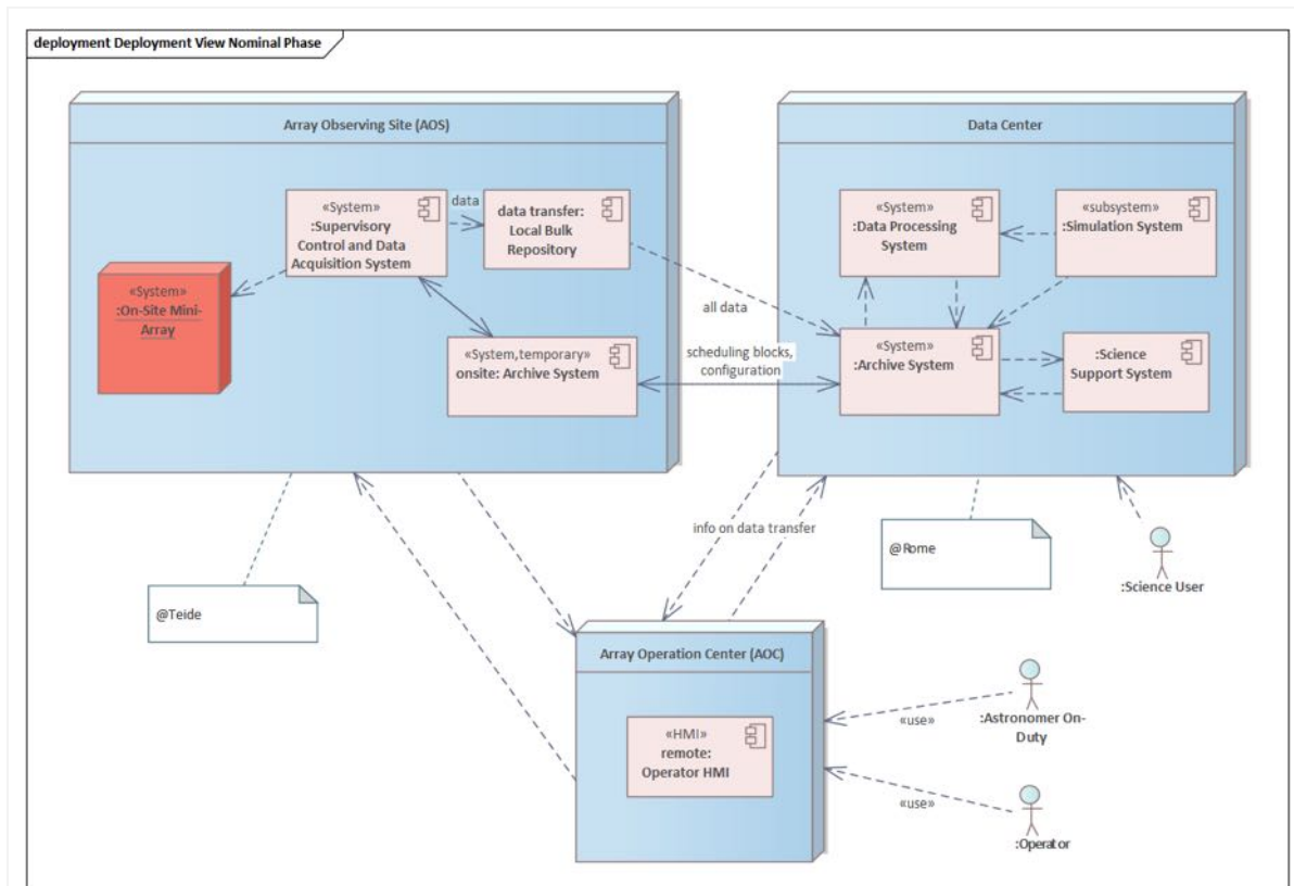
Figure 53: Deployment View in nominal phase.
