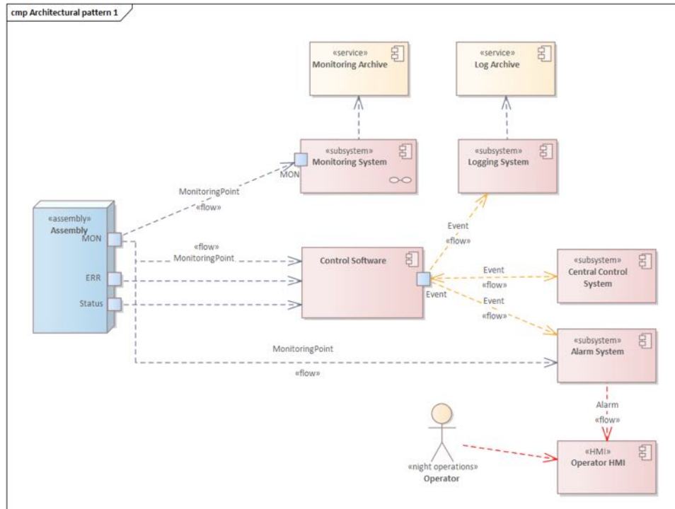
Figure 32: Pattern #1: identification of an assembly event with a control software/collector. The Figure shows only a Control Software, but a Connector can be present instead of the Control Software. If a Control Software/Collector is not present, this responsibility is given to the Monitoring System .
