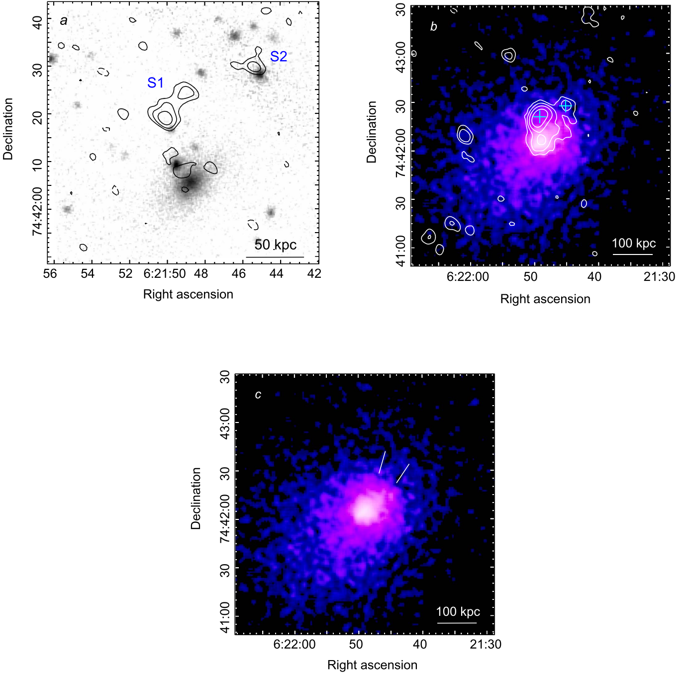
Figure 8. PSZ1 G139.61+24.20. (a) GMRT 1.28 GHz contours at a resolution of 3'' \times 2'' in PA 53^\circ , overlaid on the r -band Pan-STARRS1 optical image. The rms noise of the radio image is 1\sigma = 15 \mu\text{Jy beam}^{-1} . Contours are scaled by a factor of 2, starting from 0.05 \text{ mJy beam}^{-1} . Contours at -0.05 \text{ mJy beam}^{-1} are shown as dashed. Here S1 is an extended radio source with no optical identification on the POSS-II image, and S2 is a radio source with an optical counterpart. (b) Contours from the combined image at 610 MHz, restored with a 7'' circular beam, overlaid on a Chandra smoothed X-ray image in the 0.5–4 keV band. The rms noise of the radio image is 1\sigma = 30 \mu\text{Jy beam}^{-1} . Contours are scaled by a factor of 2, starting from 0.08 \text{ mJy beam}^{-1} . Crosses mark the positions of the radio galaxies S1 and S2 (panel (a)). (c) Chandra X-ray image, same as panel (b). White lines mark the position of an X-ray cold front (Savini et al. 2018).
