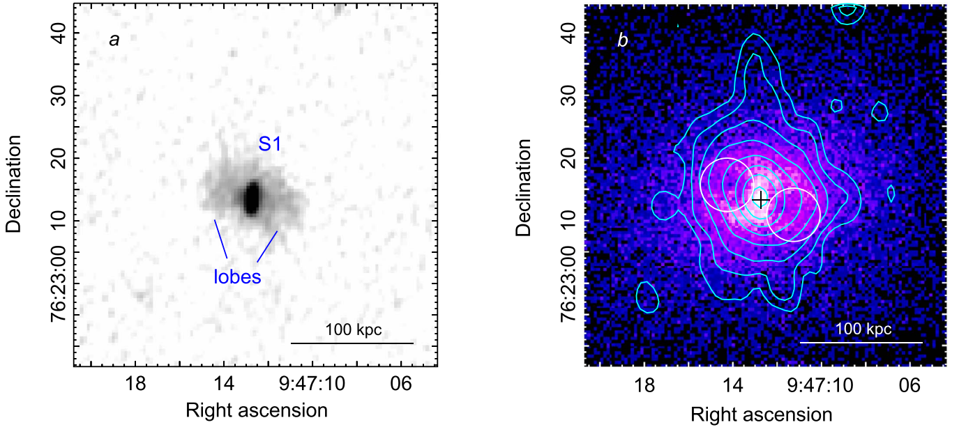
Figure 13. RBS 797. (a) VLA 1.4 GHz A-configuration image, restored with a 2'' \times 1'' beam. The rms noise is 1\sigma = 17 \mu\text{Jy beam}^{-1} . The central radio galaxy S1 and the radio lobes filling the X-ray cavities (white circles in panel (b)) are labeled. (b) VLA 1.4 GHz B-configuration contours overlaid on the Chandra image in the 0.5\text{--}4 \text{ keV} band. The radio image has a restoring beam of 5'' \times 4'' . The rms noise is 1\sigma = 27 \mu\text{Jy beam}^{-1} . Contours start at 70 \mu\text{Jy beam}^{-1} and then scale by a factor of 2. No levels at -3\sigma are present in the portion of the image shown. Circles mark the X-ray cavities filled by the radio lobes (panel (a)).
