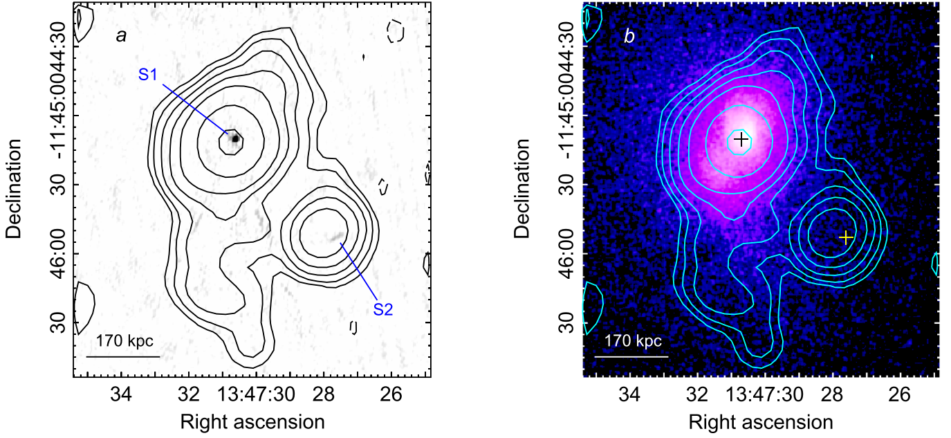
Figure 14. RX J1347.5–1145. (a) VLA 1.4 GHz C-configuration contours, overlaid on the 1.4 GHz A-configuration image. The restoring beam and rms noise are 17'' and 1\sigma = 40 \mu\text{Jy beam}^{-1} and 1''/2 and 1\sigma = 35 \mu\text{Jy beam}^{-1} , respectively. Contours are -0.12 (dashed), 0.12 , 0.24 , 0.48 , 0.96 , 2 , 8 , 32 , and 128 \text{ mJy beam}^{-1} . Individual radio galaxies are labeled. (b) VLA 1.4 GHz C-configuration contours of the minihalo and radio galaxies (black and yellow crosses; see panel (a)), overlaid on the Chandra image in the 0.5\text{--}4 \text{ keV} band.
