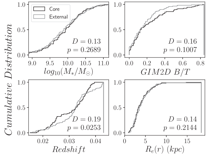
Figure 5. Cumulative distributions of stellar mass, B/T , redshift, and effective radius for core (black) and external galaxies (gray). The K-S D and p -value are shown in each panel. The samples are comparable except in terms of redshift, with the external sample offset to slightly higher values. This difference does not affect our results.
