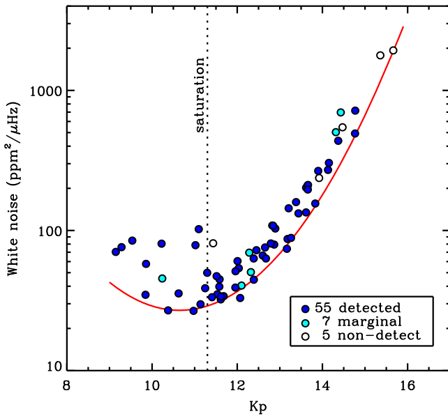
Figure 4. Noise level in power spectra as function of Kp magnitude for all stars with APOGEE T_{\text{eff}} < 5000 K and APOGEE \log g in the range 2.1–3.35 (see Figure 3(a)). The noise is measured as the median power in the range 260–280 \mu\text{Hz} . For reference we show a fiducial line described by \log(\text{WhiteNoise}) = 9.77 - 1.57Kp + 0.074Kp^2 \text{ppm}^2/\mu\text{Hz} that follows the lower envelope of the magnitude-dependent noise floor (red curve). The saturation limit of K2 is indicated by the dotted line. The increased noise for saturated stars can be mitigated using larger aperture masks than in the VJ photometry used here (Lund et al. 2015).
