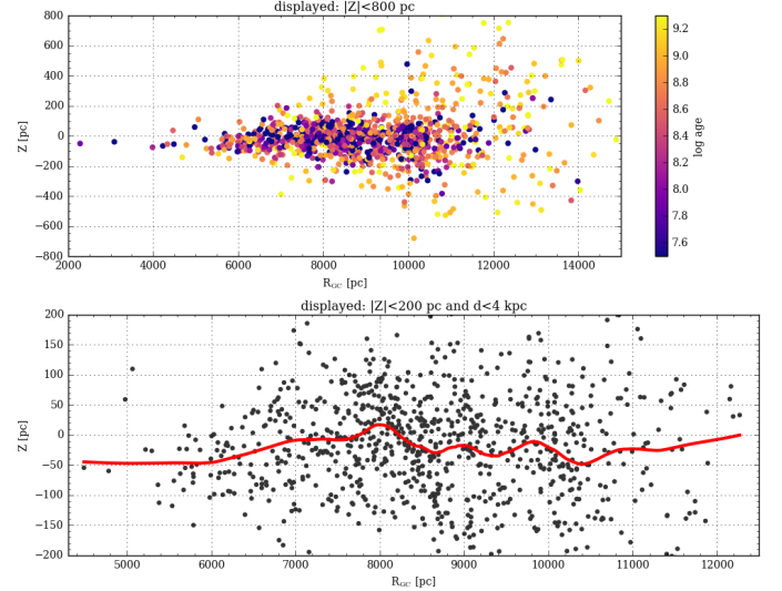
Fig. 12. Top: distance Z to the Galactic plane vs Galactocentric distance R_{GC} , colour-coded by age (as listed in MWSC). Bottom: Z vs R_{GC} for OCs within 4 kpc of the Sun. The red line is a lowess smoothing (local median based on the nearest 15% of points in the sample).
