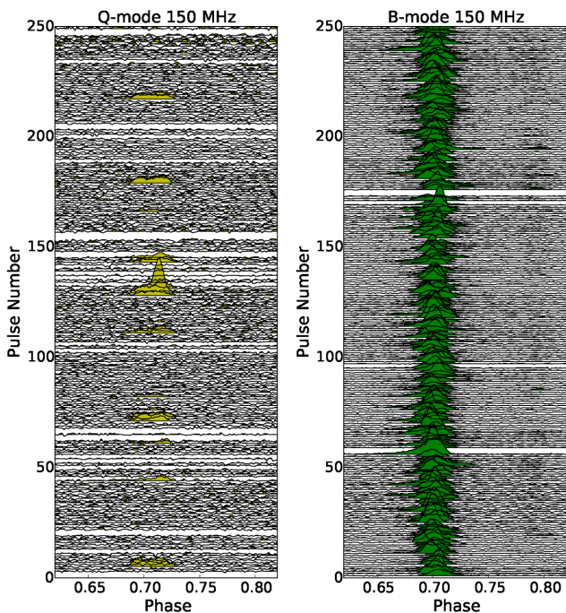
Figure 7. Representative examples of single-pulse profiles from the LOFAR observation on 2013 April 7, arbitrarily normalized. Left: sporadic and weak emission during the Q mode, right: B -mode regular emission for comparison. Single pulses rejected due to RFI are not shown.
