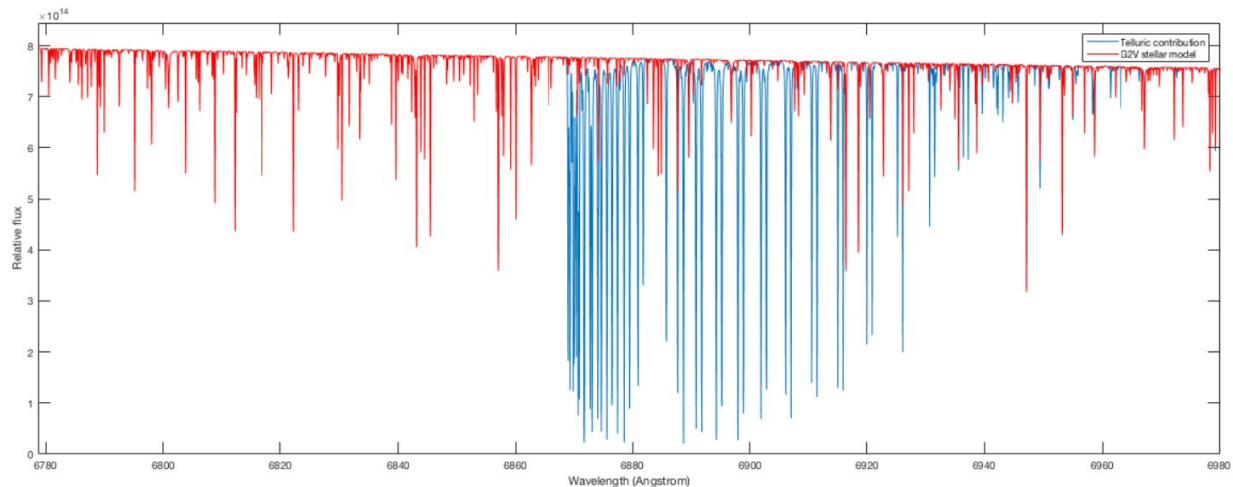
Figure 5. Example of part of simulated spectrum in output from the Atmospheric Module; in red a G2V stellar model and in blue the telluric spectrum. Both are computed at a resolution 3 times higher than the main observing mode resolution.
