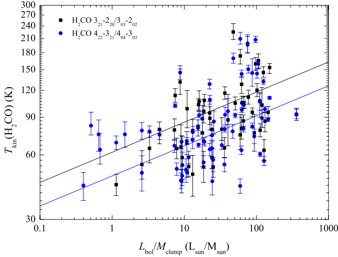
Fig. 12. Kinetic temperatures derived from para-H 2 CO (3 21 –2 20 /3 03 –2 02 and 4 22 –3 21 /4 04 –3 03 ), black squares and blue points) vs. luminosity-to-mass ratio L_{\text{bol}}/M_{\text{clump}} . The straight lines are the results from unweighted linear fits for clumps with L_{\text{bol}}/M_{\text{clump}} \geq 10 L_{\odot}/M_{\odot} .
