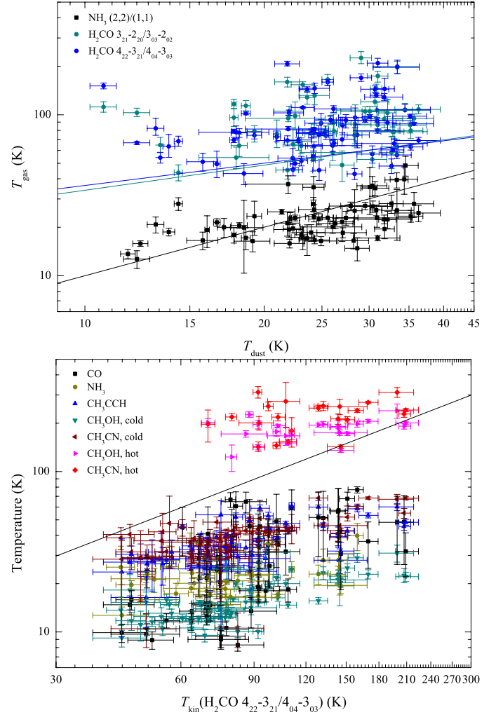
Fig. 8. Top panel: comparison of kinetic temperatures derived from para-H 2 CO (3 21 –2 20 /3 03 –2 02 and 4 22 –3 21 /4 04 –3 03 , cyan and blue points) and NH 3 (2,2)/(1,1) (black squares) ratios against the dust temperatures. NH 3 kinetic temperatures are selected from Wienen et al. (2012). The cyan and blue straight lines are the results from unweighted linear fits for gas temperatures derived from para-H 2 CO (3 21 –2 20 /3 03 –2 02 and 4 22 –3 21 /4 04 –3 03 , respectively). Bottom panel: comparisons of gas temperatures derived from para-H 2 CO (4 22 –3 21 /4 04 –3 03 ), CO, NH 3 (2,2)/(1,1), CH 3 OH, CH 3 CN, and CH 3 CCH. Temperatures of CO, CH 3 OH, CH 3 CN, and CH 3 CCH are taken from Giannetti et al. (2017). The black straight lines in both panels indicate equal temperatures.
