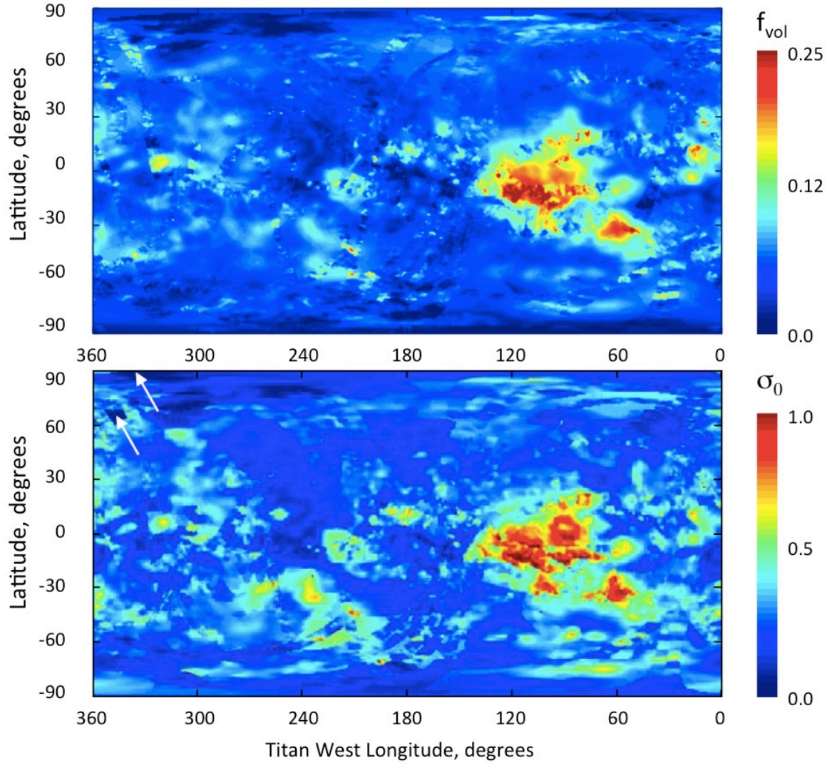
Figure 1. Predicted and observed maps of scattering from Titan's surface. The upper panel is a map of the volume scattering parameter f_{\text{vol}} for a simple surface model composed of a smooth dielectric interface separating free space from an inhomogeneous and isotropically scattering subsurface. f_{\text{vol}} is the probability that a photon entering the surface (as determined by the effective dielectric constant) scatters and escapes from the subsurface before it is absorbed. The map of f_{\text{vol}} reconciles the maps of effective dielectric constant and emissivity and predicts the overall magnitude of the scattering. The lower panel is a global mosaic of Titan's normalized radar cross-section from all real aperture data through T71 (Wye et al., 2011), showing the actually observed scattering. The white arrows in the upper left-hand corner indicate two small regions that were not mapped.
