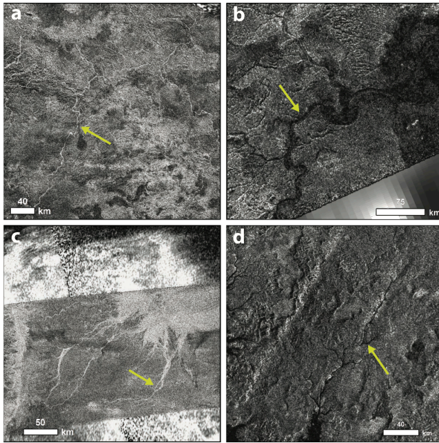
Figure 19. (a) Rectilinear networks in eastern Xanadu ; (b) Celadon Flumina, a meandering network near the south pole ; (c) Elvigar Flumina, a braided network that deposits into an alluvial fan ; (d) Vid Flumina, a dendritic canyon network up to 500 m deep that drains into Ligeia Mare .
