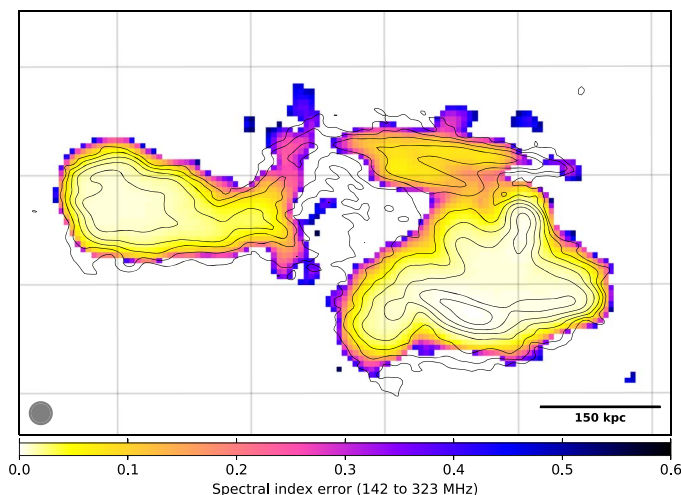
Fig. 4. Spectral index error map. Each pixel shows the standard deviation of the bootstrapped spectral index distribution.
