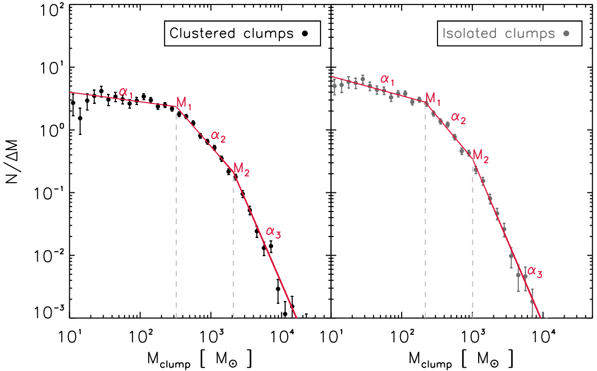
Fig. A.2. Mass distribution of clustered clumps ( left panel ) and isolated clumps ( right panel ) in the first quadrant. Only clumps with HDEs are used. The two plots correspond to the function \Phi (Eq. (7)) versus mass. The red lines correspond to the fitting segments of the CMF.
