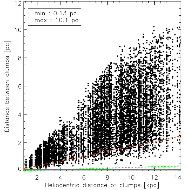
Fig. 16. Distribution of the distance between clustered clumps in cluster candidates. The green dashed line represents the linear diameter of the beam at 70\ \mu\text{m} . The orange dashed line corresponds to the same size, but at 500\ \mu\text{m} . The grey line marks the Jeans length (0.1 pc).
