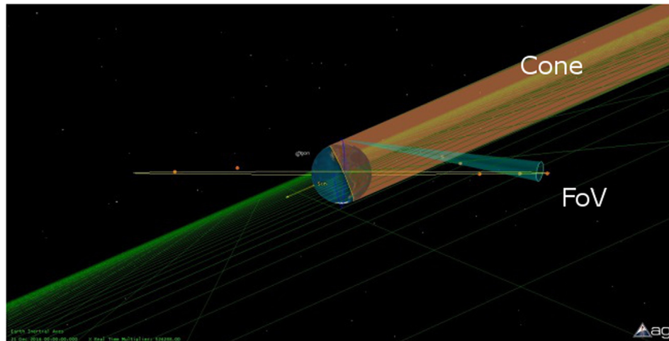
Fig. 9. December Solstice – Umbra and penumbra cones Vs FoV.
