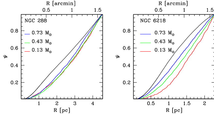
Figure 6. Comparison between the cumulative profile of dark mass (black lines) with those of stars in different mass bins in NGC 288 (left-hand panel) and NGC 6218 (right-hand panel). All profiles are normalized at a distance corresponding to the ACS field of view (1.6 arcmin).
