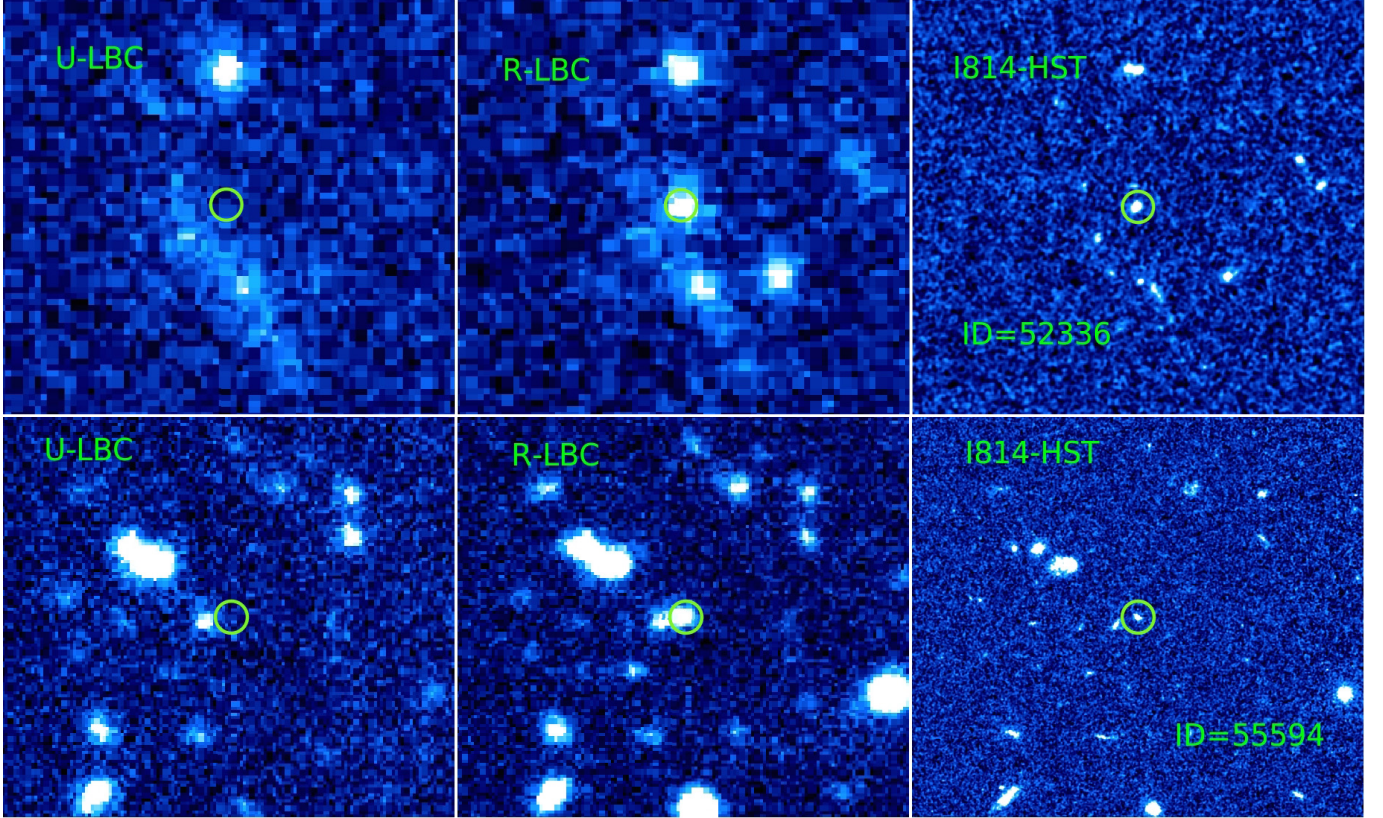
Fig. A.1. Cutouts of sources ID = 52336 and 55594 in the U -band ( left ) and in the R -band ( central panels ) by the LBC instrument. The right cutouts show the same sky area observed by HST in the I814W filter. The positions of the galaxies with spectroscopic redshifts z \sim 3.3 are indicated with green circles. The size of the cutouts is 12 arcsec for source ID = 52336 and 25 arcsec for ID = 55594, respectively.
