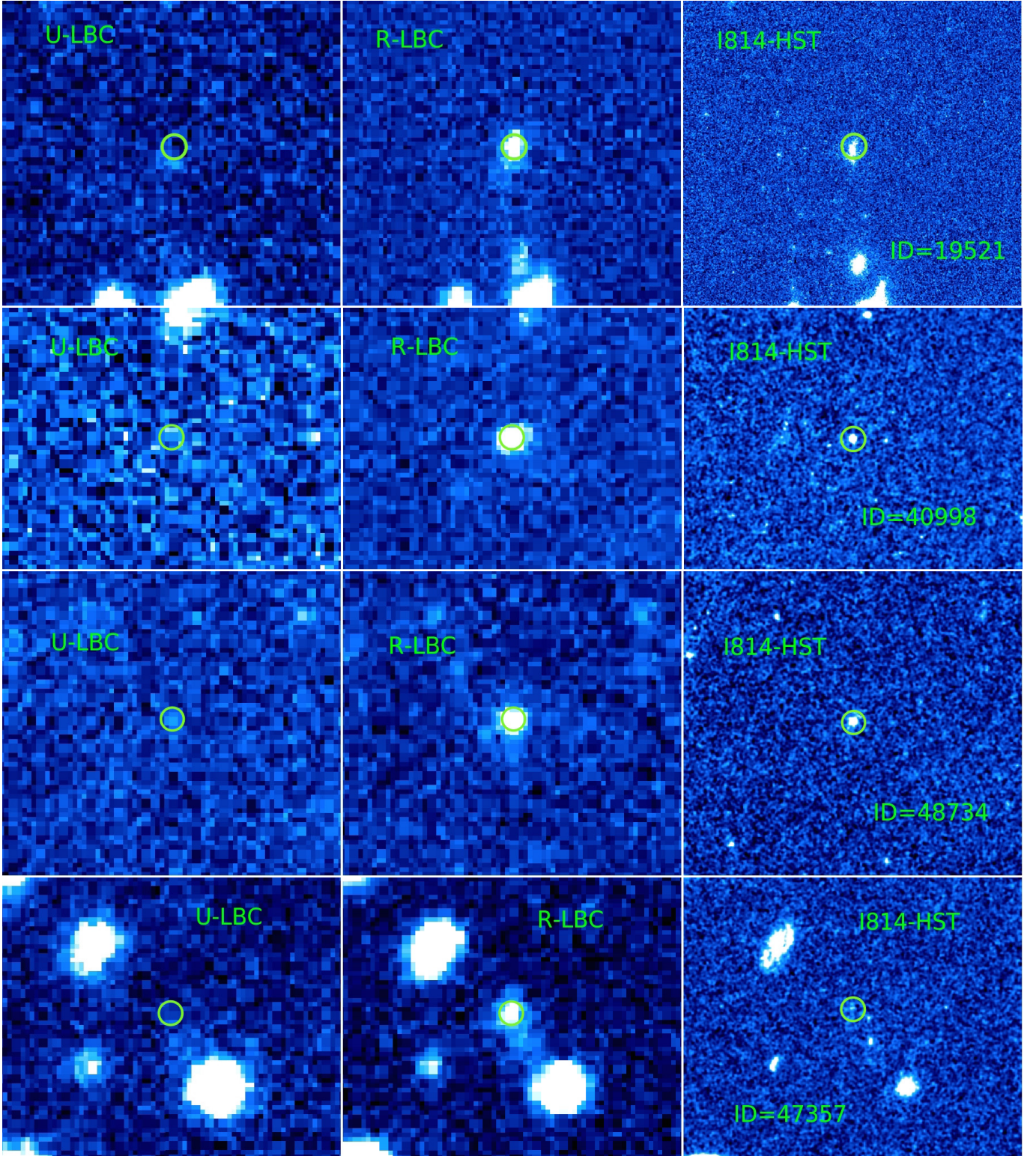
Fig. A.2. Cutouts of sources ID = 19521, 40998, 48734, and 47357 in the U -band ( left ) and in the R -band ( central panels ) by the LBC instrument. The right cutouts show the same sky area observed by HST in the I814W filter. The positions of the galaxies with spectroscopic redshifts z \sim 3.3 are indicated with green circles. The size of the cutouts is 15, 10, 12, and 10 arcsec for source ID = 19521, 40998, 48734, and 47357, respectively.
