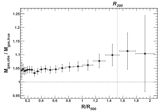
Figure 8. Bias in gas mass derived by comparing standard and clumping-corrected gas mass profiles (see equation 5).
