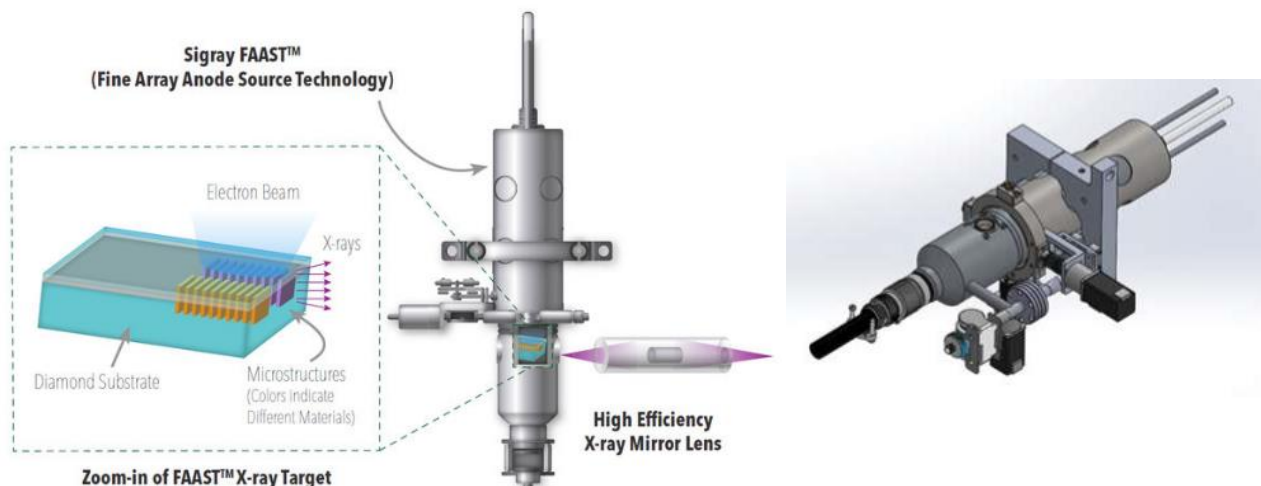
Figure 4-5: Pictorial image of the Sigray FAAST-Micro™ X-ray source
