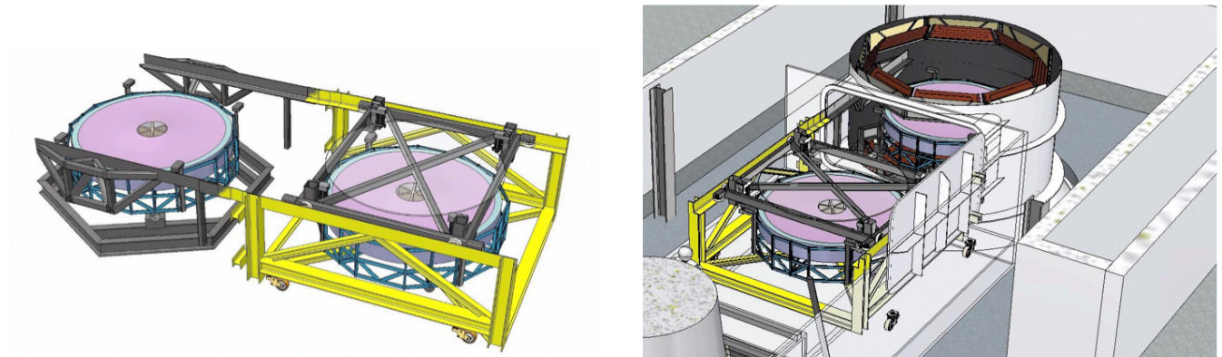
Figure 4-11 The MA trolley, with the HT component in Grey and the GT component in Yellow.
