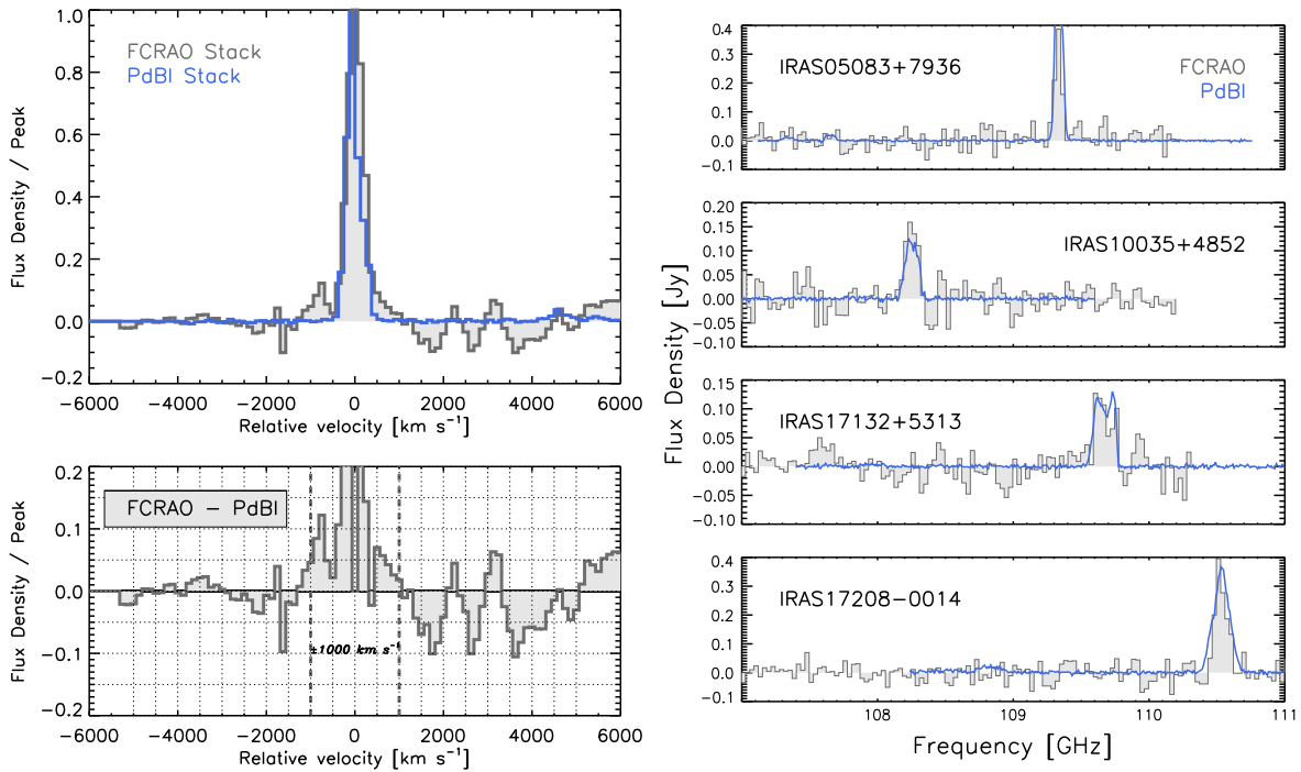
Figure 3. (left) Stacked spectra, normalized to the peak of each spectrum from our PdBI observations (blue) over stacked FCRAO spectra of the same four targets from C11 (gray) at 150 \text{ km s}^{-1} spectral resolution. As discussed in C11, the stacked FCRAO spectrum exhibits broad line wings at \sim 10\% of the peak flux density. This is evident even in the FCRAO stack of only our four targets. However, the PdBI spectra of the same galaxies, which have an order of magnitude better sensitivity, do not detect these wings or corresponding features in individual spectra (blue) despite a very good match of the observed (main) lines otherwise. The difference between the stacked spectra from FCRAO and the PdBI is shown in the bottom panel. This highlights the presence of a faint, broad component at \sim 10\% of the peak intensity in the FCRAO spectra but not the PdBI spectra. (right) Comparisons of individual spectra. The PdBI observations match the FCRAO results for the bright part of the line, but the faint line wings implied by the FCRAO stack are absent.
