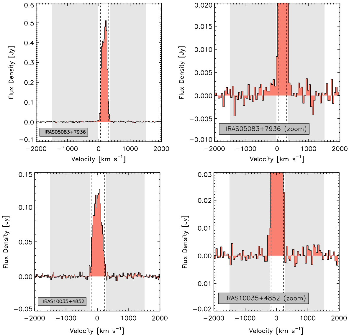
Figure 2. Spectra of our sources integrated over the regions of interest shown in Figure 1. Each spectrum is shown twice: first showing the full CO line (left, using 25 \text{ km s}^{-1} channels) and then zooming in to focus on faint emission near the level of the noise (right, using 50 \text{ km s}^{-1} channels). The gray region shows the part of the spectrum used to measure the flux in line wings. Dashed vertical lines show w_{20} , the width of the profile at 20% of its peak value. Table 2 reports integrated quantities for each spectrum.
