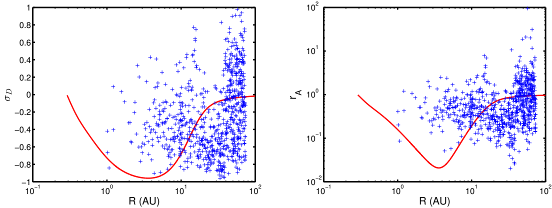
Figure 5. Left: Comparison between the theoretical and observed normalized residual energy as a function of heliocentric distance. Right: Comparison between the theoretical and observed fluctuating Alfvén ratio as a function of heliocentric distance. Solid curves are theoretical results and scatter plus symbols are observational results.
