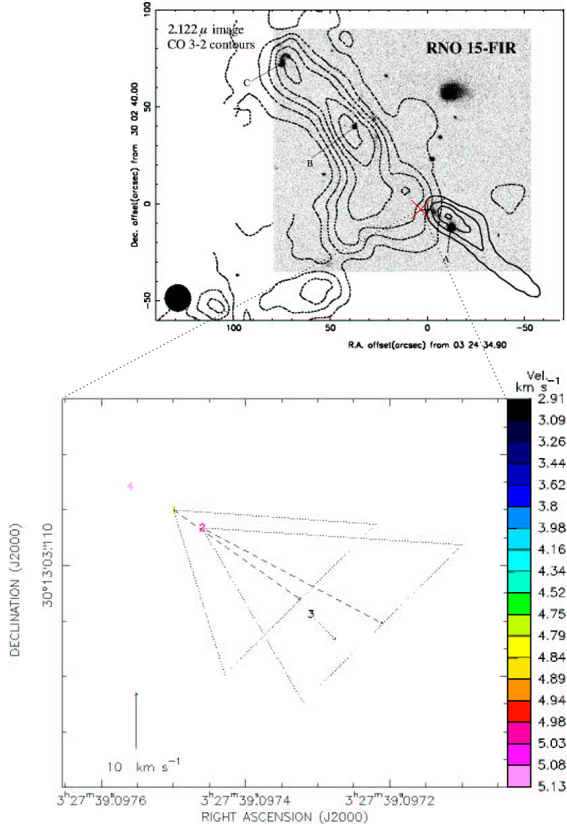
Fig. 3. VLBA results towards RNO 15-FIR. The top panel shows a H_2 2.12 \mu m image (gray scale) of the RNO 15-FIR outflow region (Davis et al. 1997b) with, overlaid, a contour map of the CO 3 \rightarrow 2 integrated intensity measured by Davis et al. (1997a) using the James Clerk Maxwell Telescope (JCMT). The blue-shifted flow lobe is reported with full lines, the red-shifted lobe with dashed lines. The three brightest, compact H_2 knots are denoted with the letters "A", "B" and "C". The black cross marks the IRAS position of RNO 15-FIR. The red cross gives the absolute position of the 22.2 GHz water masers as deduced with our phase-reference VLBA observations. The bottom panel shows the water maser map derived with two epochs of phase-reference VLBA observations. Feature positions and line of sight velocities are indicated with the same notation used for the water maser maps of the Serpens region (see caption of Fig. 1). The dashed arrows indicate the measured (absolute) proper motions. The dotted triangles drawn around the proper motion vectors represent the amplitude and orientation uncertainty. A dotted arrow is used for representing the proper motion of the feature with label number "3" to indicate that is at most uncertain, with \text{SNR} \leq 1 . The amplitude scale of the proper motions is given at the bottom left-hand corner of the panel. The plot axes give absolute, RA and DEC coordinates.
