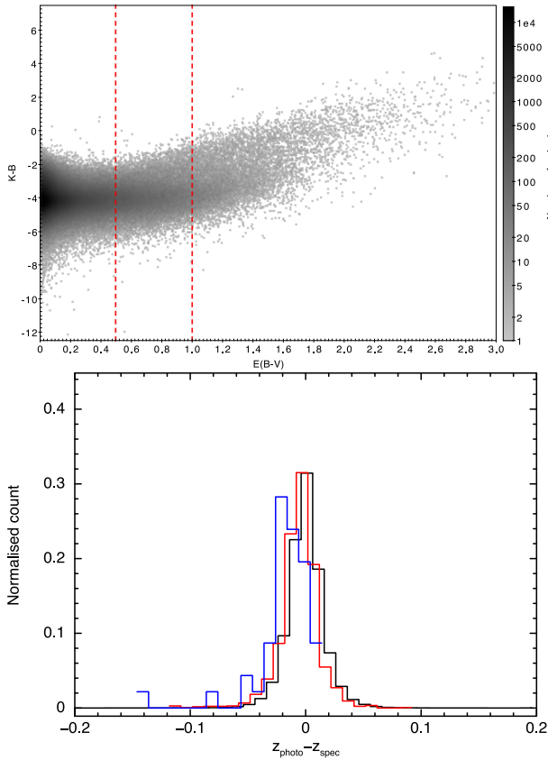
Figure 4. The effect of extinction on the colour and redshift accuracy of the 2MPZ v1.1 catalogue. Top: The extinction-corrected K - B colour as a function of extinction. For values of E(B - V) \geq 0.5 , a clear trend starts to emerge, indicating a selection effect due to reddening. The contours indicate the density of the points, and the red lines mark E(B - V) = 0.5 and 1. Bottom: histograms of z_{\text{photo}} - z_{\text{spec}} for objects with spectroscopic redshift measurements, for E(B - V) < 0.5 (black), 0.5 \leq E(B - V) < 1 (red) and E(B - V) \geq 1 (blue). The red histogram shows a small systematic shift, such that the mean photometric redshift is 0.004 too low compared to spectroscopic values; the widths are comparable. At high extinction, the photometric redshift calibration becomes very poor.
