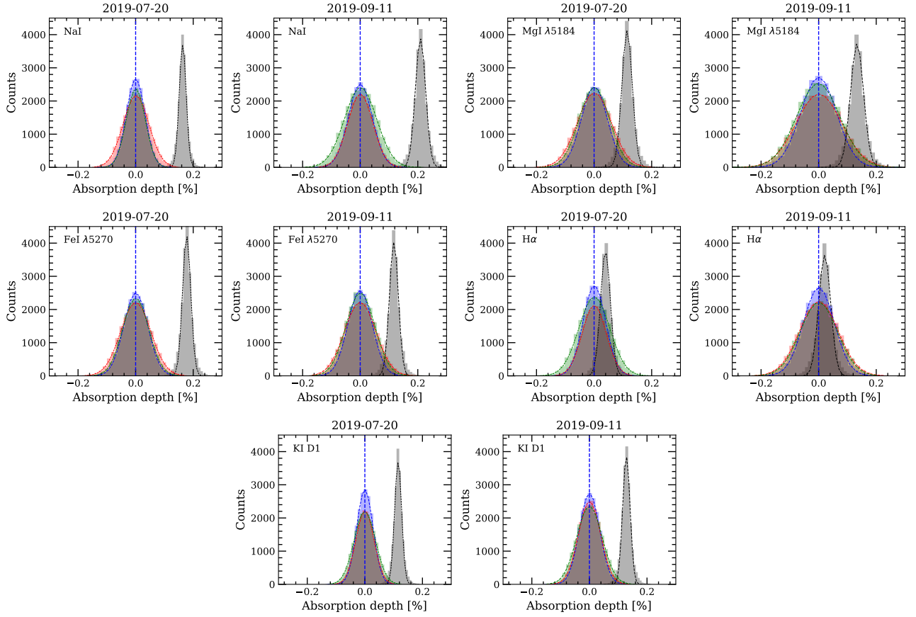
Fig. B.1. Distributions of the EMC analysis of each individual night for different spectral lines: Na I D1 and D2, Mg I \lambda 5184 , Fe I \lambda 5270 , H \alpha , and K I D1. The absorption depth calculations are performed using 0.4 \text{ \AA} bandwidth except for the H \alpha for which we use 0.5 \text{ \AA} . In green we present the ‘out-out’ scenario, in red the ‘in-in’, in blue the ‘mix-mix’, and in grey the ‘in-out’. The blue dashed vertical lines show the zero absorption level. In coloured dashed lines, we show the Gaussian fit to the histograms.
