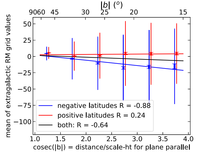
Figure 11. Extragalactic RM grid, sampled at the same points that are used for Figures 8 and 9, data from Oppermann et al. (2015). The gradual separation of the red and blue points at lower latitudes, similar to that seen in the left panel of Figure 8, suggests that the north Galactic hemisphere has a net line-of-sight B -field component pointing toward the Sun, while the southern hemisphere has a net B -field component pointing away from the Sun. The leftmost points are at 4.52 \pm 0.19 \text{ rad m}^{-2} in blue (negative latitudes) and 5.45 \pm 0.16 \text{ rad m}^{-2} in red (positive latitudes), a 5\sigma difference.
